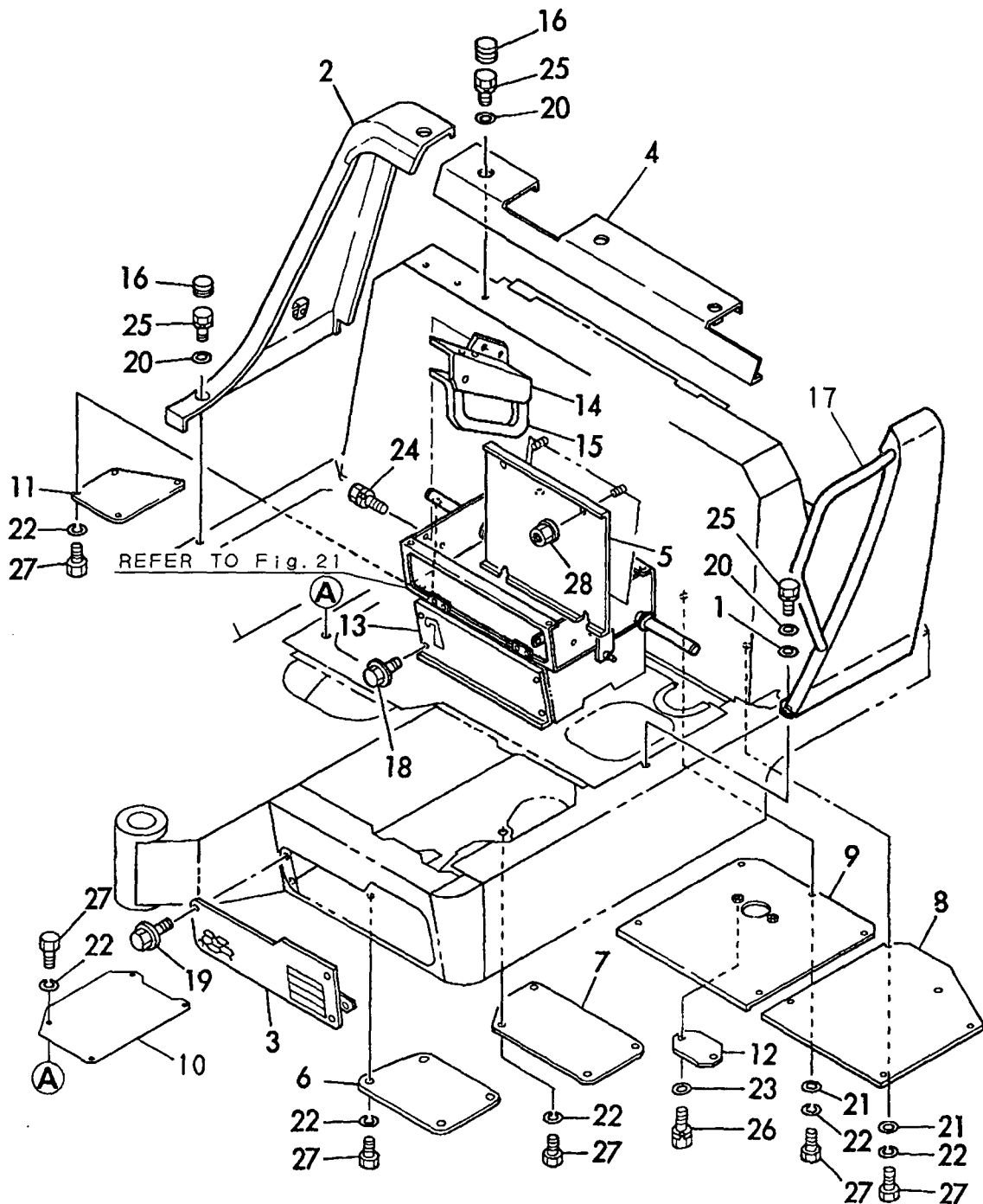
Fig. 19 FRAME COVER https://truckmanualshub.com/
