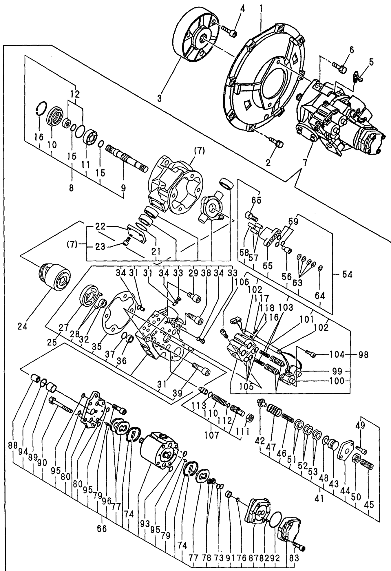
Fig. 24 HYD. OIL PUMP & JOINT https://truckmanualshub.com/
