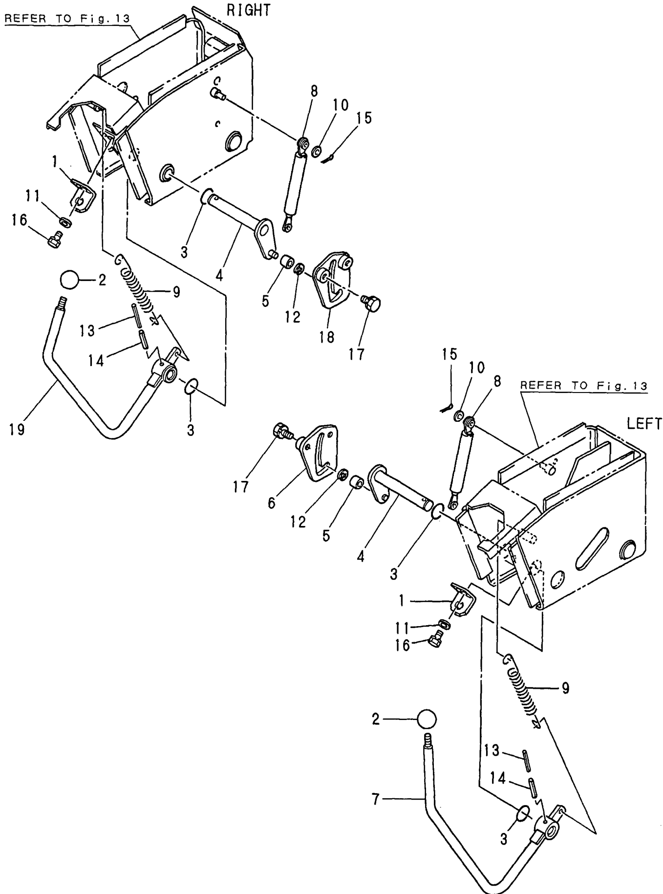
Fig. 17 CONTROL EQUIPMENT (CUT OFF LEVER)
