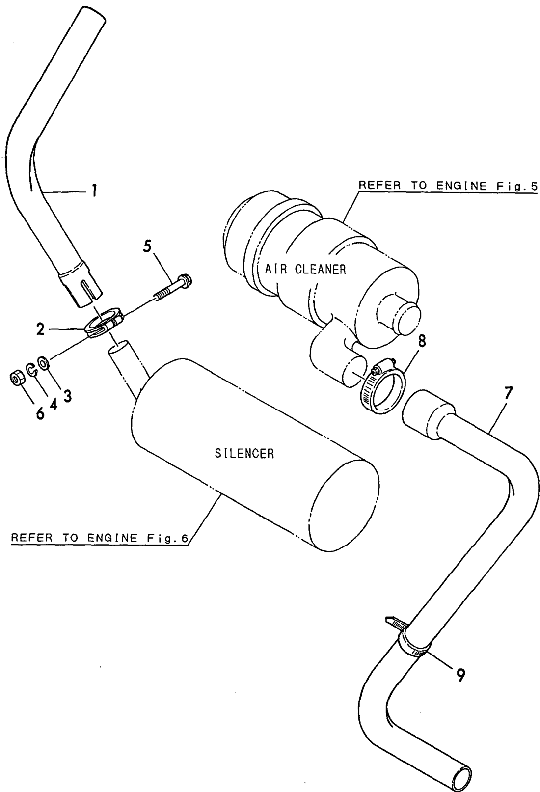
Fig. 3 INLET HOSE & EXHAUST PIPE https://truckmanualshub.com/
