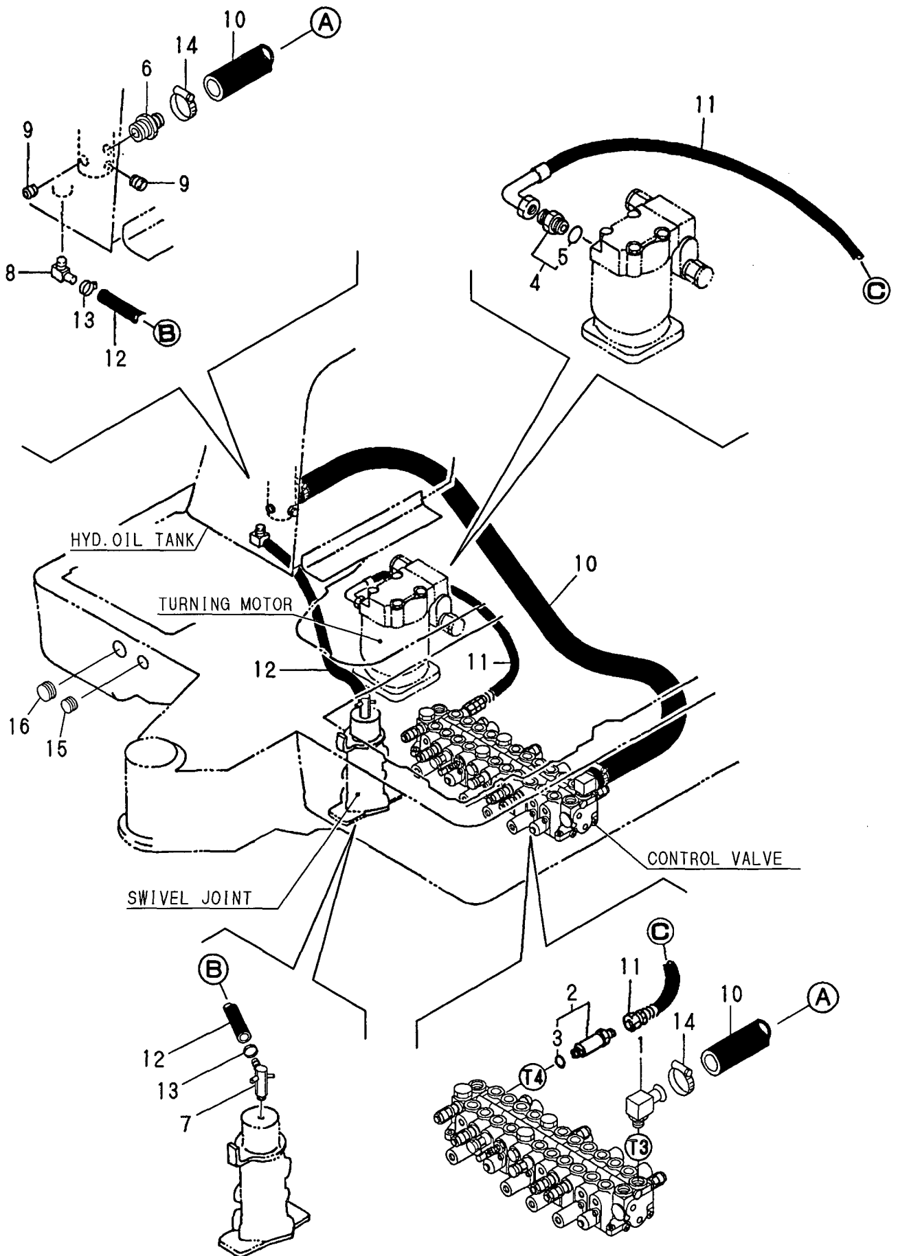
Fig. 43 HYD. OIL PIPING (RETURN) https://truckmanualshub.com/
