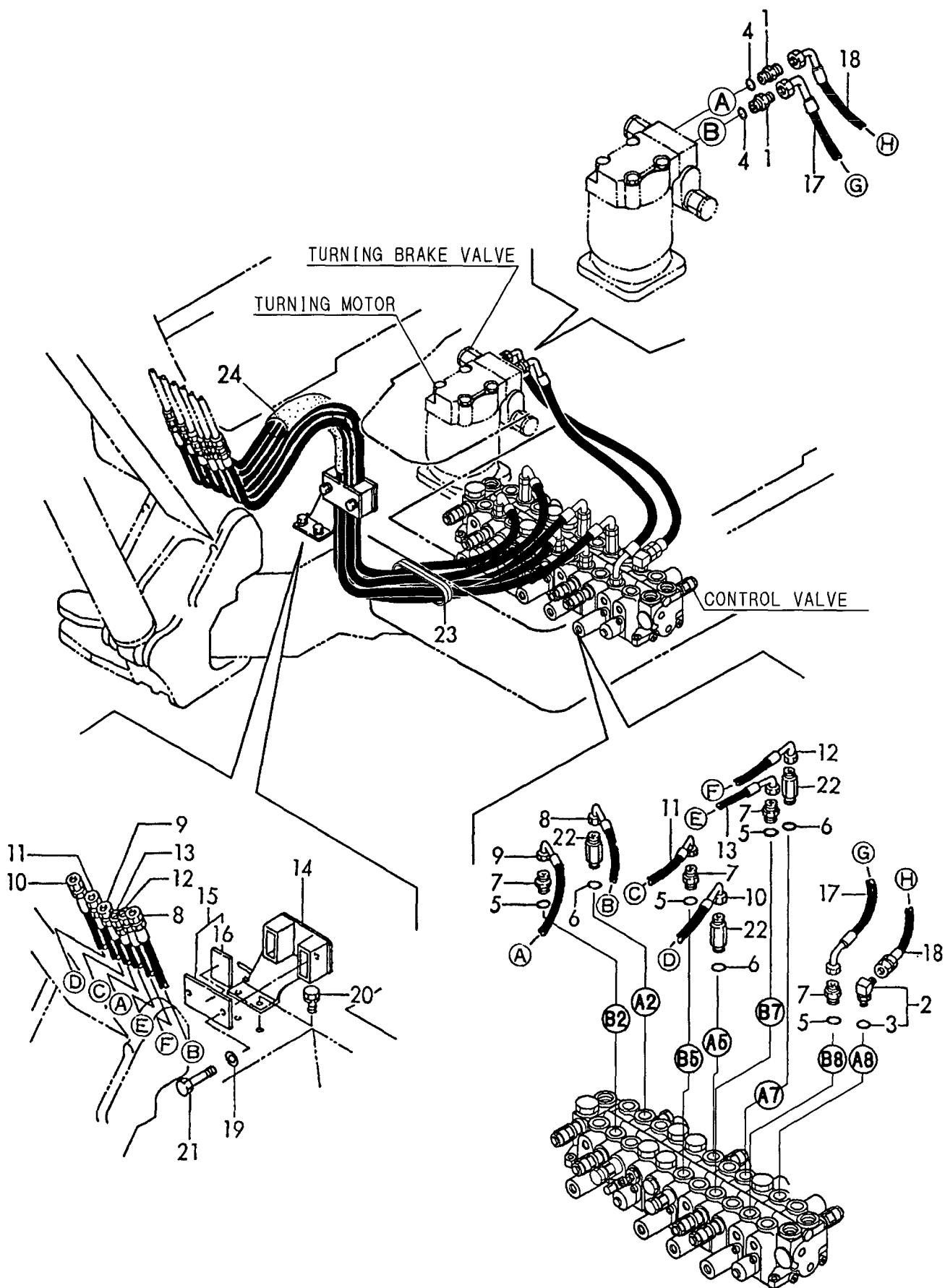
Fig. 41 HYD. OIL PIPING (VALVE~MOTOR~BOOM) https://truckmanualshub.com/
