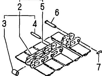
1 CRAWLER (350, TRAIANGLE)
