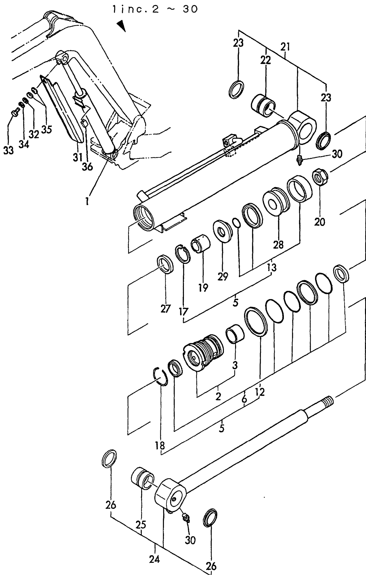
Fig. 25 BOOM CYLINDER https://truckmanualshub.com/
