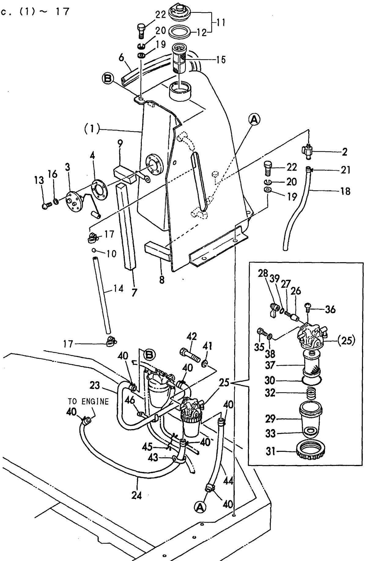
Fig. 7 FUEL TANK & FUEL PIPE https://truckmanualshub.com/
