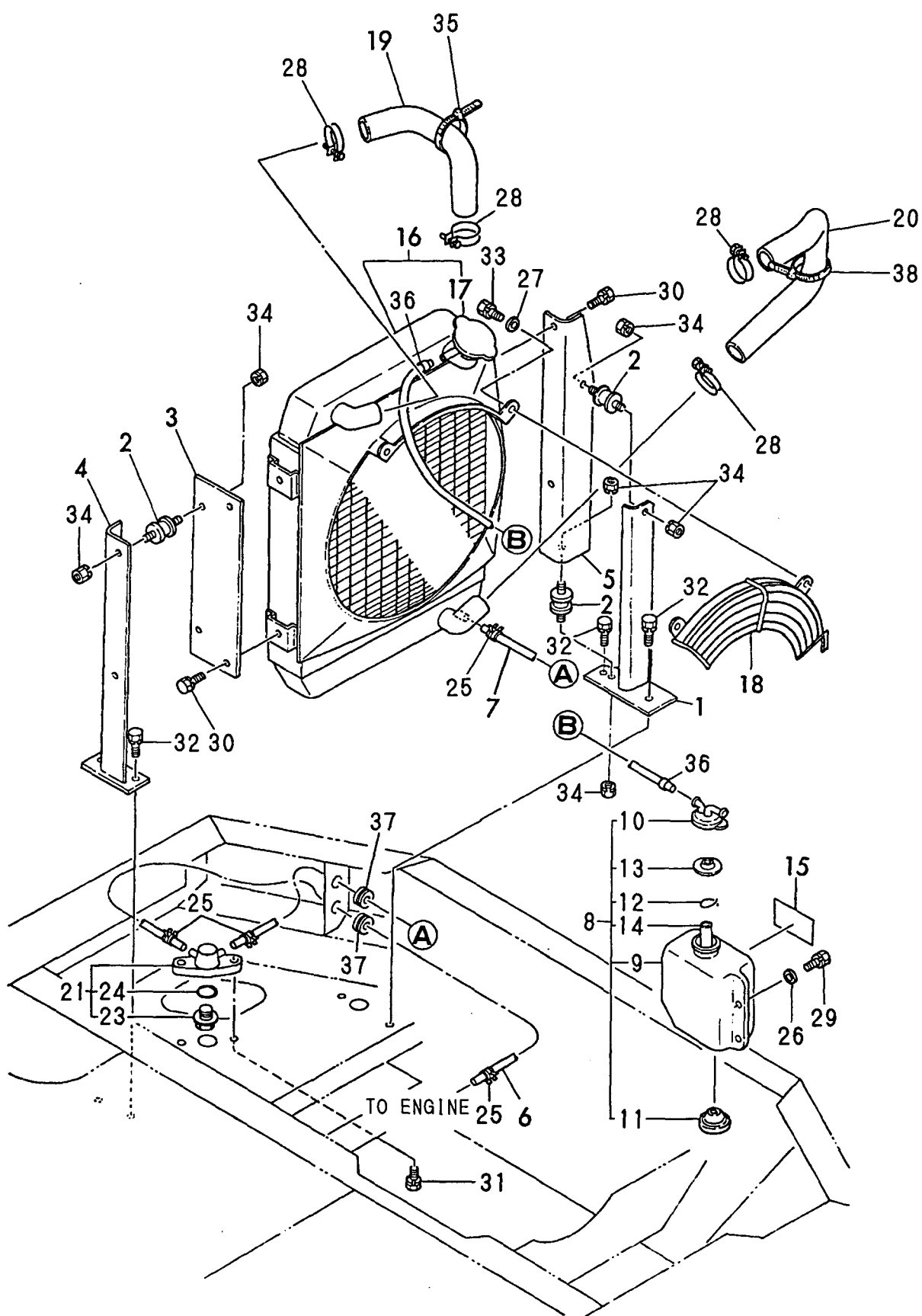
Fig. 6 RADIATOR & MOUNT https://truckmanualshub.com/
