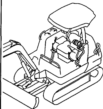
Fig. 3 INLET HOSE & EXHAUST PIPE
