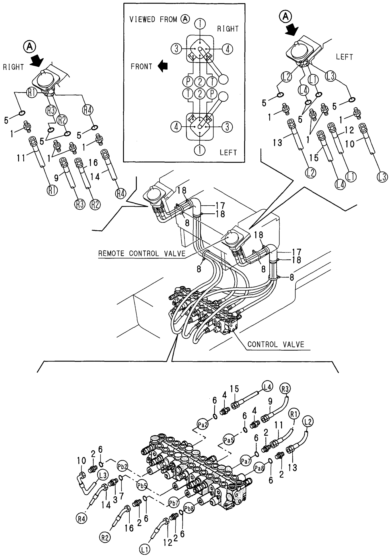
Fig. 47 CONTROL PIPING (REMO.-CON. V.~CONTROL V.)
