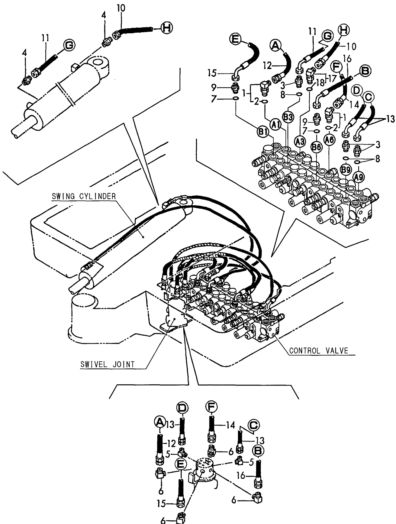
Fig. 42 https://truckmanualshub.com/ HYD. OIL PIPING (VALVE~SWIVEL~SWING)
