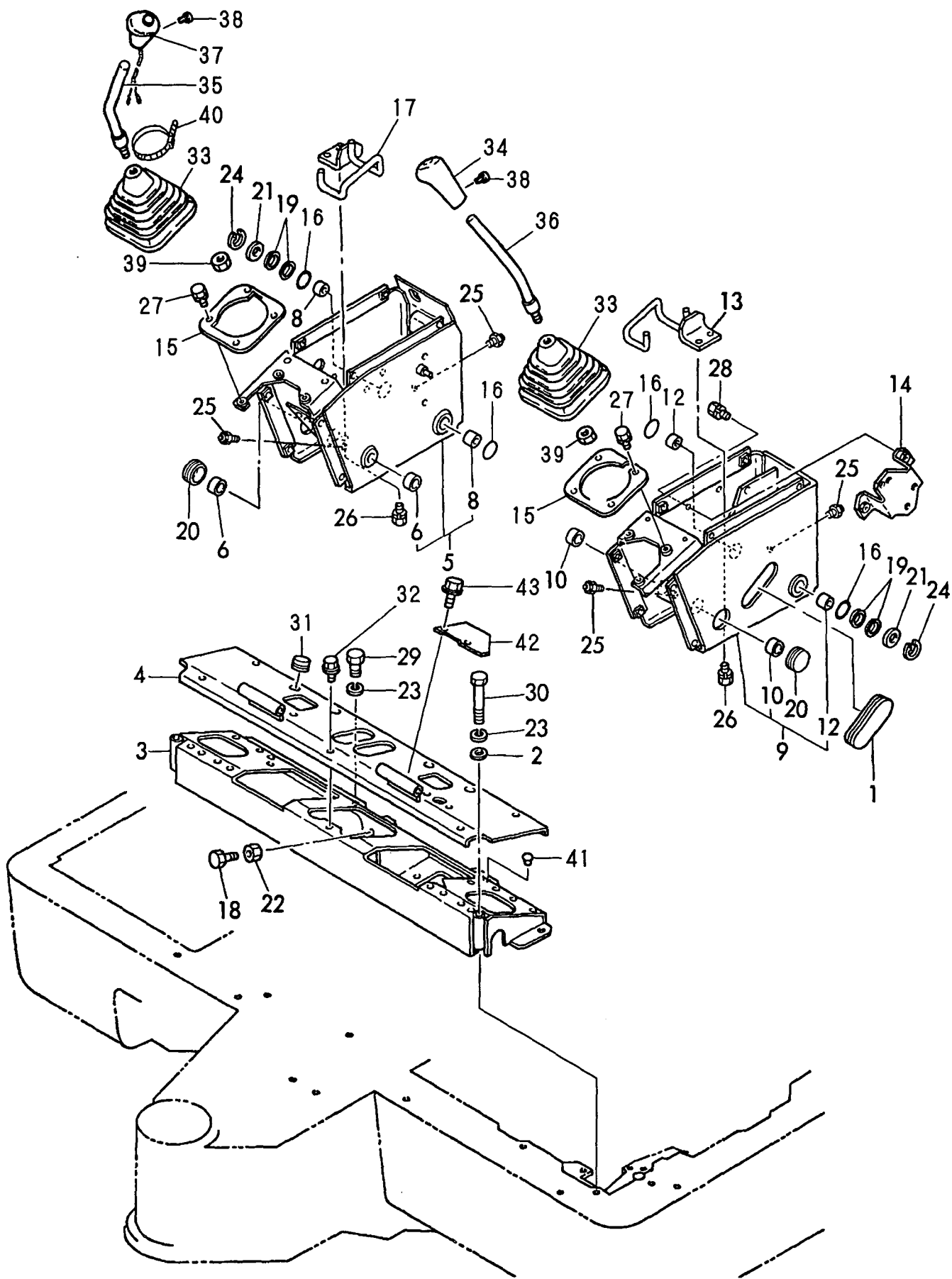
Fig. 13 CONTROL EQUIPMENT (LEVER STAND & OPERATION LEVER)
