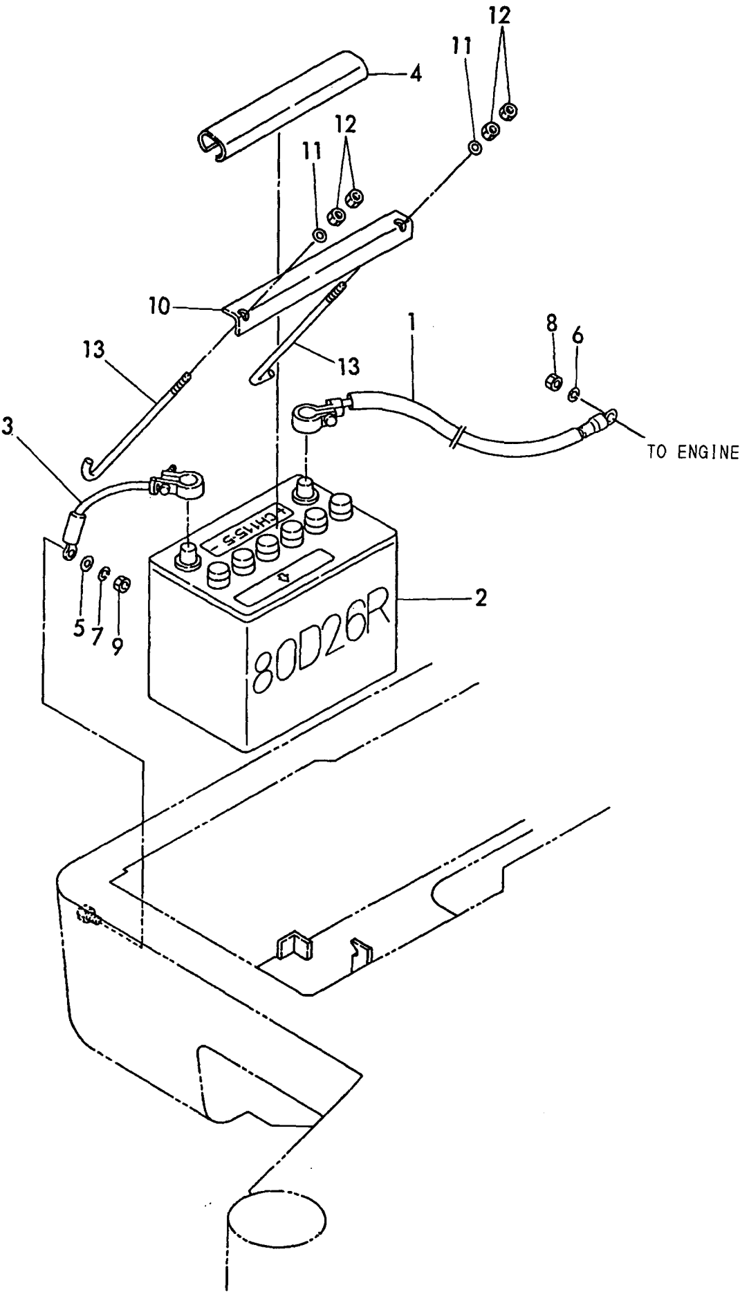
Fig. 8 BATTERY
