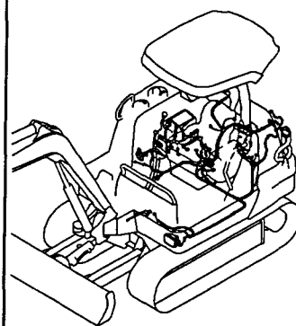
Fig. 10 WORK LAMP
