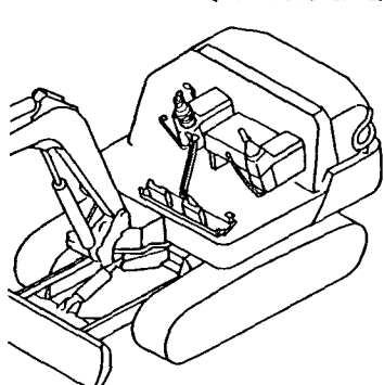
Fig.71 リモコンバルブ(右:AS仕様) REMOTE CONTROL VALVE (RIGHT:AS SPEC.)
