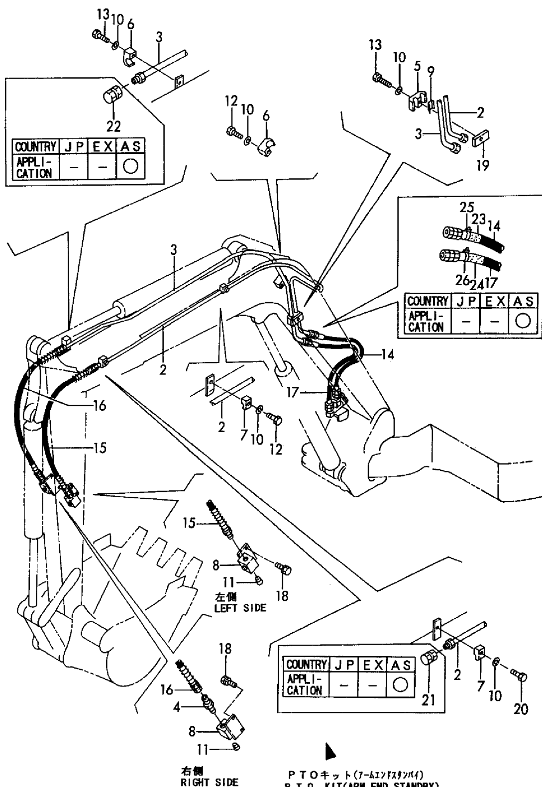
Fig. 85 油圧配管(PTO7 th -M:7 th -M:7 th -M:7 th 仕様)(新形) HYD. OIL PIPING(P. T. O. BOOM:ARM END SPEC. )(NEW)
