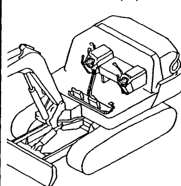
Fig.69 リモコンバルブ(JP, EX仕様) REMOTE CONTROL VALVE (JP, EX SPEC.)
