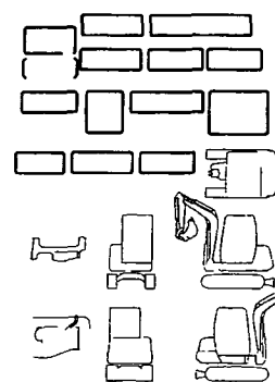
Fig 10 安全銘板(キャビン) (AS, EX) SAFETY LABEL (CANOPY) (AS, EX)
