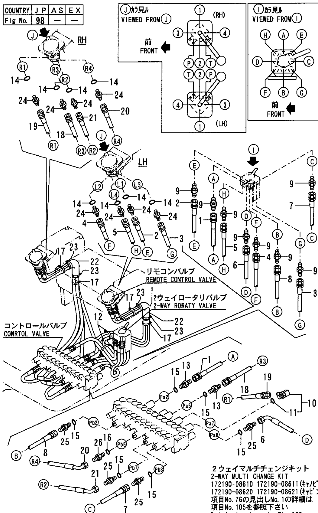
Fig. 98 CONTROL PIPING (MULTI CHANGE: 2-WAY, SIDE LEVER)
