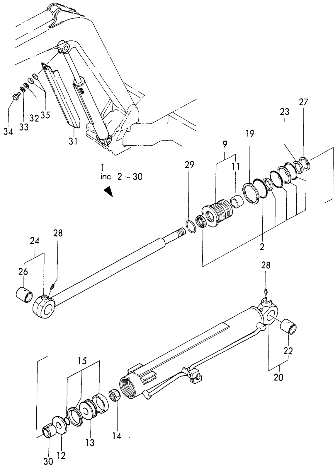
Fig. 35 ブームシリンダ(UA)(キャビン) https://trucks.machinery.com BOOM CYLINDER (UA) (CABIN SPEC.)
