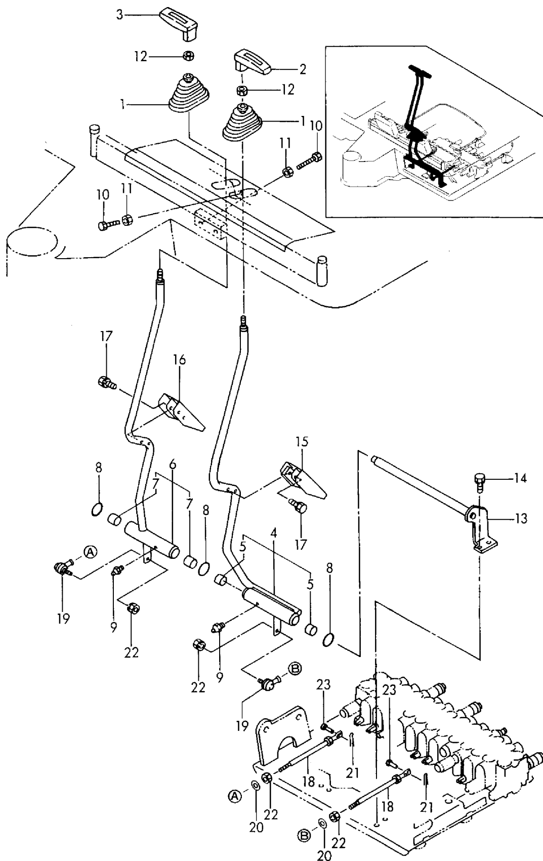
Fig. 25 操縦装置(走行) CONTROL EQUIPMENT(DRIVE)
