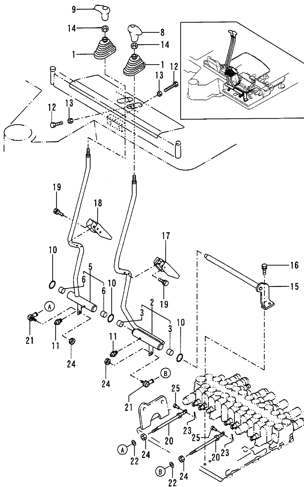
Fig. 35 操縦装置(走行) http://www.manualshub.com/ CONTROL EQUIPMENT (DRIVE)
