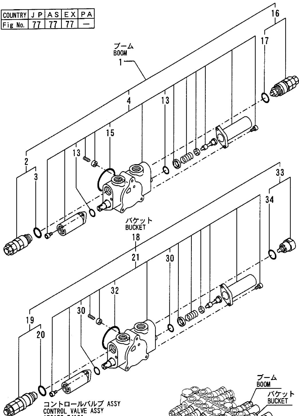
Fig. 77 77 CONTROL VALVE (BOOM & BUCKET: P. T. O. SPEC.)
