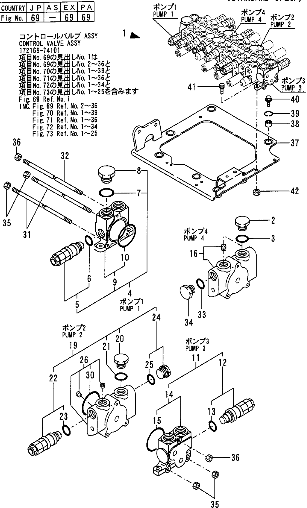
Fig. 69 CONTROL VALVE (P PORT & VALVE STAND : STANDARD SPEC.)
