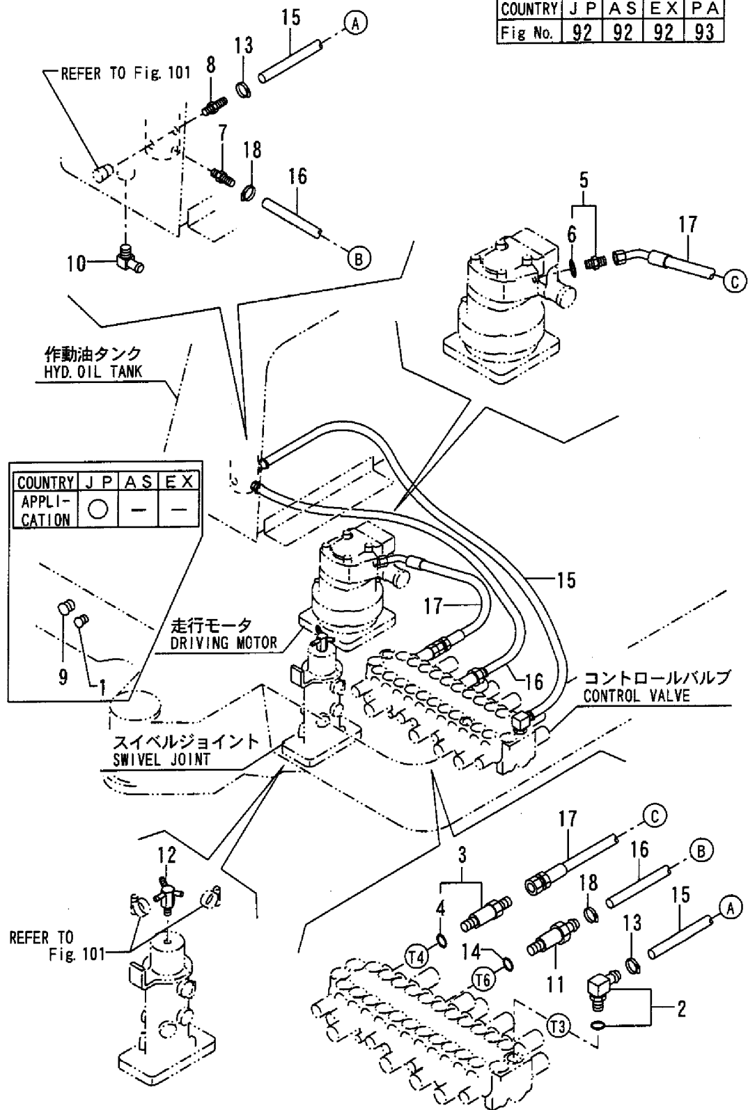
Fig. 92 油圧配管(帰管) HYD. OIL PIPING (RETURN)
