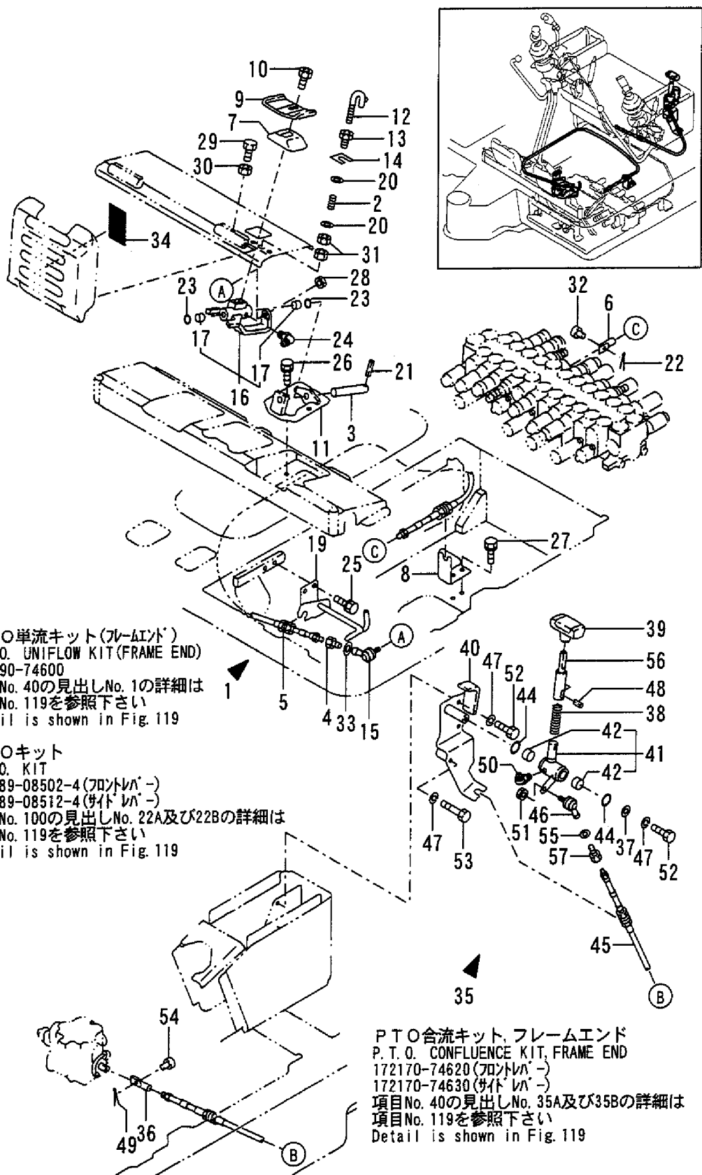
Fig. 40 操縦装置 (P.T.O. CONTROL) CONTROL EQUIPMENT (P. T. O. CONTROL)
