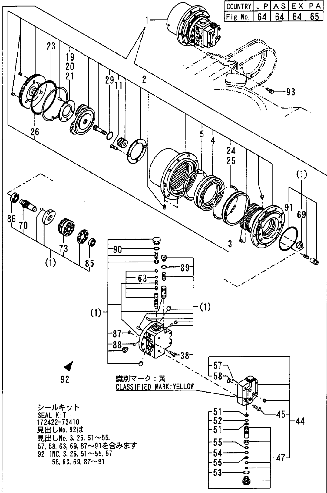
Fig. 65 走行モータ(PA) http://www.truckmanualshub.com/ DRIVING MOTOR (PA)
