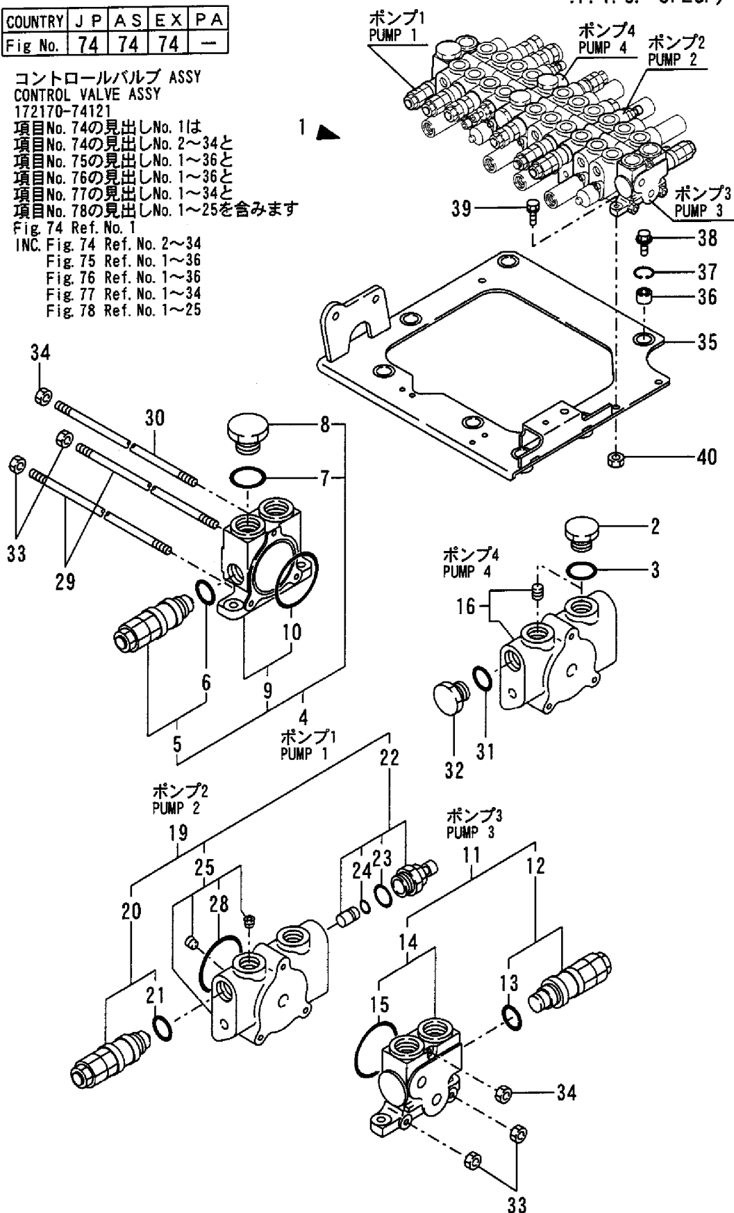
Fig. 74 CONTROL VALVE (P PORT & VALVE STAND : P. T. O. SPEC.)
