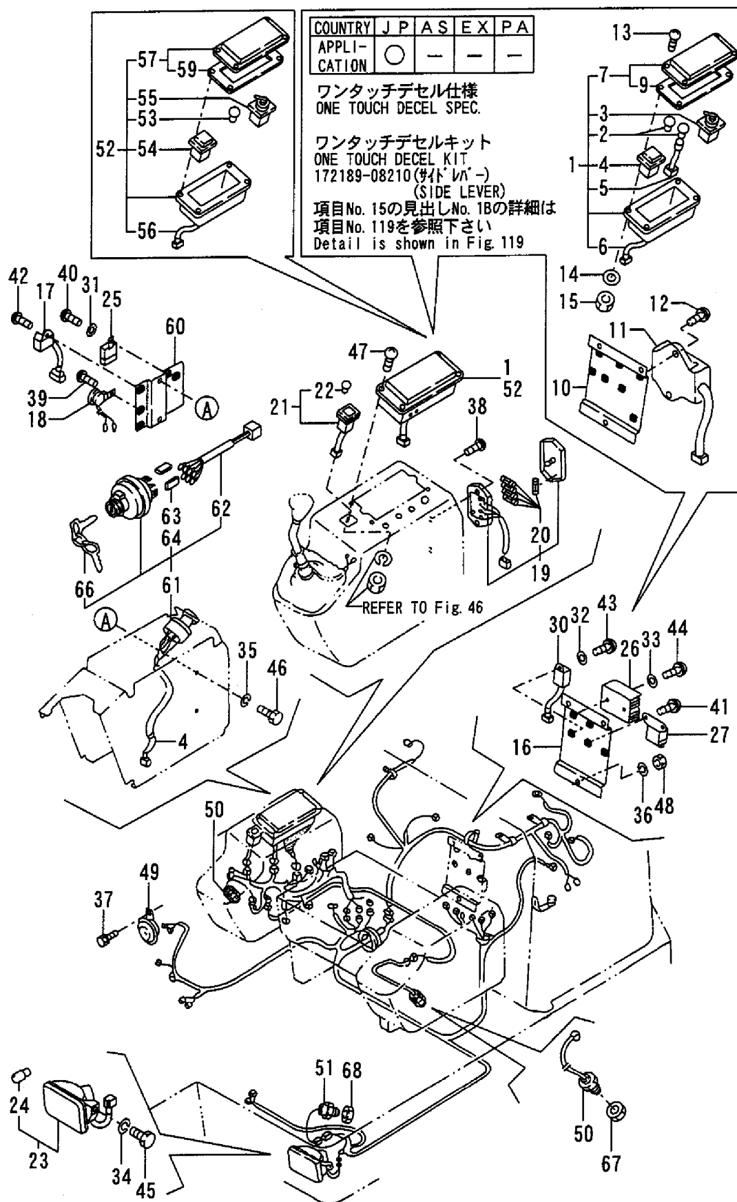
Fig. 24 電装品(機器:サイドレバ) ps:manuals.kob.com/ ELECTRIC PART (EQUIPMENT: SIDE LEVER)
