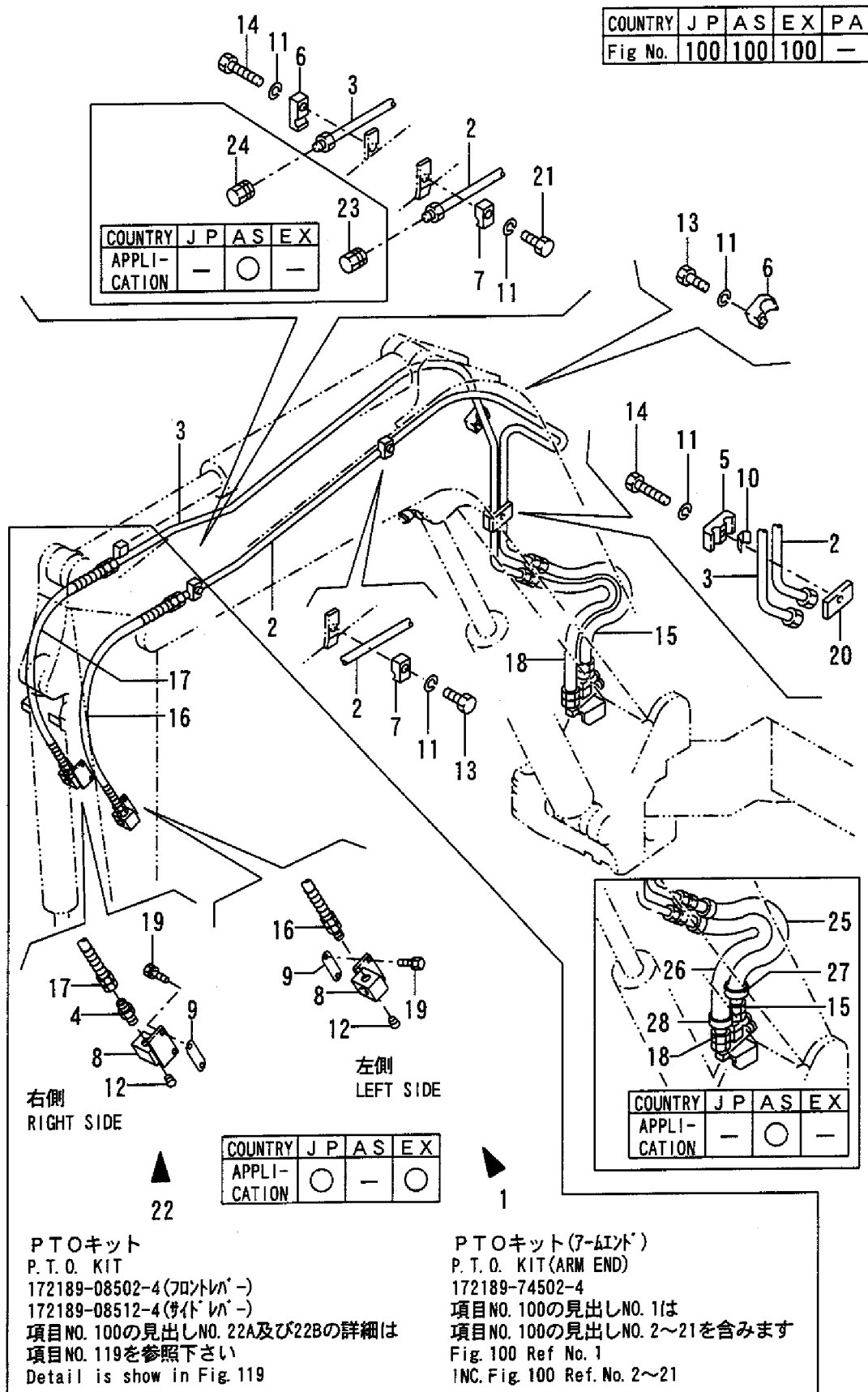
Fig. 100 油圧配管 (P.T.O. 7-11ト) / HYD. OIL PIPING (P. T. O. ARM END)
