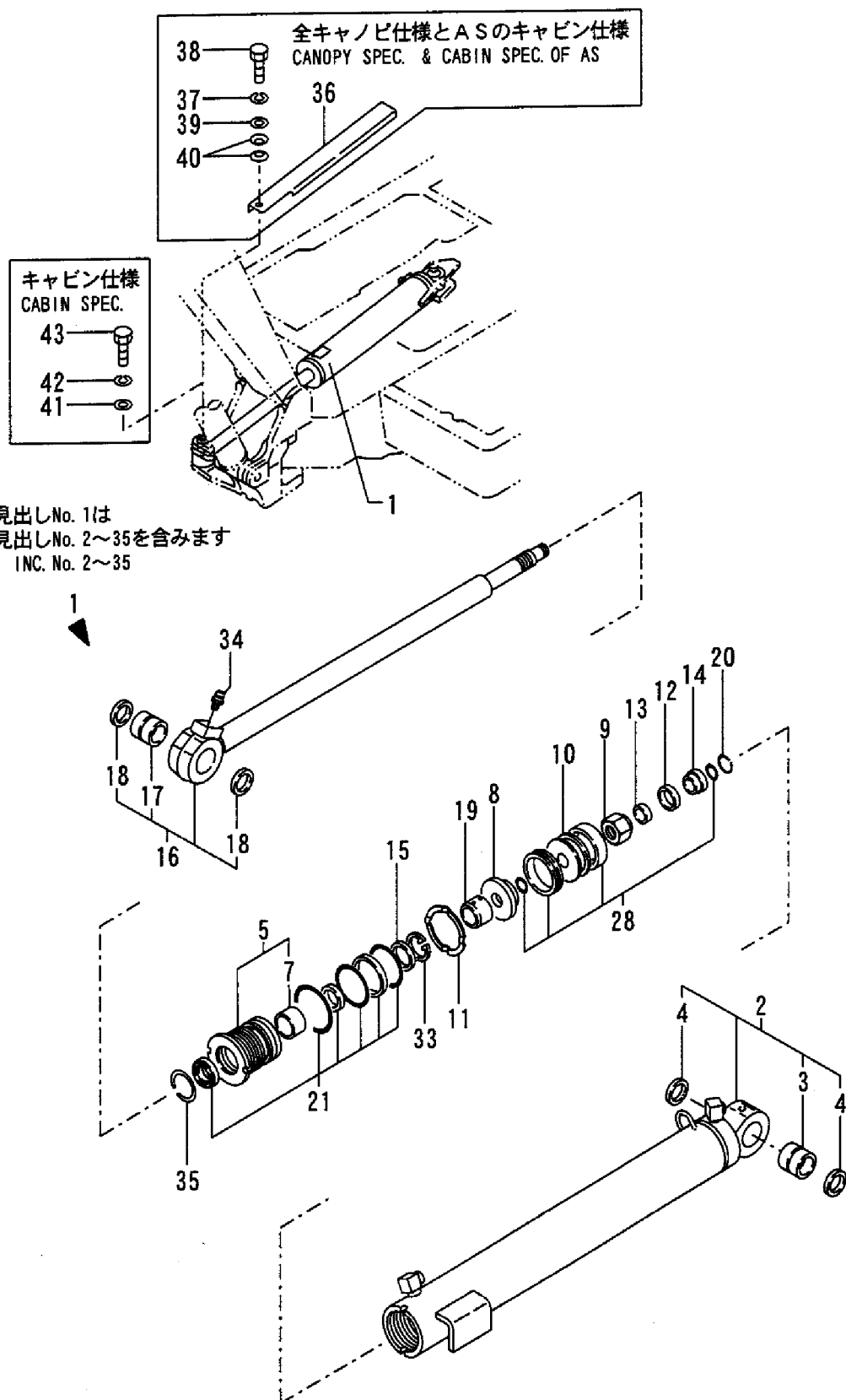
Fig. 62 SWING CYLINDER
