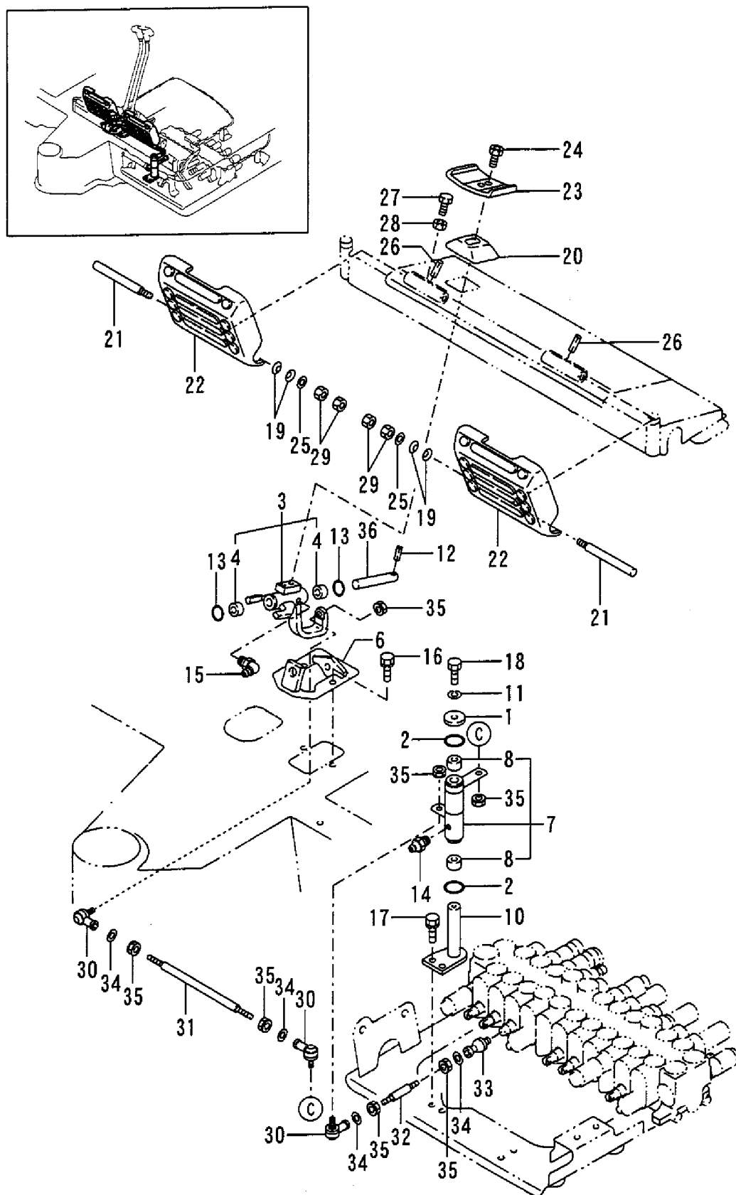
Fig. 36 操縦装置 ( Swing ) CONTROL EQUIPMENT (SWING)
