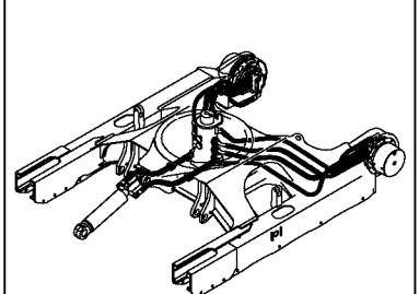
Fig. 46 HYD. OIL PIPING (TRAVEL)
