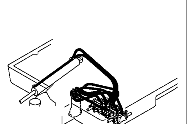
Fig. 42 HYD. OIL PIPING (VALVE ~ SWIVEL, SWING)
