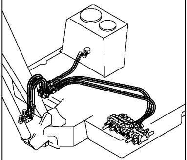
Fig. 46 HYD. OIL PIPING (TRAVEL)
