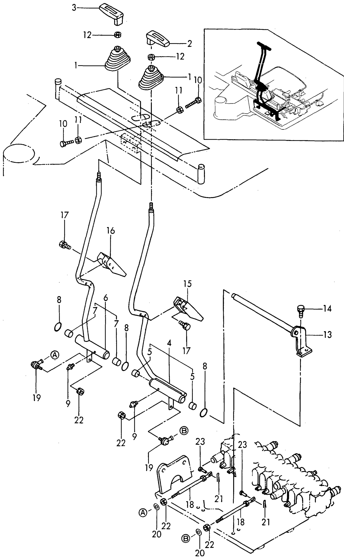
Fig. 17 操縦装置(走行) https://truckmanualshub.com/ CONTROL EQUIPMENT(DRIVE)
