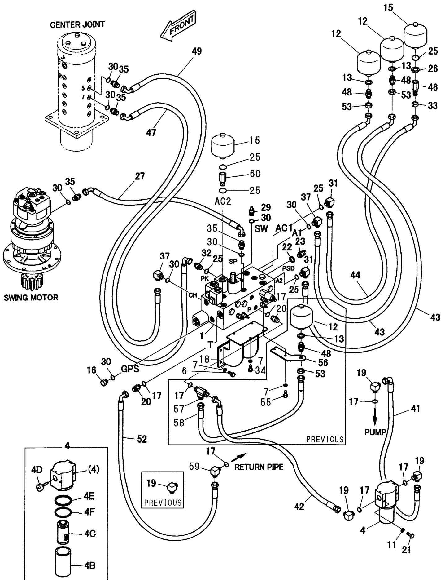
Fig. 119 BRAKE PIPING (2)
