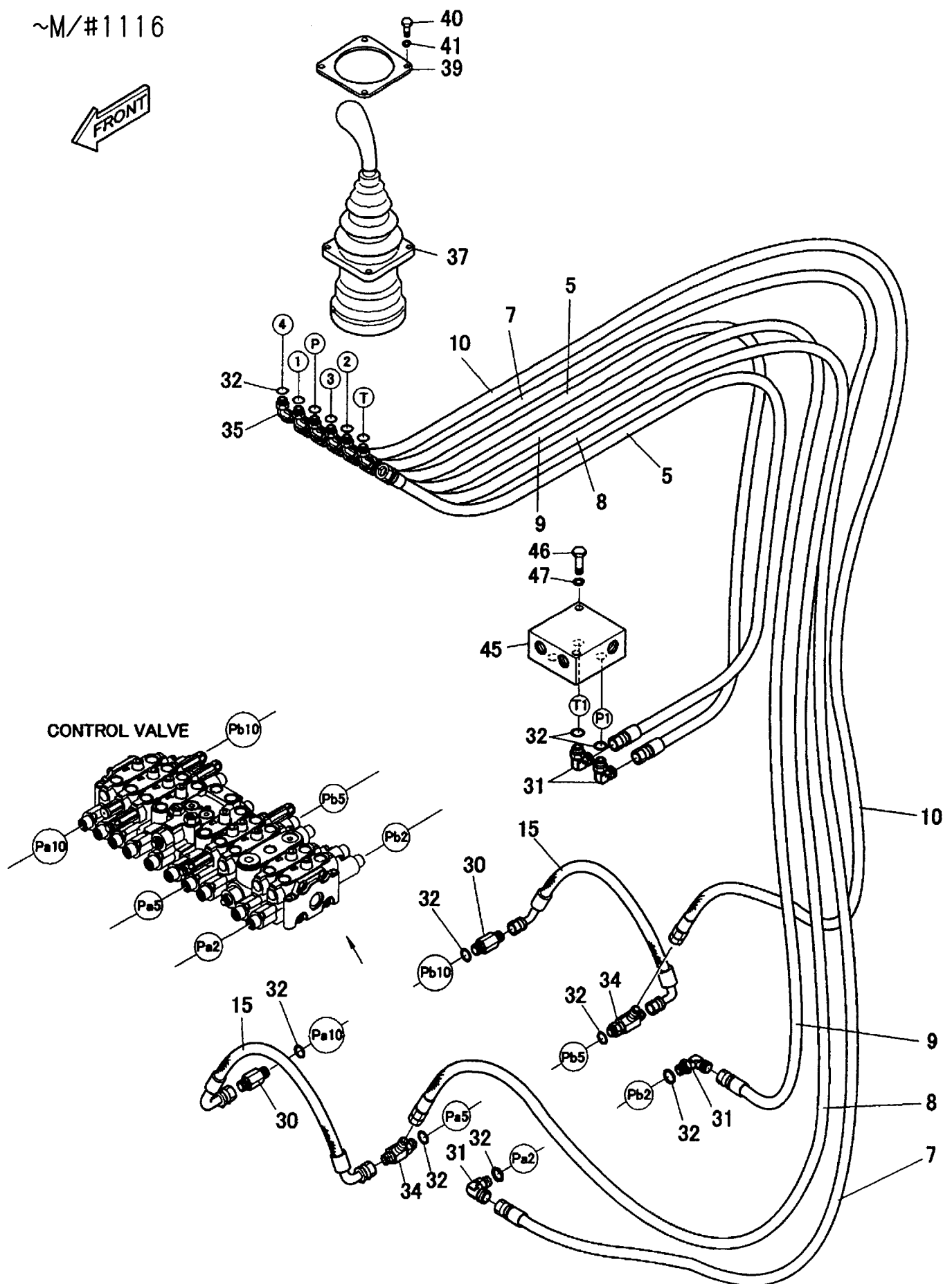
Fig. 114 PILOT PIPING (1) (PREVIOUS)
