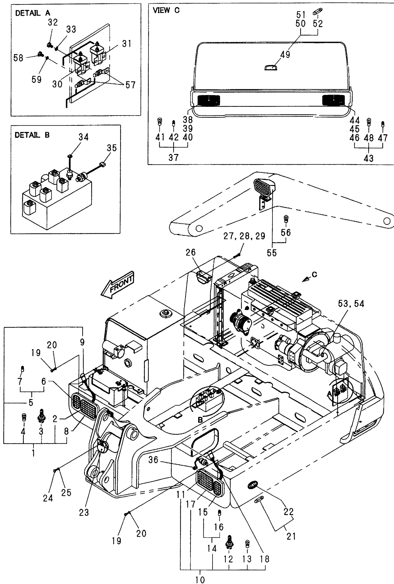
Fig. 46 ELECTRIC PARTS (8) -RELATED PART
