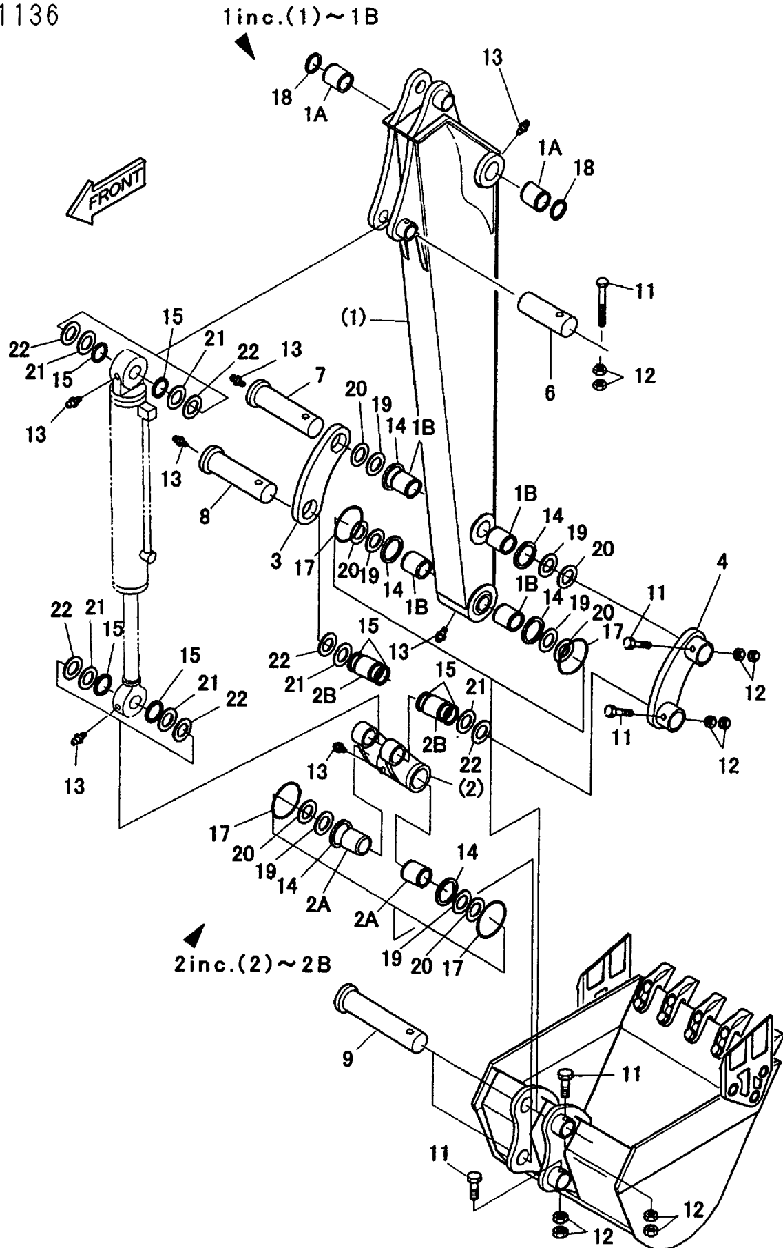
Fig. 132 ARM-1. 6M (PREVIOUS)
