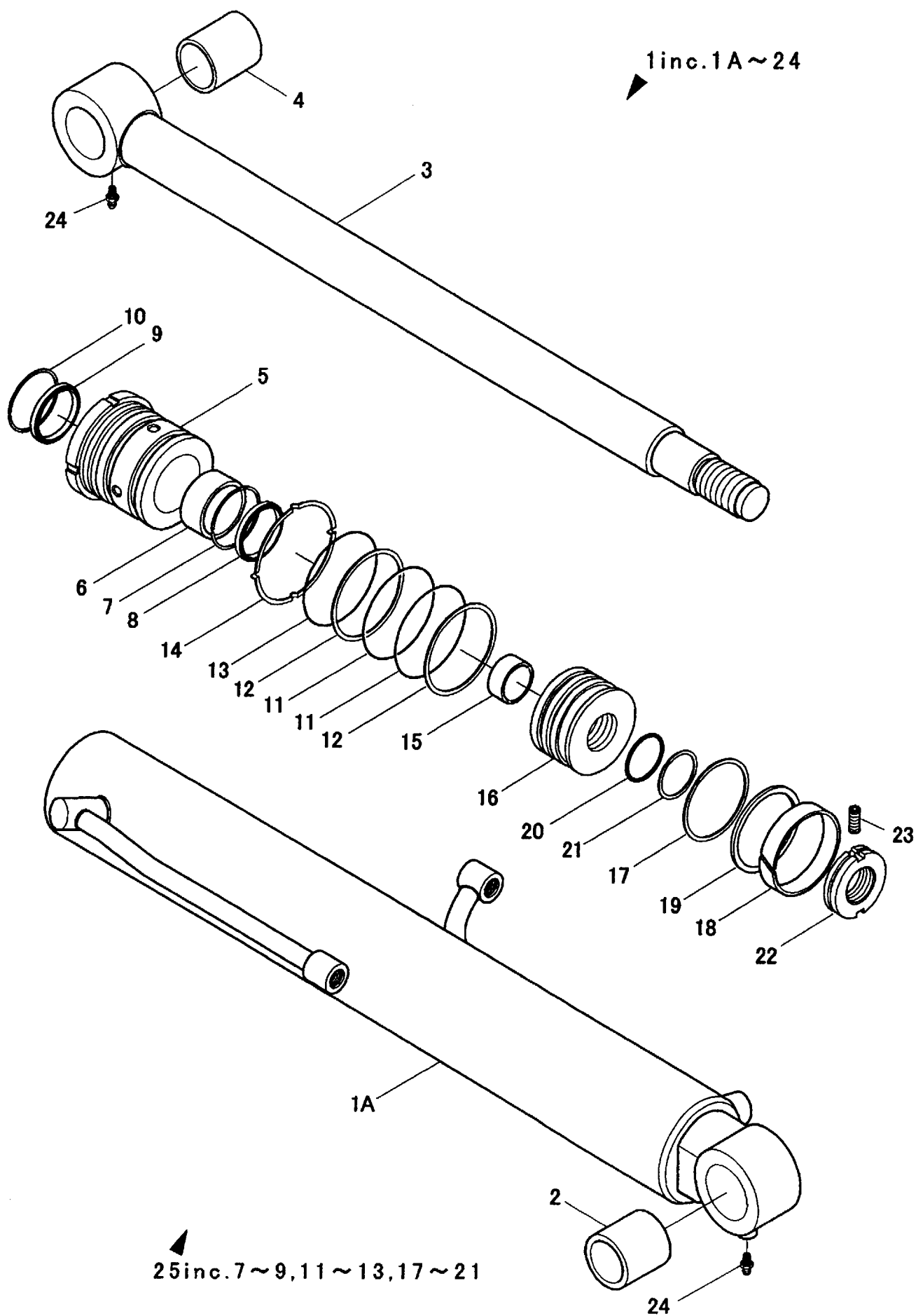
Fig. 91 BOOM CYLINDER
