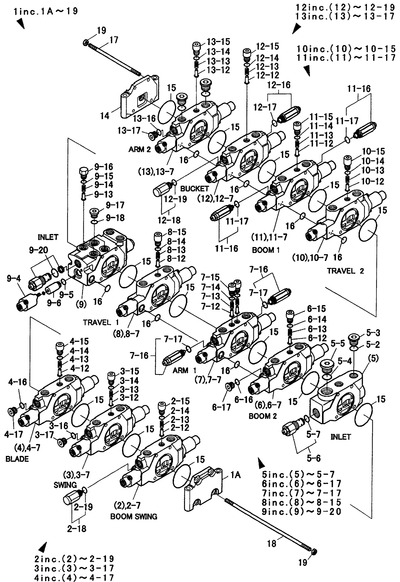
Fig. 83 CONTROL VALVE-BOOM SWING
