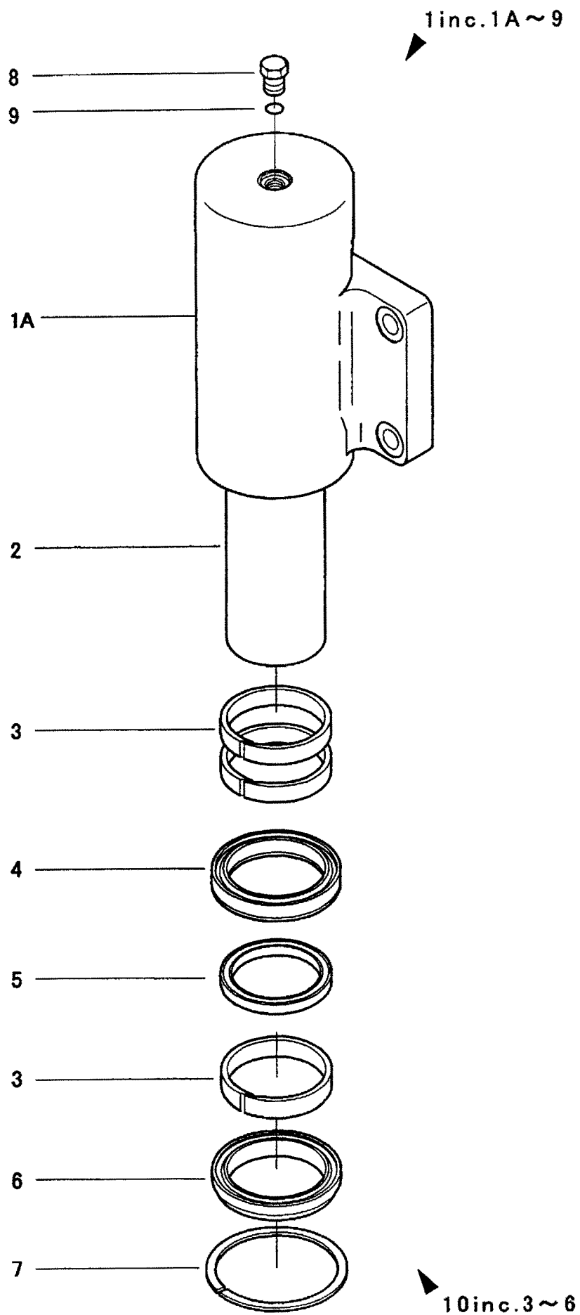
Fig. 96 CHOCKING CYLINDER
