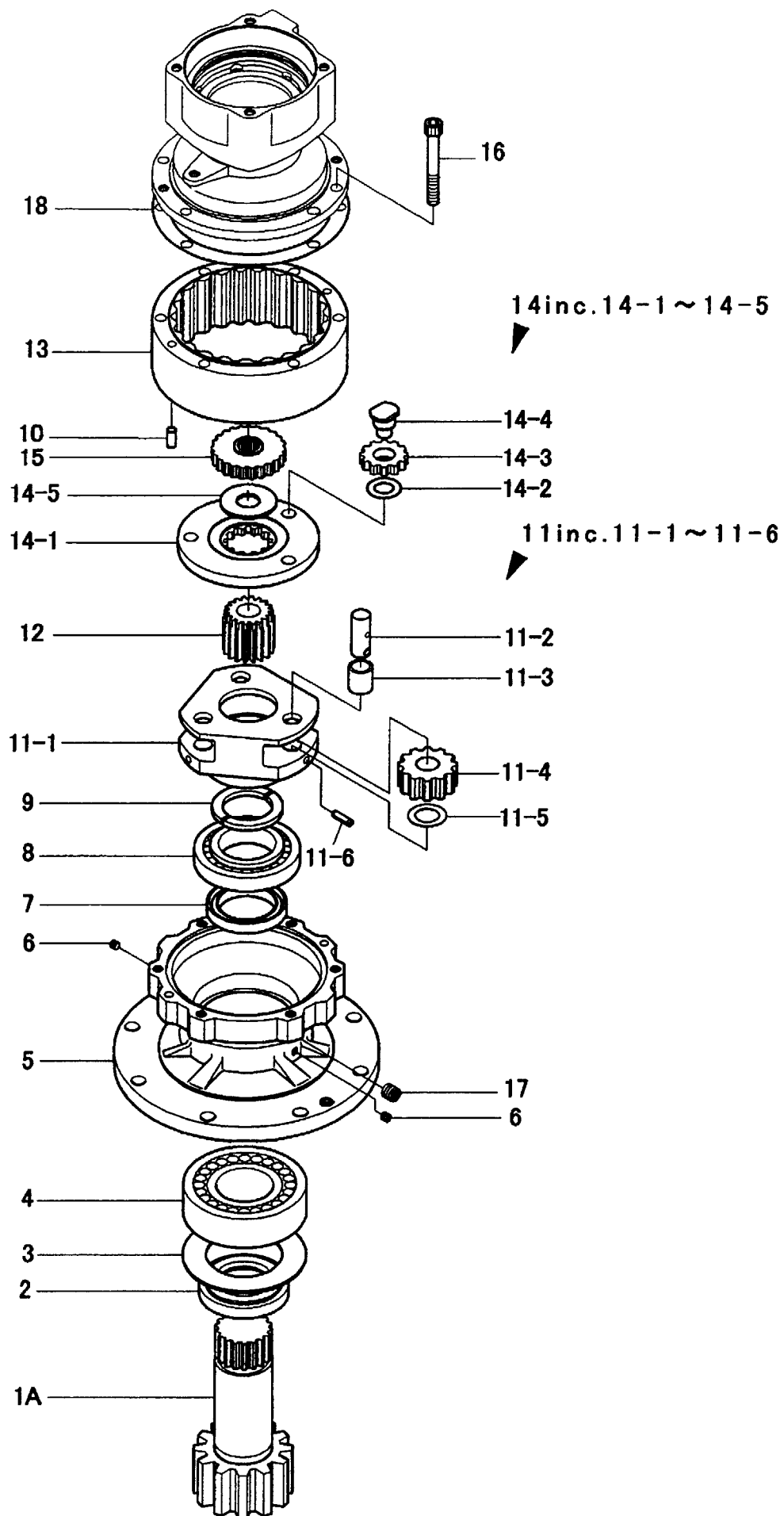
Fig. 76 REDUCTION GEAR
