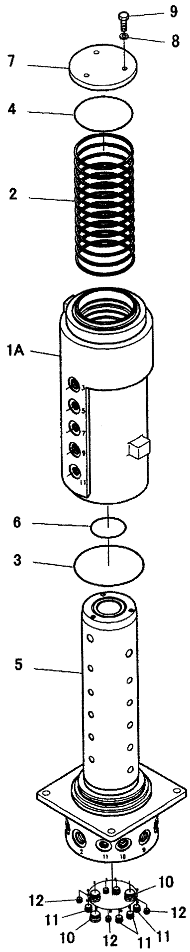
Fig. 97 CENTER JOINT
