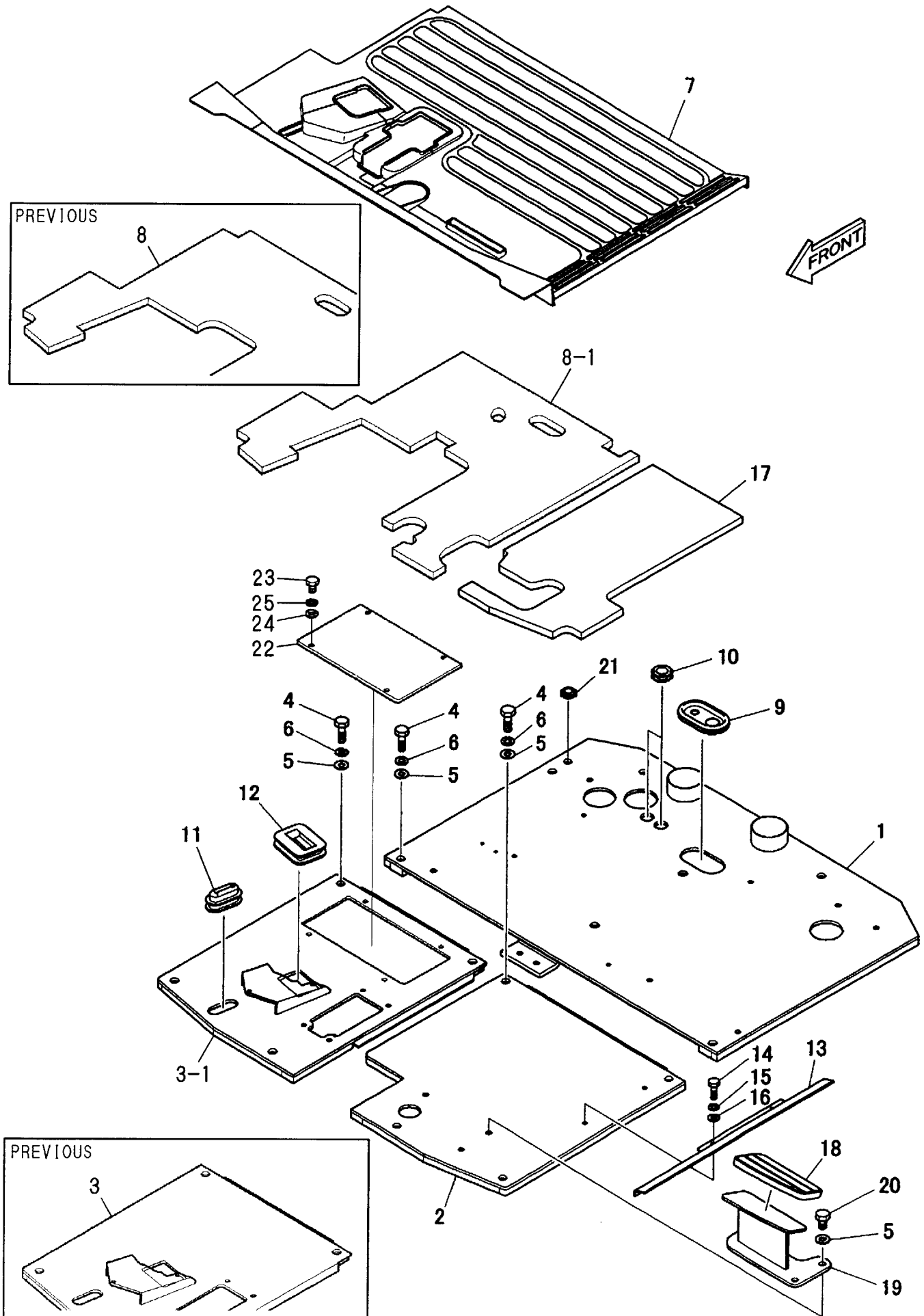
Fig. 38 FLOOR PLATE
