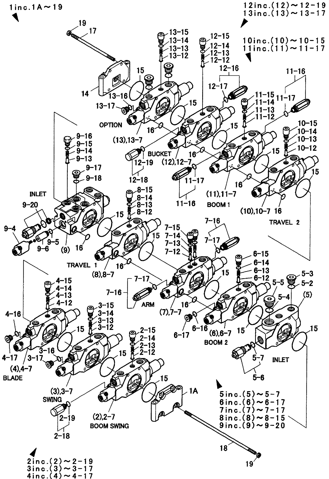
Fig. 84 CONTROL VALVE-BOOM SWING (2-WAY SPEC.)
