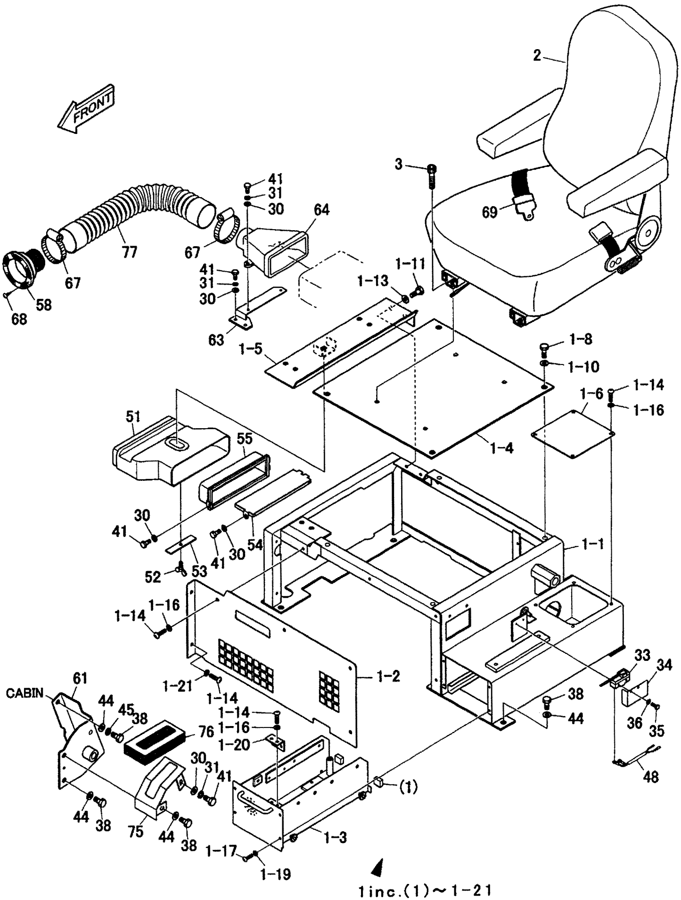
Fig. 29 ELECTRIC BOX-STAND
