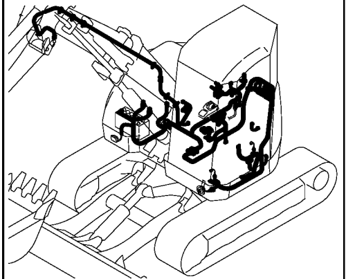
Fig. 12 ELECTRIC PART (WIRING)
