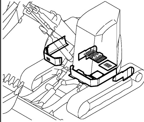
Fig. 29 COVER (FRAME)
