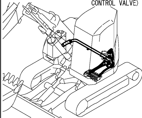
Fig. 59 HYD. OIL PIPING (TANK~PUMP~ CONTROL VALVE)
