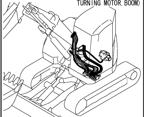
Fig. 60 HYD. OIL PIPING (PUMP, CONTROL V. ~ TURNING MOTOR, BOOM)
