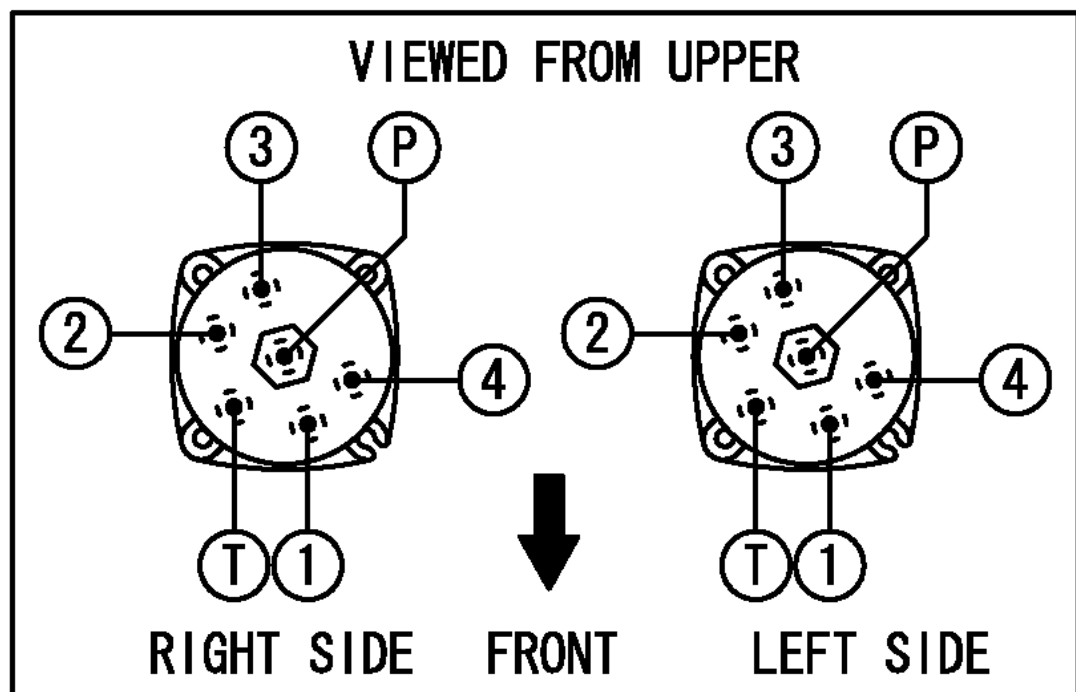
REMOTE CONTROL VALVE
