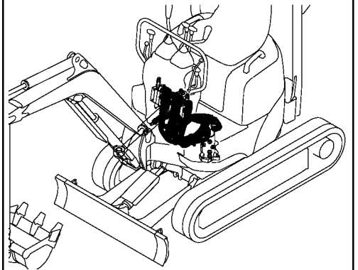
Fig. 48 HYD. OIL PIPING (VALVE-SWIVEL, SWING)
