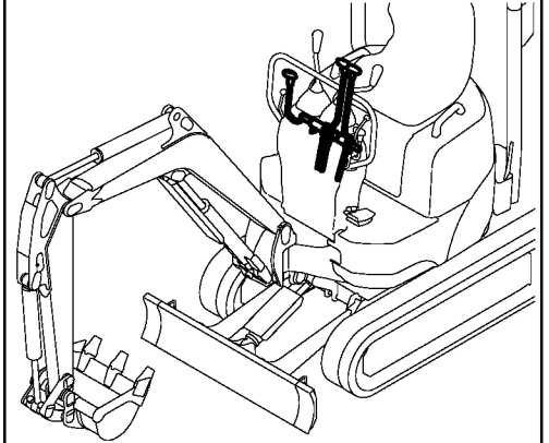
Fig. 18 CONTROL EQUIPMENT (TRAVEL & BLADE)
