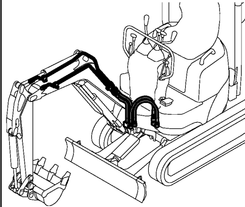
Fig. 53 HYD. OIL PIPING (P. T. O. : BOOM END)
