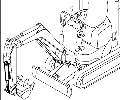
Fig. 29 BUCKET CYLINDER
