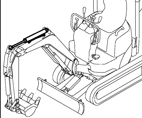
Fig. 28 ARM CYLINDER
