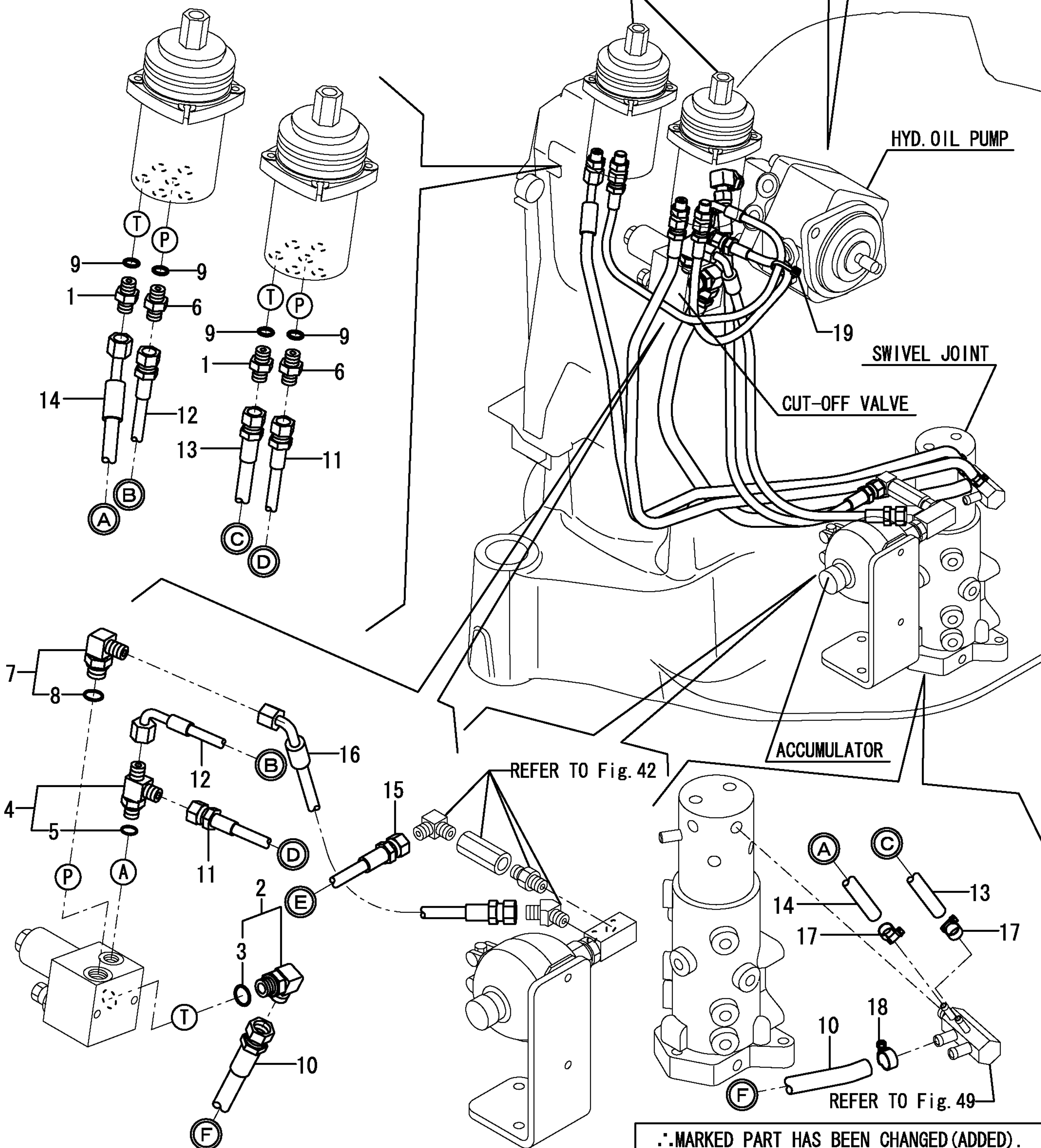
REMOTE CONTROL VALVE
