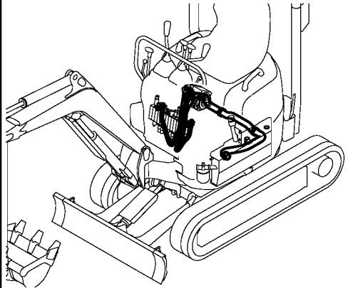
Fig. 46 HYD. OIL PIPING (TANK-PUMP-VALVE)
