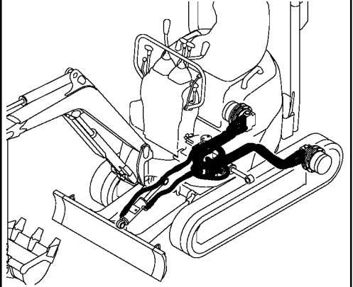
Fig. 51 HYD. OIL PIPING (TRACK FRAME)
