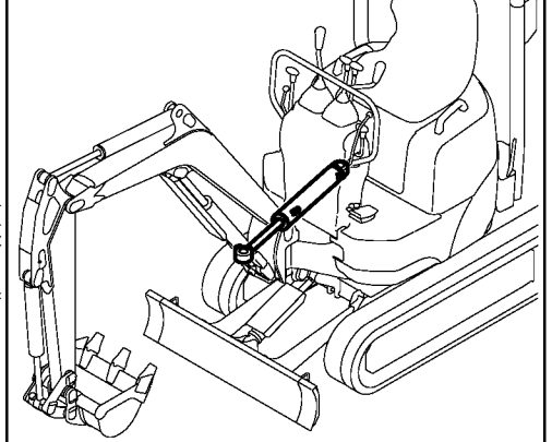
Fig. 30 SWING CYLINDER
