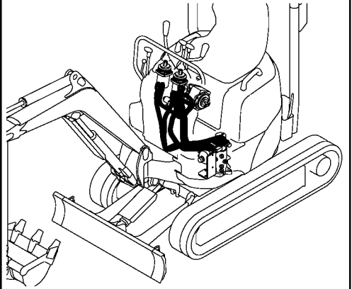
Fig. 54 CONTROL PIPING (PUMP-VALVE-RETURN)
