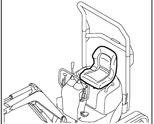
Fig. 24 SEAT & SEAT MOUNT
