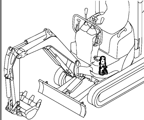
Fig. 35 SWIVEL JOINT
