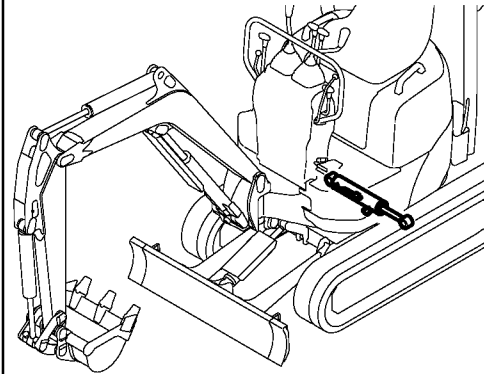
Fig. 32 VARIABLE LEG WIDEN/SHORTEN CYLINDER
