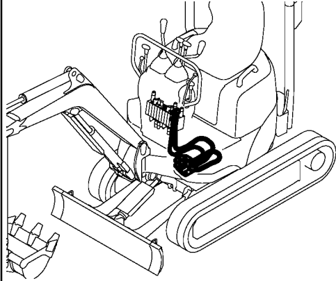
Fig. 50 HYD. OIL PIPING (P. T. O. : FRAME END)
