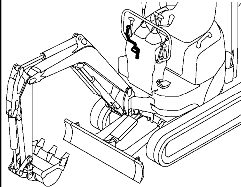
Fig. 20 CONTROL EQUIPMENT (VARIABLE LEG OPERATE)
