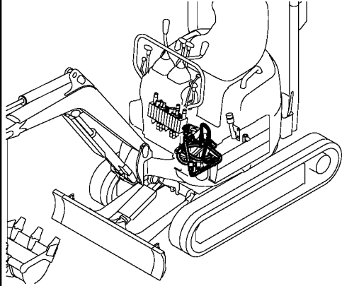
Fig. 49 HYD. OIL PIPING (RETURN)
