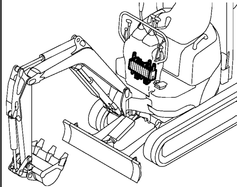
Fig. 41 CONTROL VALVE (TRAVEL : LEFT & P2 PORT)
