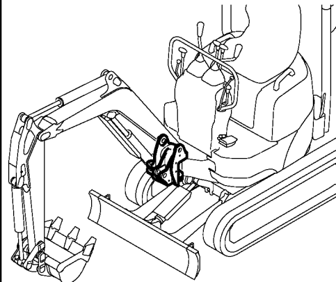
Fig. 58 BOOM BRACKET
