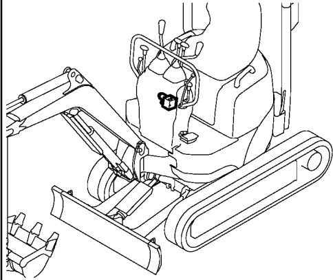
Fig. 44 CUT-OFF VALVE
