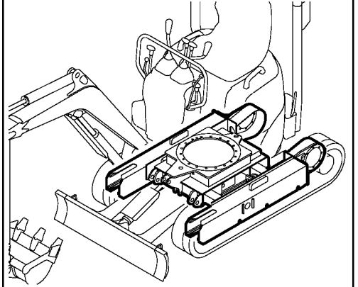
Fig. 21 TRACK FRAME
