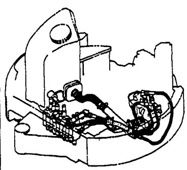
Fig. 38 HYD.OIL PIPING (VALVE ~ MOTOR, BOOM)
