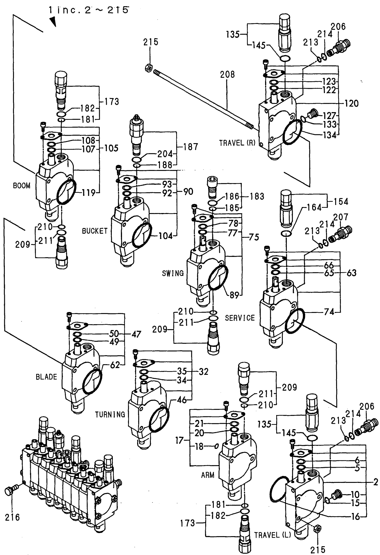
Fig. 34 CONTROL VALVE https://truckmanualshub.com/
