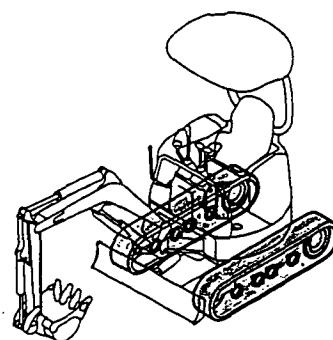
Fig. 12 CONTROL EQUIPMENT (LINK STAND & LEVER STOPPER)
