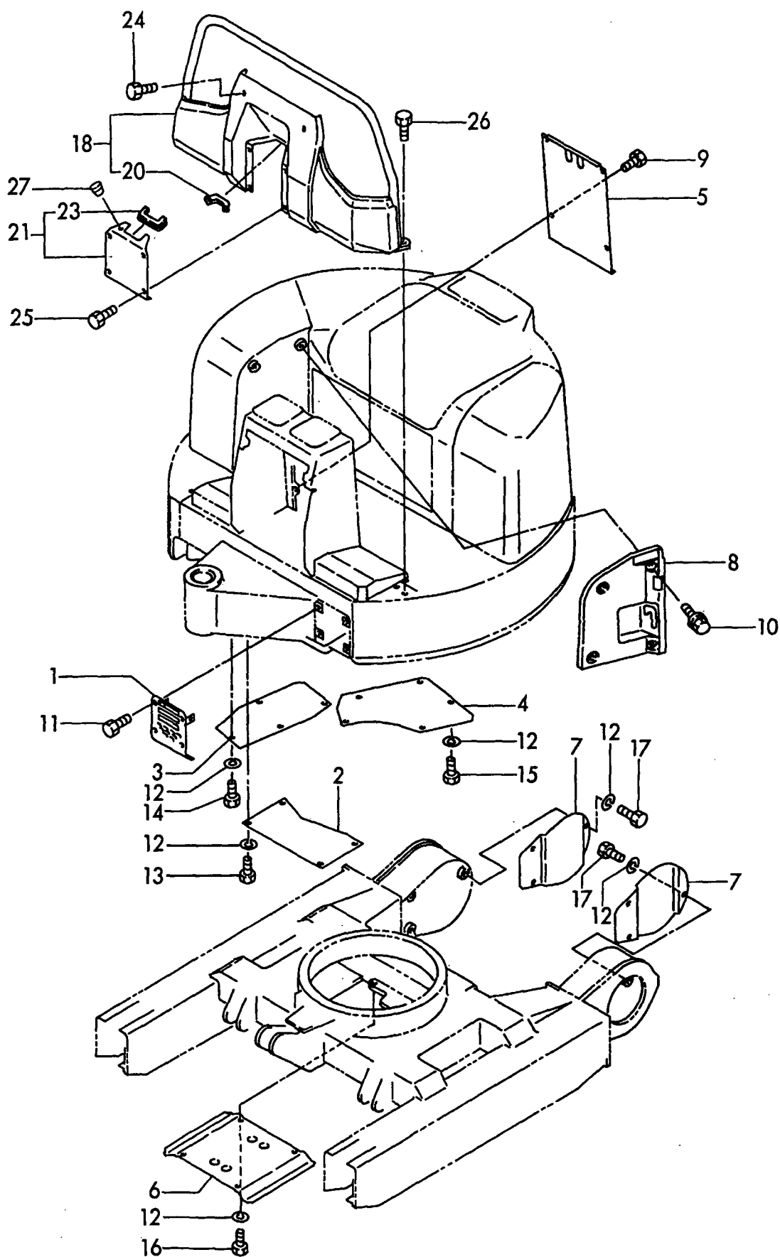
Fig. 20 FRAME COVER https://truckmanualshub.com/
