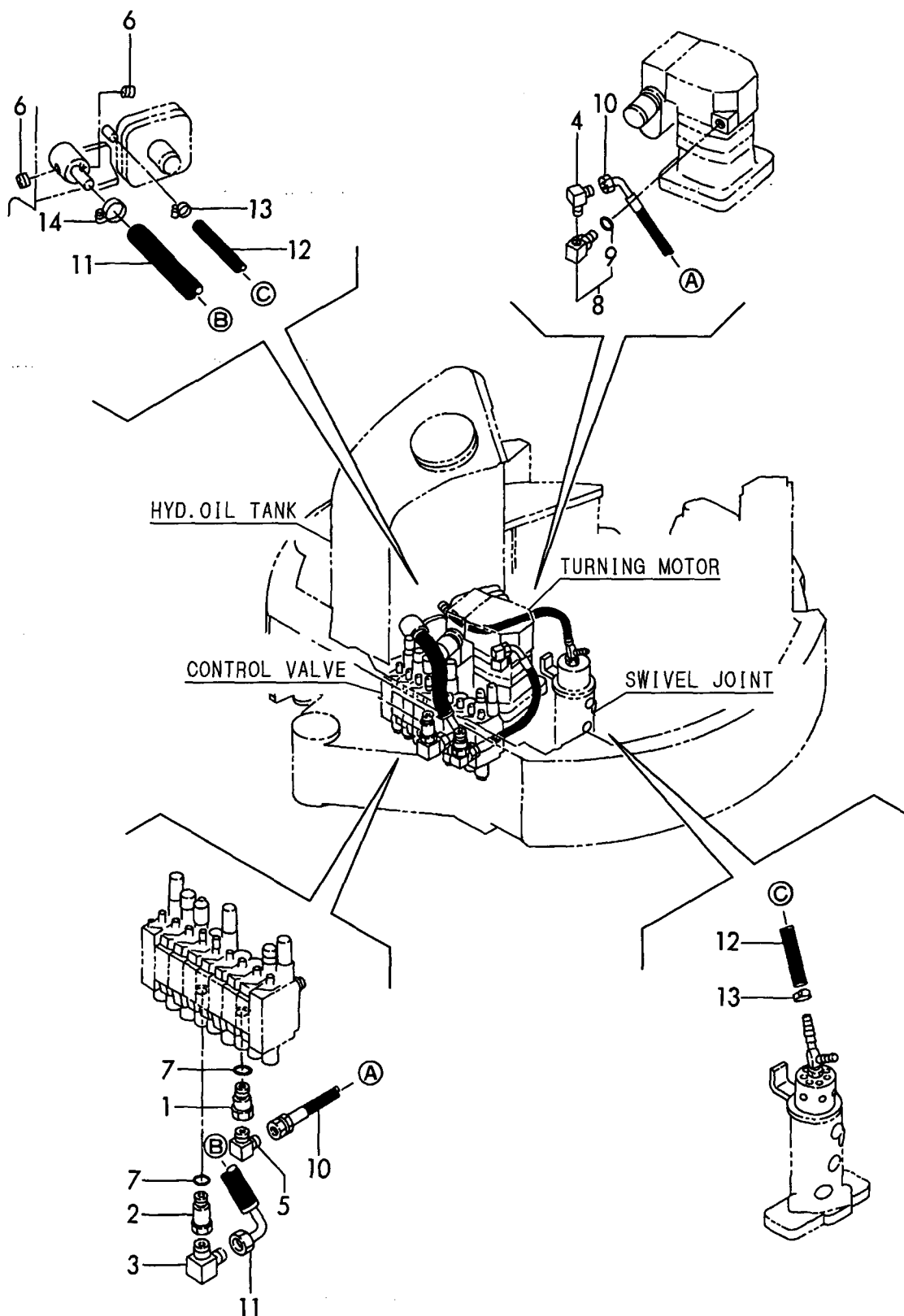
Fig. 40 HYD.OIL PIPING (RETURN) https://truckmanualshub.com/
