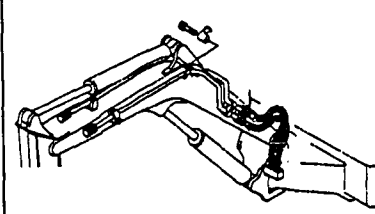
Fig. 44 HYD.OIL PIPING (P.T.O. ARM END)
