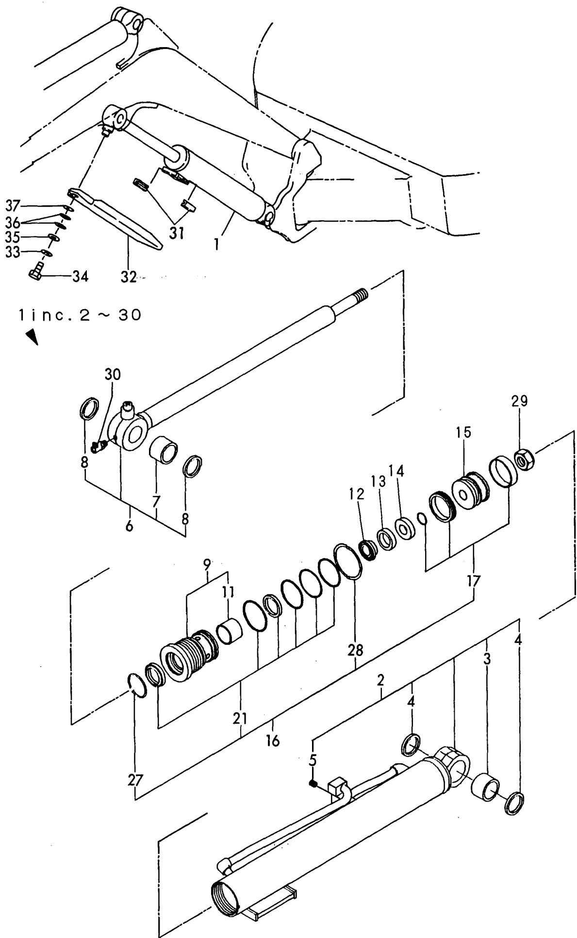
Fig. 26 BOOM CYLINDER https://truckmanualshub.com/
