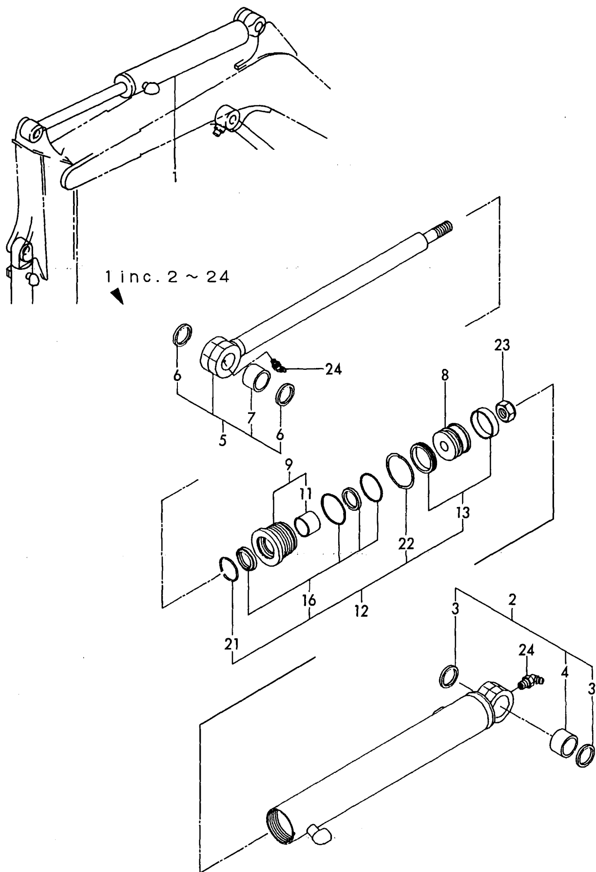
Fig. 27 ARM CYLINDER https://truckmanualshub.com/
