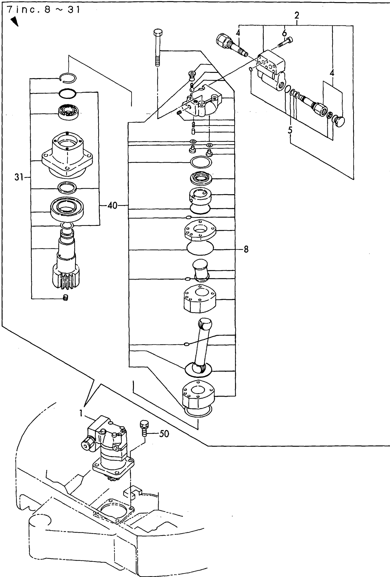
Fig. 32 TURNING MOTOR https://truckmanualshub.com/
