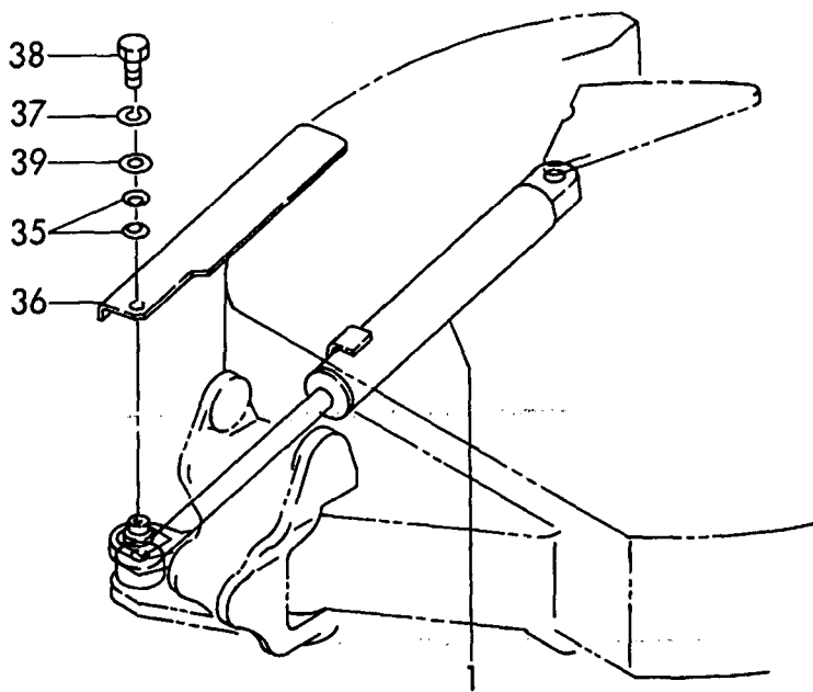
Fig. 29 SWING CYLINDER https://truckmanualshub.com/
