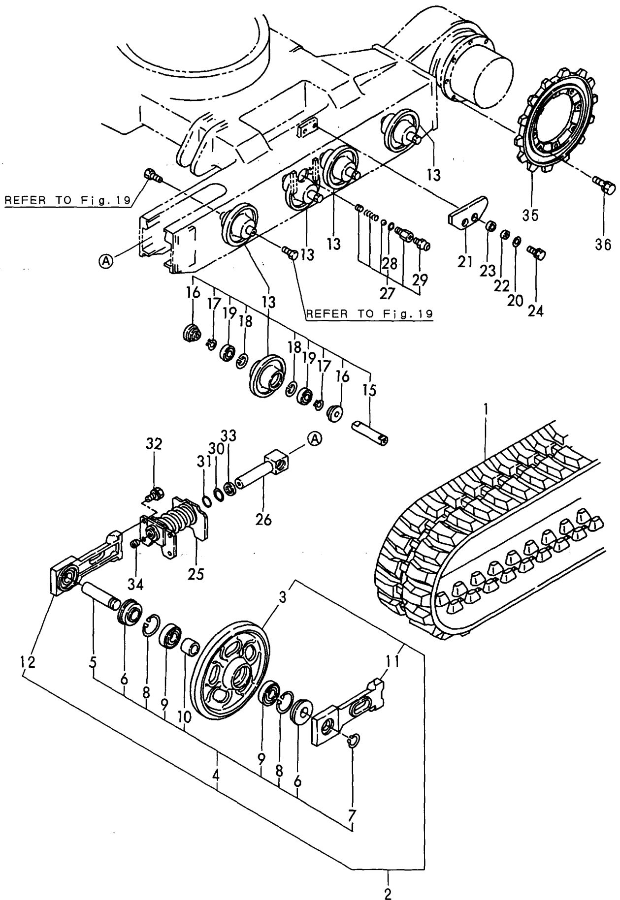
Fig. 11 CRAWLER, ROLLER & ADJUST
