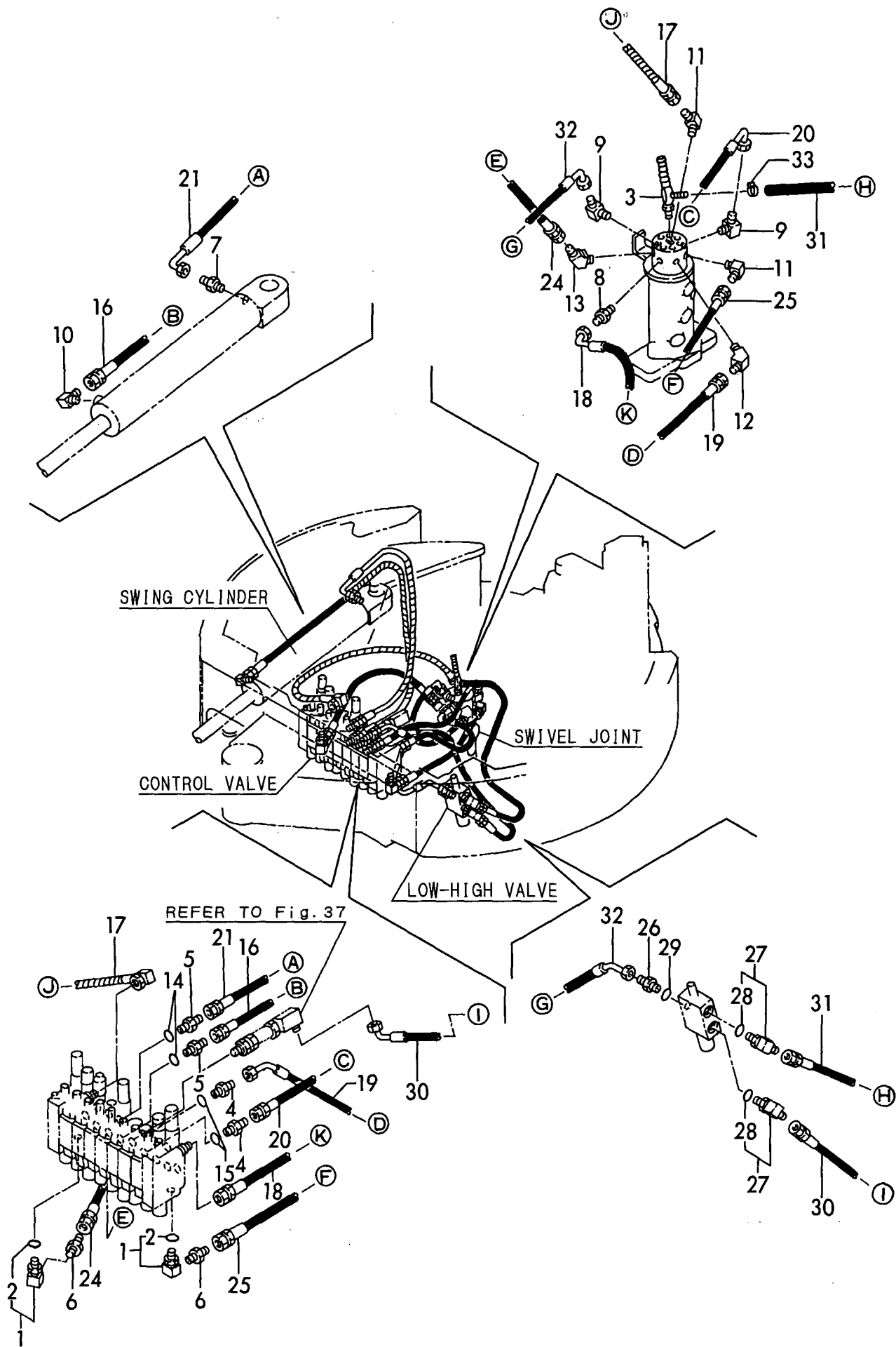
Fig. 39 HYD. OIL PIPING (VALVE ~ SWIVEL, SWING)
