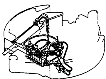
Fig. 39 HYD.OIL PIPING (VALVE ~ SWIVEL, SWING)
