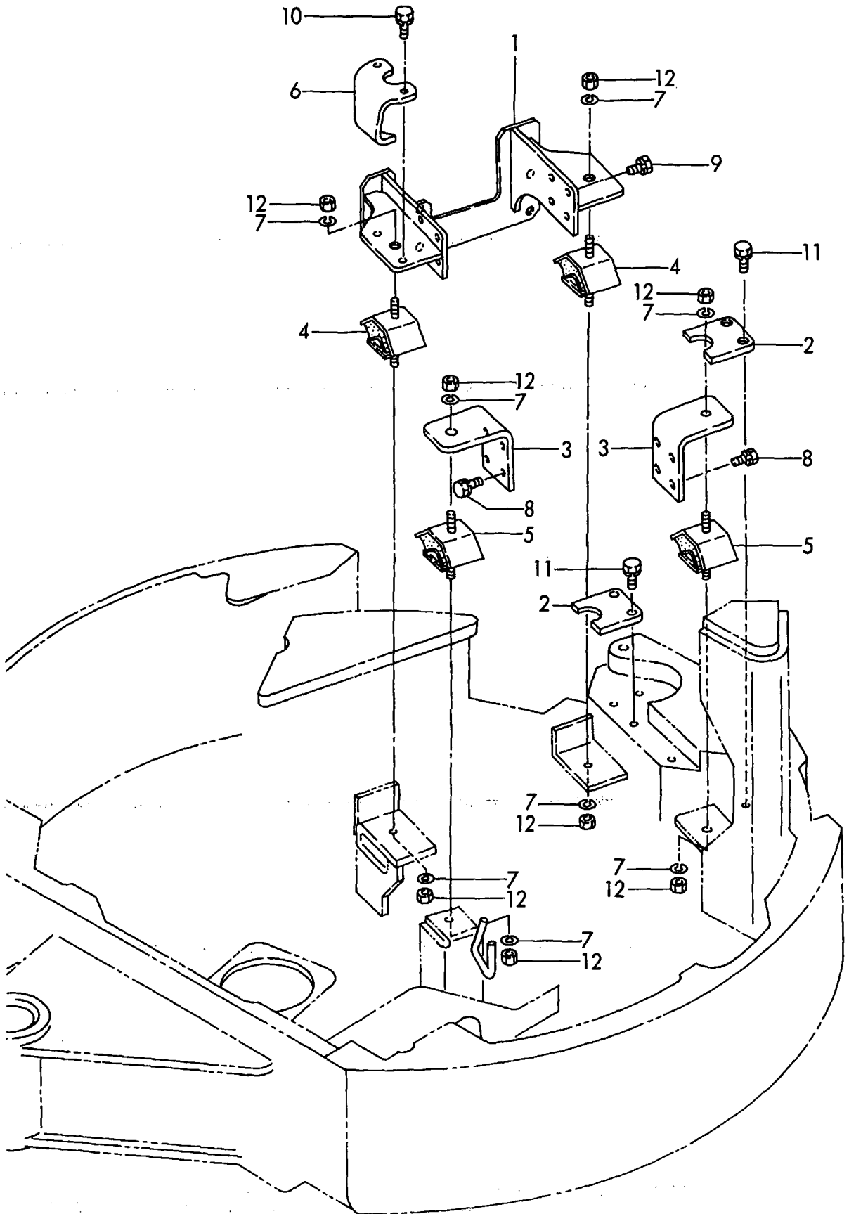
Fig. 5 ENGINE MOUNT
