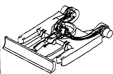
Fig. 43 HYD.OIL PIPING (BOOM)
