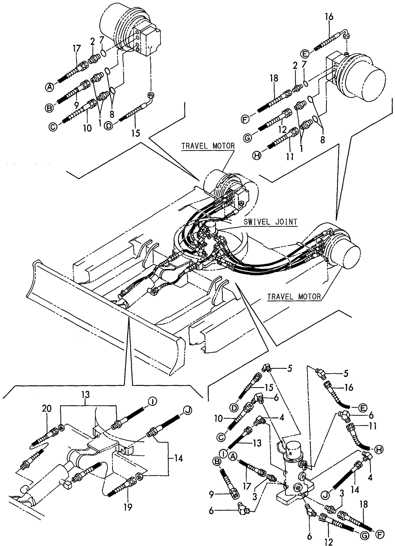
Fig. 42 HYD. OIL PIPING (TRAVEL) https://truckmanualshub.com/
