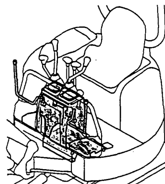
Fig. 12 CONTROL EQUIPMENT (LINK STAND & LEVER STOPPER)
