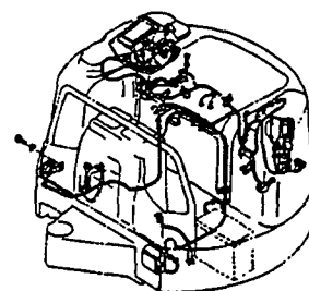
Fig. 10 WORK LAMP
