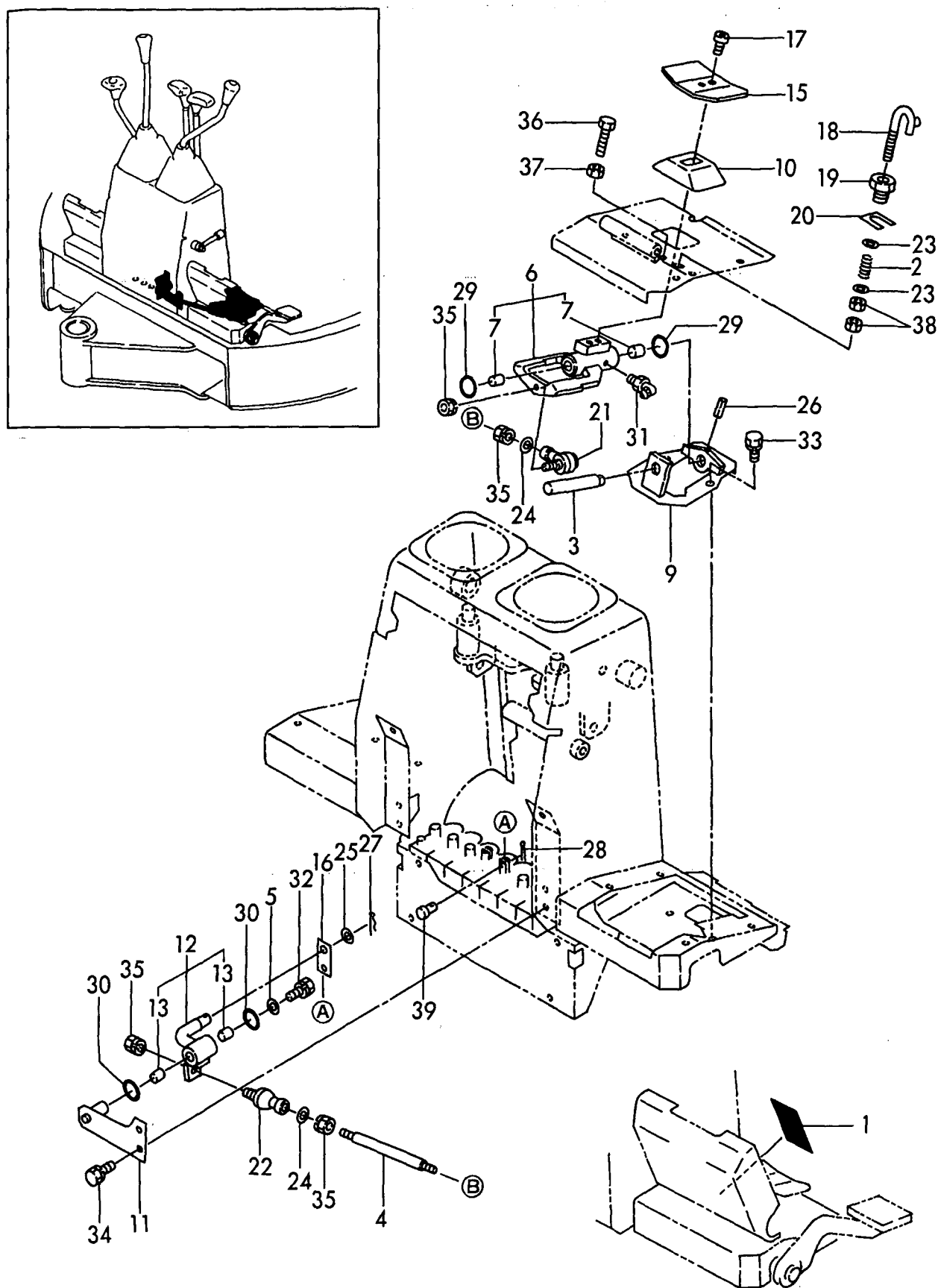
Fig. 18 CONTROL EQUIPMENT (P. T. O. CONTROL)
