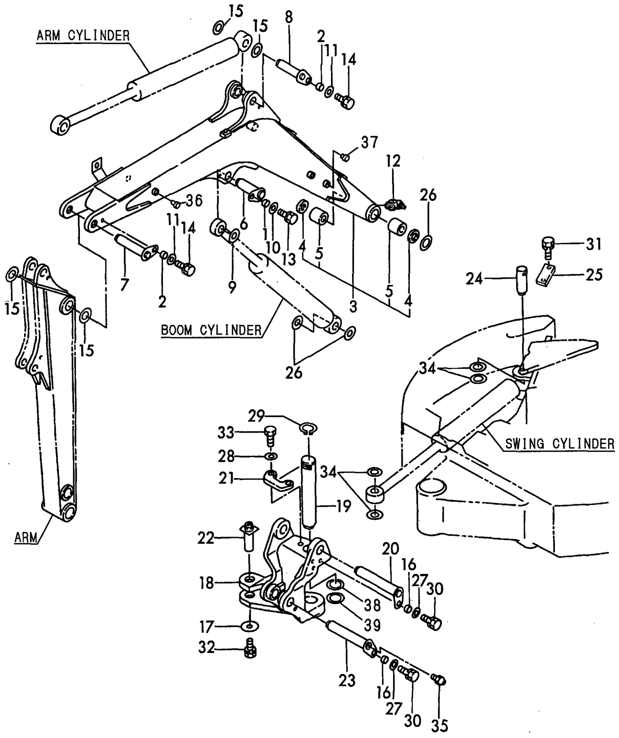
Fig. 46 BOOM & BOOM BRACKET https://truckmanualshub.com/
