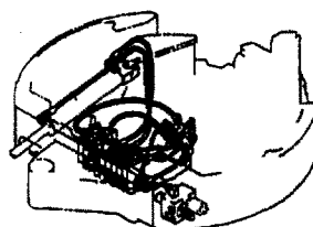
Fig. 56 油圧配管 (リターン) (旧形) HYD. OIL PIPING (RETURN) (PREVIOUS)
