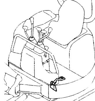
Fig. 24 操縦装置 (ロー・ハイペダル) (旧形) CONTROL EQUIPMENT (LOW-HIGH PEDAL) (PREVIOUS)
