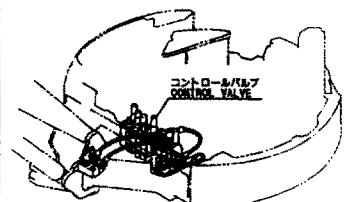
Fig. 59 油圧配管 (走行) HYD. OIL PIPING (TRAVEL)
