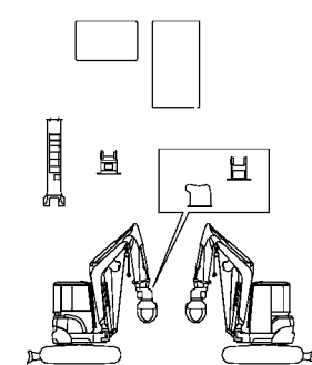
Fig. 12 安全銘板(林業) (JP) SAFETY LABEL (FORESTRY) (JP)
