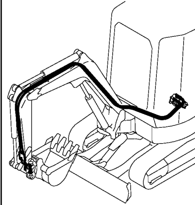
Fig. 138 油圧配管 (グラブドル, 1) (林業: 電磁仕様) HYD. OIL PIPING (GRAPPLE, 1) (FORESTRY: ELECTRICAL SPEC.)
