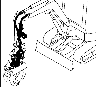
Fig. 140 油圧配管 (グラブドル, 3) (林業: 電磁仕様) HYD. OIL PIPING (GRAPPLE, 3) (FORESTRY: ELECTRICAL SPEC.)
