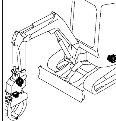
Fig. 120 バルブ (林業:電磁仕様) VALVE (FORESTRY: ELECTRICAL SPEC.)
