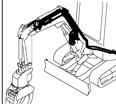
Fig. 143 油圧配管 (グラブドル, 3) (林業: 効仕様) HYD. OIL PIPING (GRAPPLE, 3) (FORESTRY: MECHANICAL SPEC.)
