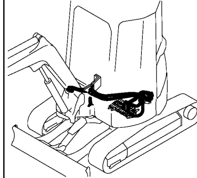
Fig. 142 油圧配管 (グラブドル, 2) (林業: 効仕様) HYD. OIL PIPING (GRAPPLE, 2) (FORESTRY: MECHANICAL SPEC.)
