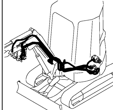
Fig. 144 油圧配管 (ウインチ) (林業仕様) HYD. OIL PIPING (WINCH) (FORESTRY SPEC.)
