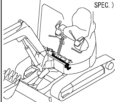
Fig. 62 操縦装置 (PTOリンク) (林業:効仕様) CONTROL EQUIPMENT (P. T. O. LINK) (FORESTRY: MECHANICAL SPEC.)
