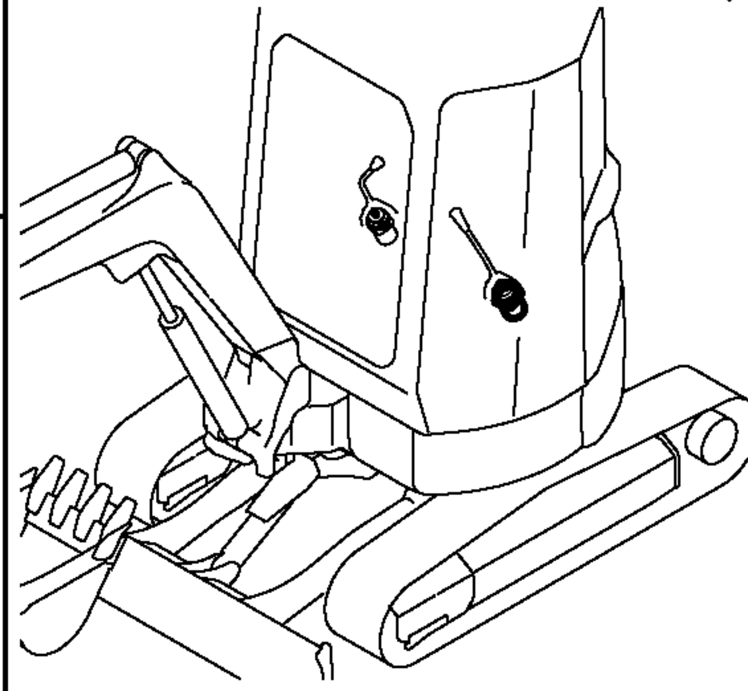
リモコンバルブ (標準: M/#25501~, 2ウェイ仕様) Fig. 123 REMOTE CONTROL VALVE (STANDARD: FROM M/#25501, 2-WAY SPEC.)
