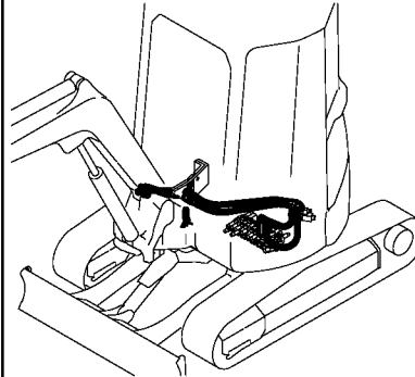
Fig. 139 油圧配管 (グラブドル, 2) (林業: 電磁仕様) HYD. OIL PIPING (GRAPPLE, 2) (FORESTRY: ELECTRICAL SPEC.)
