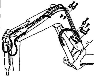
Fig.54 油圧配管 (3RDバルブ、ブーム) HYD.OIL PIPING (3RD VALVE, BOOM)
