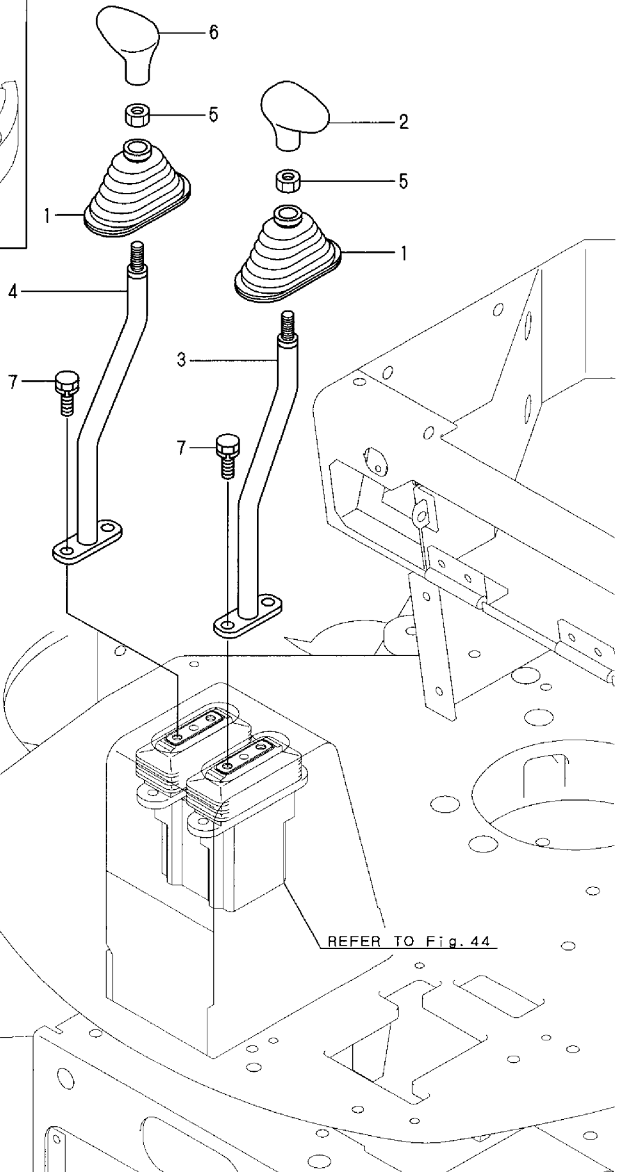
Fig. 14 操縦装置 (走行) CONTROL EQUIP. (TRAVEL)
