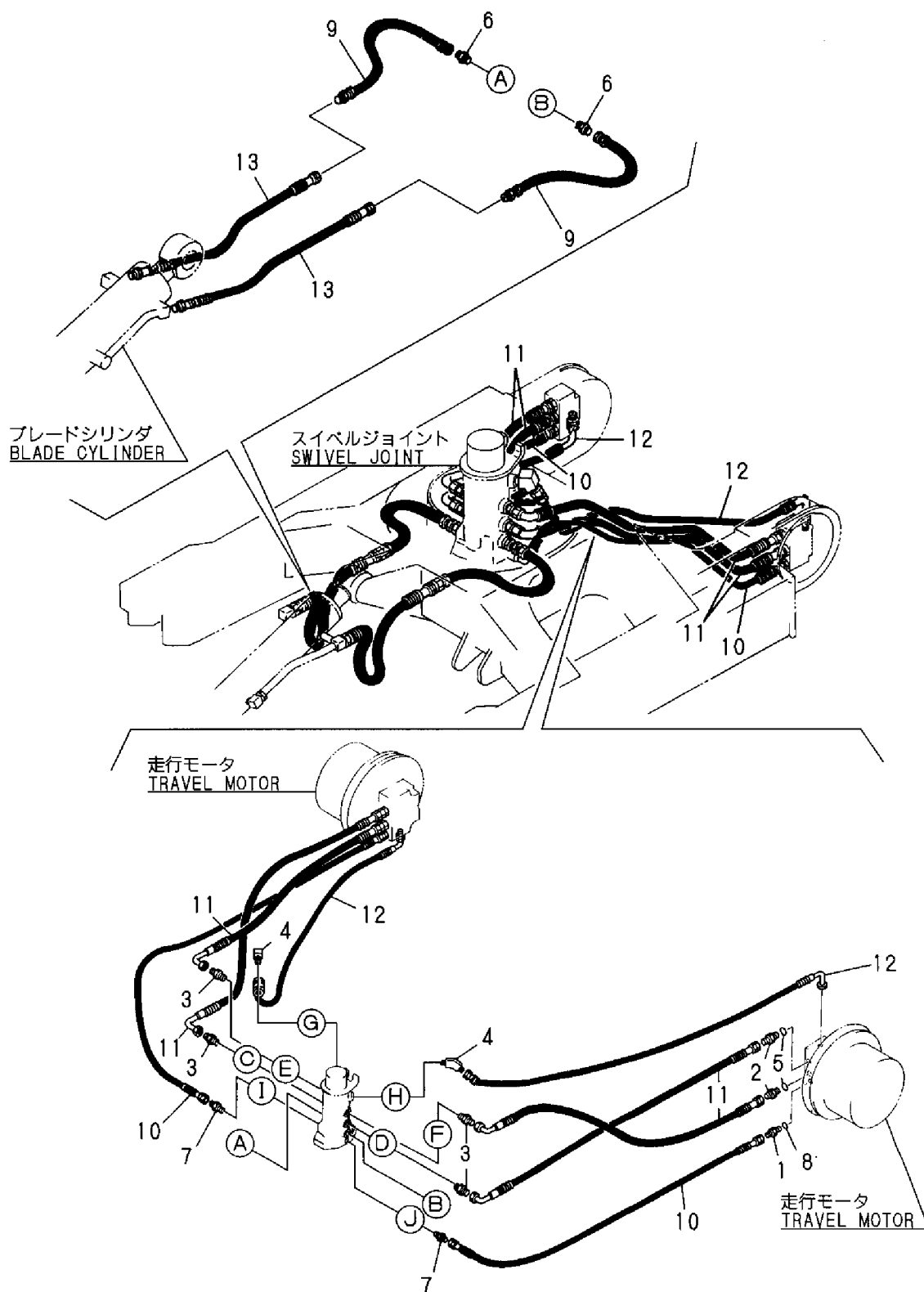
Fig. 52 油圧配管 (走行) HYD. OIL PIPING (TRAVEL)
