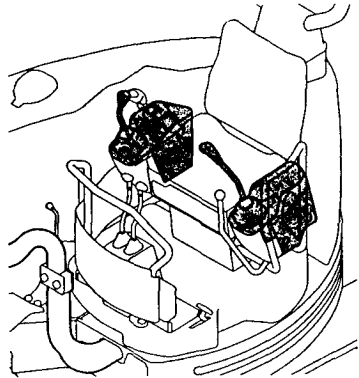
Fig.14 操縦装置 (走行) CONTROL EQUIP. (TRAVEL)
