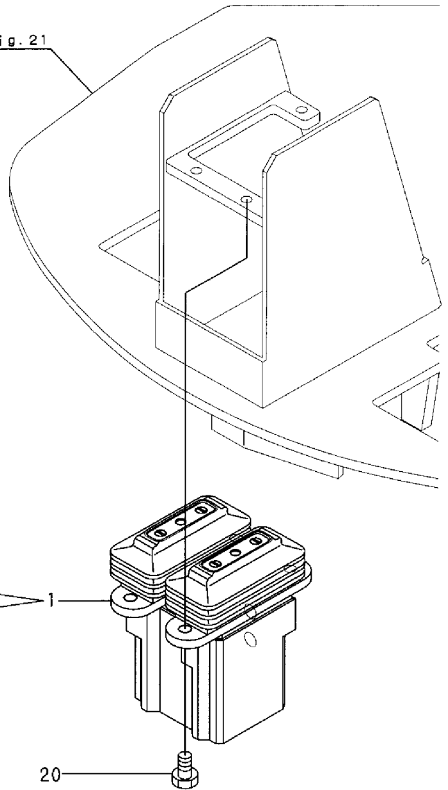
Fig. 44 リモコンバルブ (走行) REMOTE CONTROL VALVE (TRAVEL)
