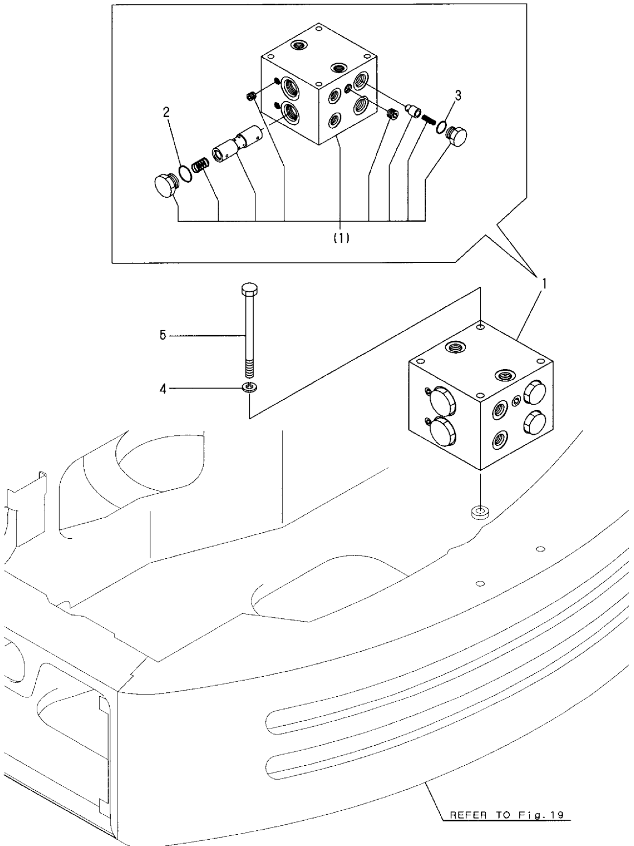
Fig. 43 分流弁 TRIBUTARY VALVE
