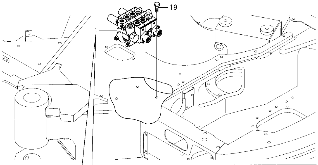
Fig. 45 切替バルブ CHANGE OVER VALVE
