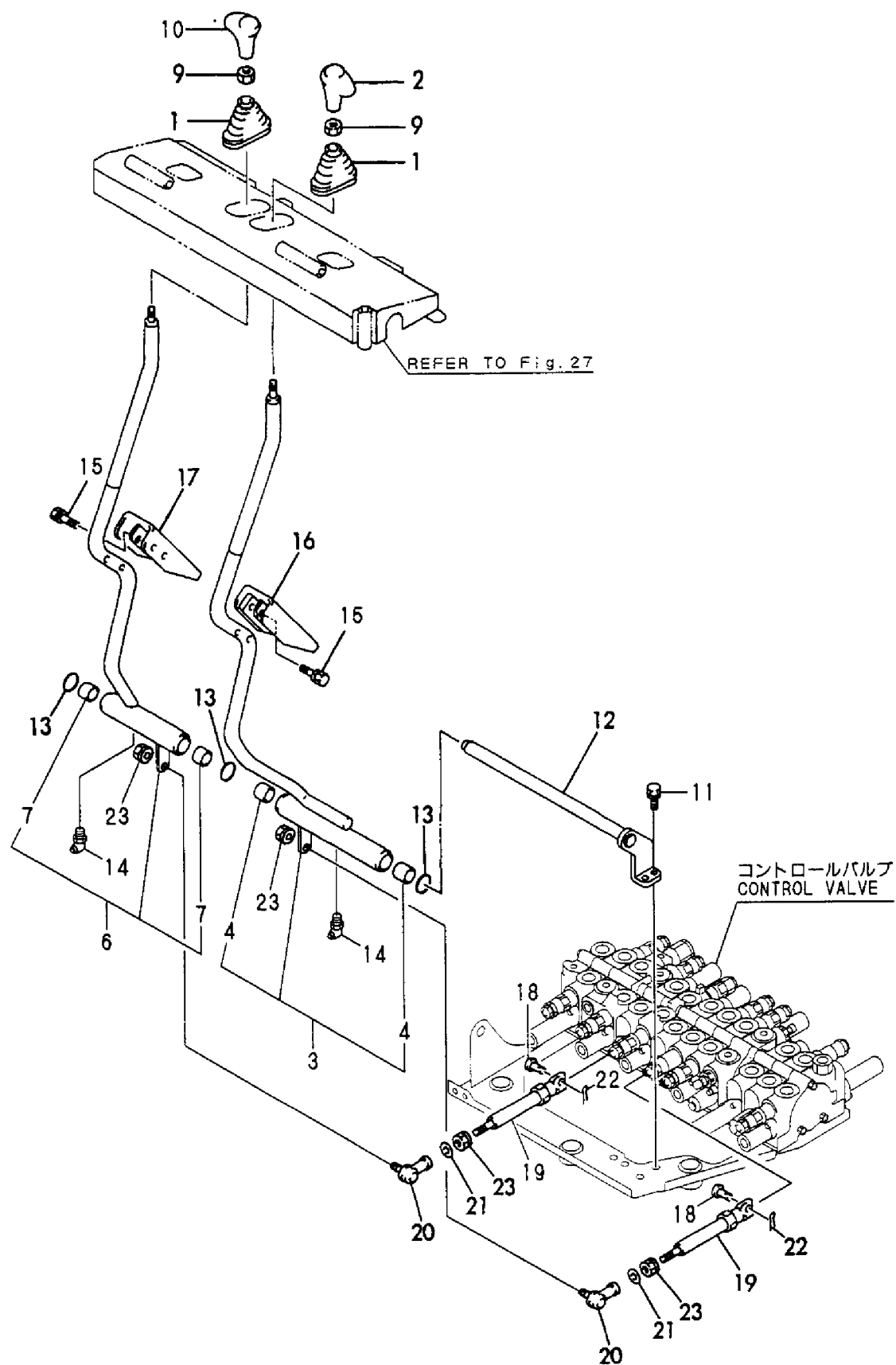
Fig. 29 操縦装置 (走行) CONTROL EQUIP. (TRAVEL)
