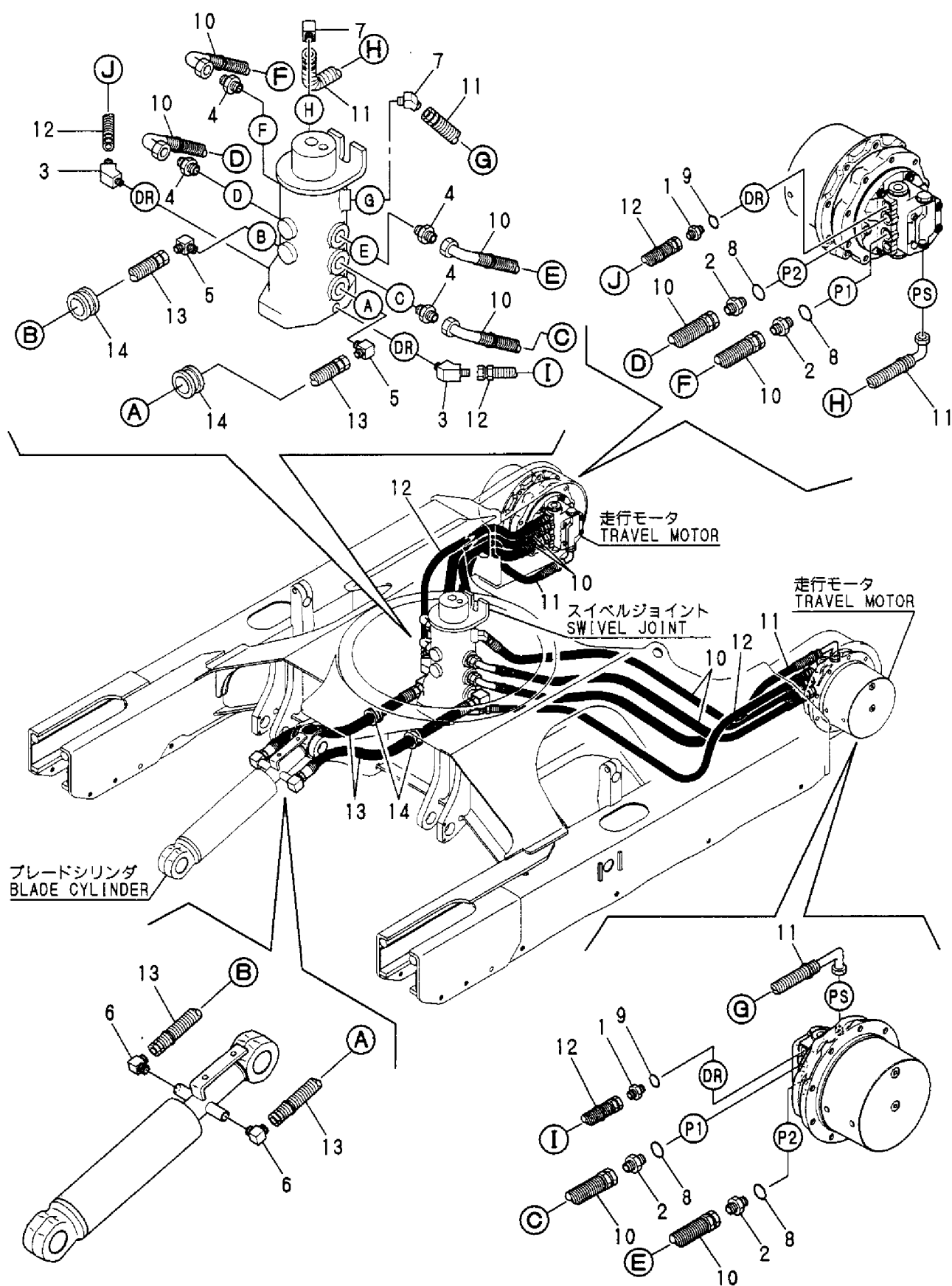
Fig. 74 油圧配管 (走行) HYD. OIL PIPING (TRAVEL)
