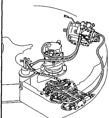
Fig. 74 油圧配管 (走行) HYD. OIL PIPING (TRAVEL)
