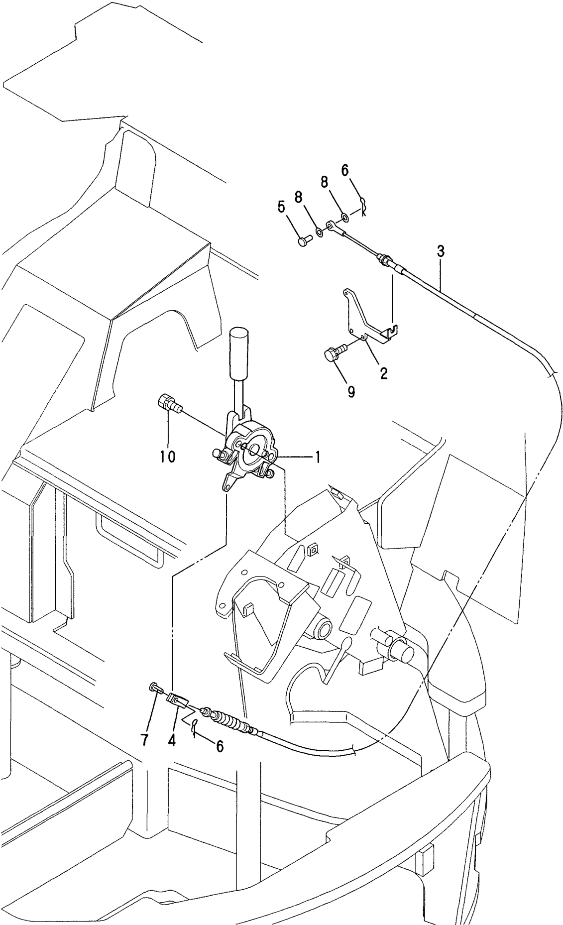
Fig. 4 ACCELERATOR
