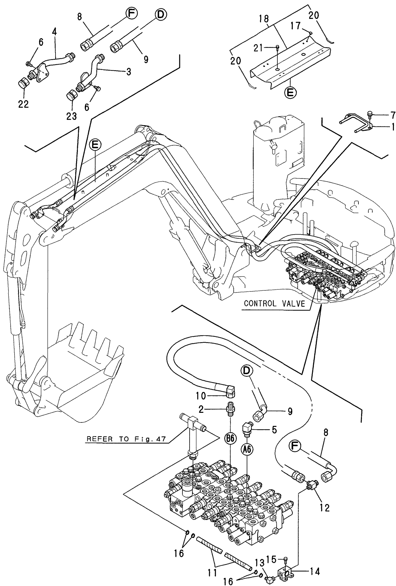
Fig. 50 HYD. OIL PIPING (P.T.O.) https://truckmanualshub.com/
