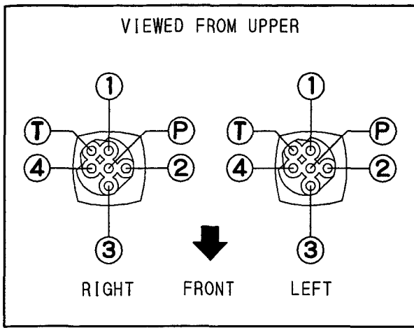
Fig. 51 CONTROL PIPING (PUMP~REMO.-CON. V. ~RETURN)
