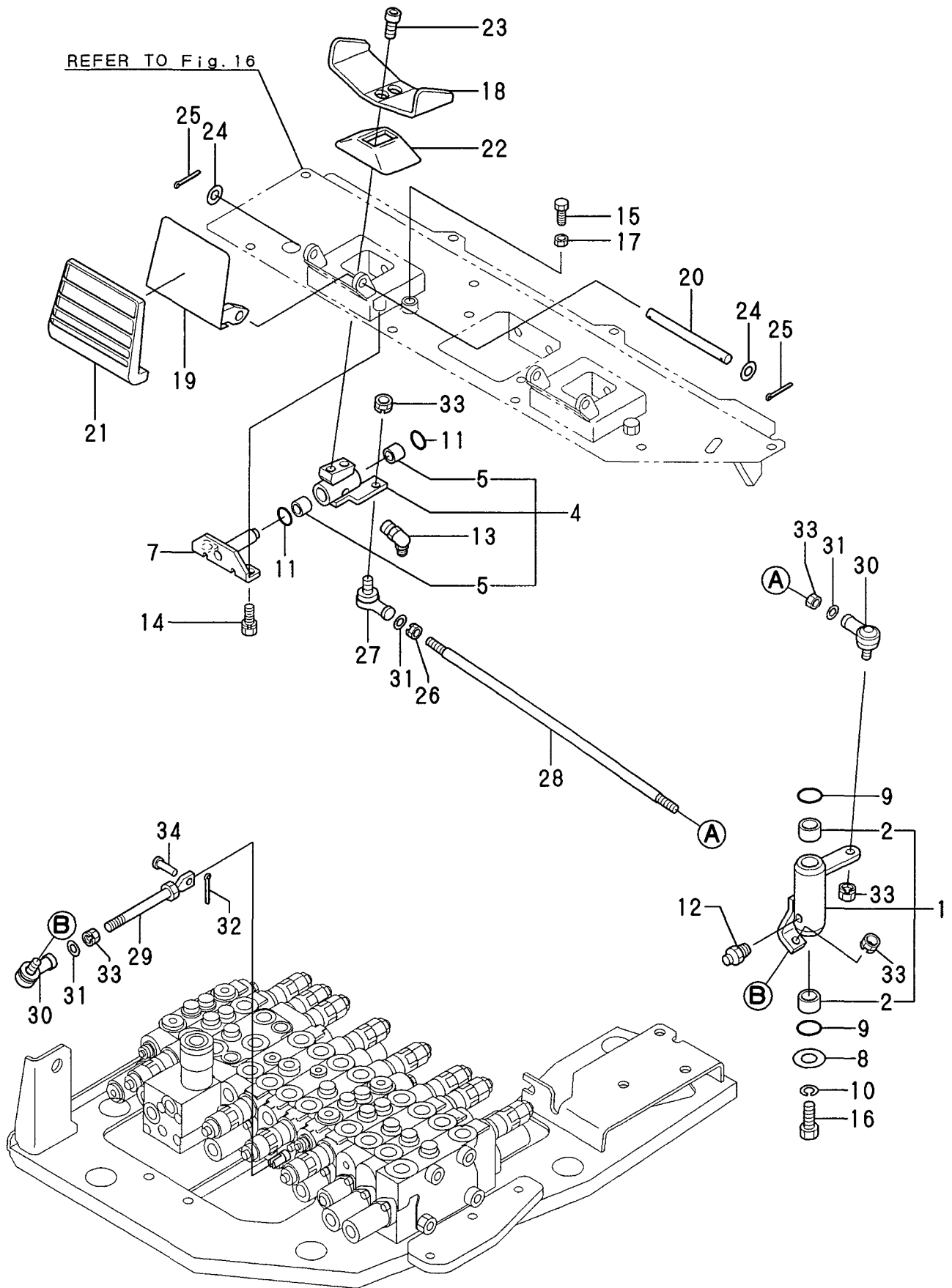
Fig. 18 CONTROL EQUIPMENT (SWING PEDAL)
