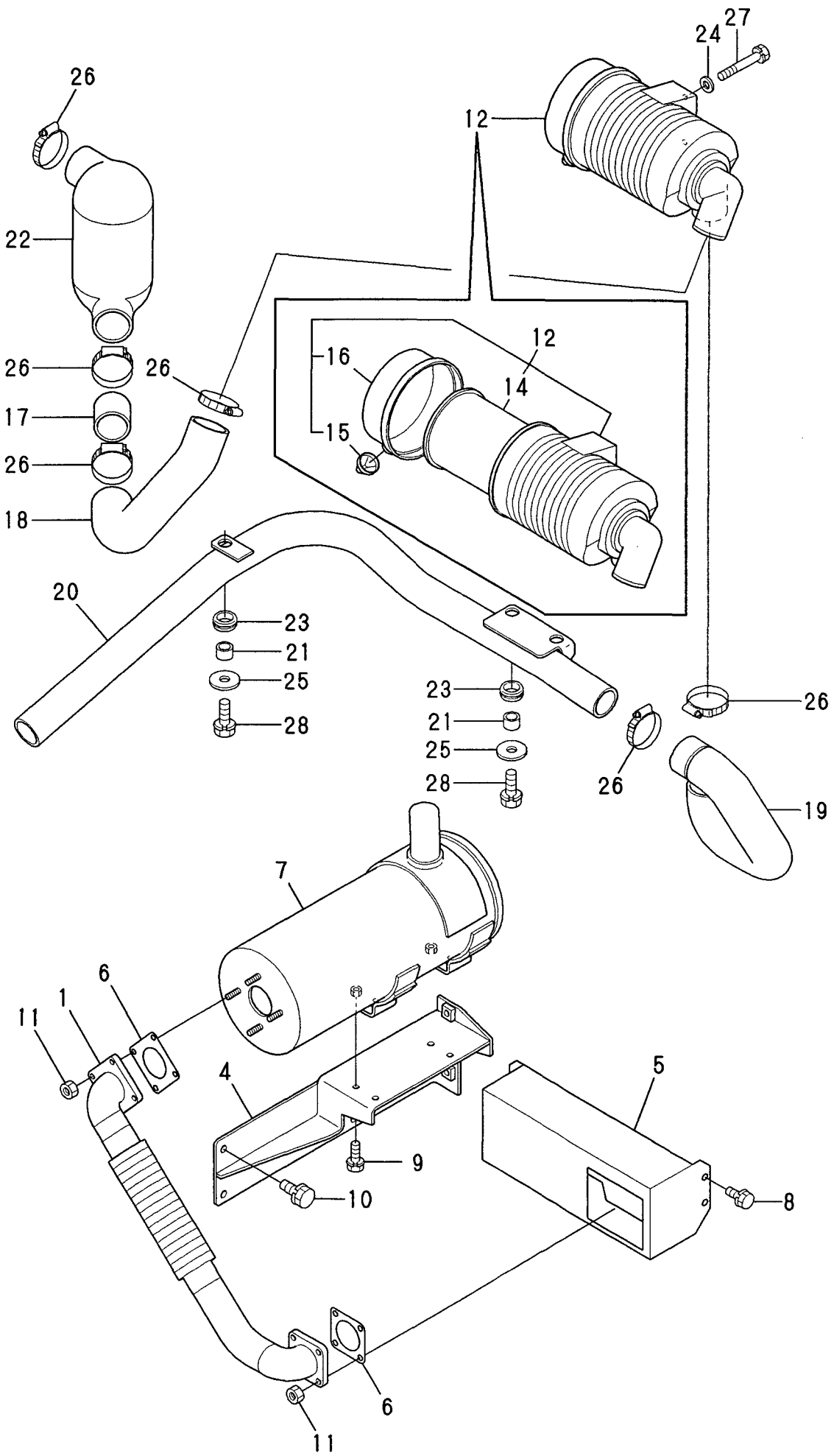
Fig. 3 SILENSER & AIR CLEANER
