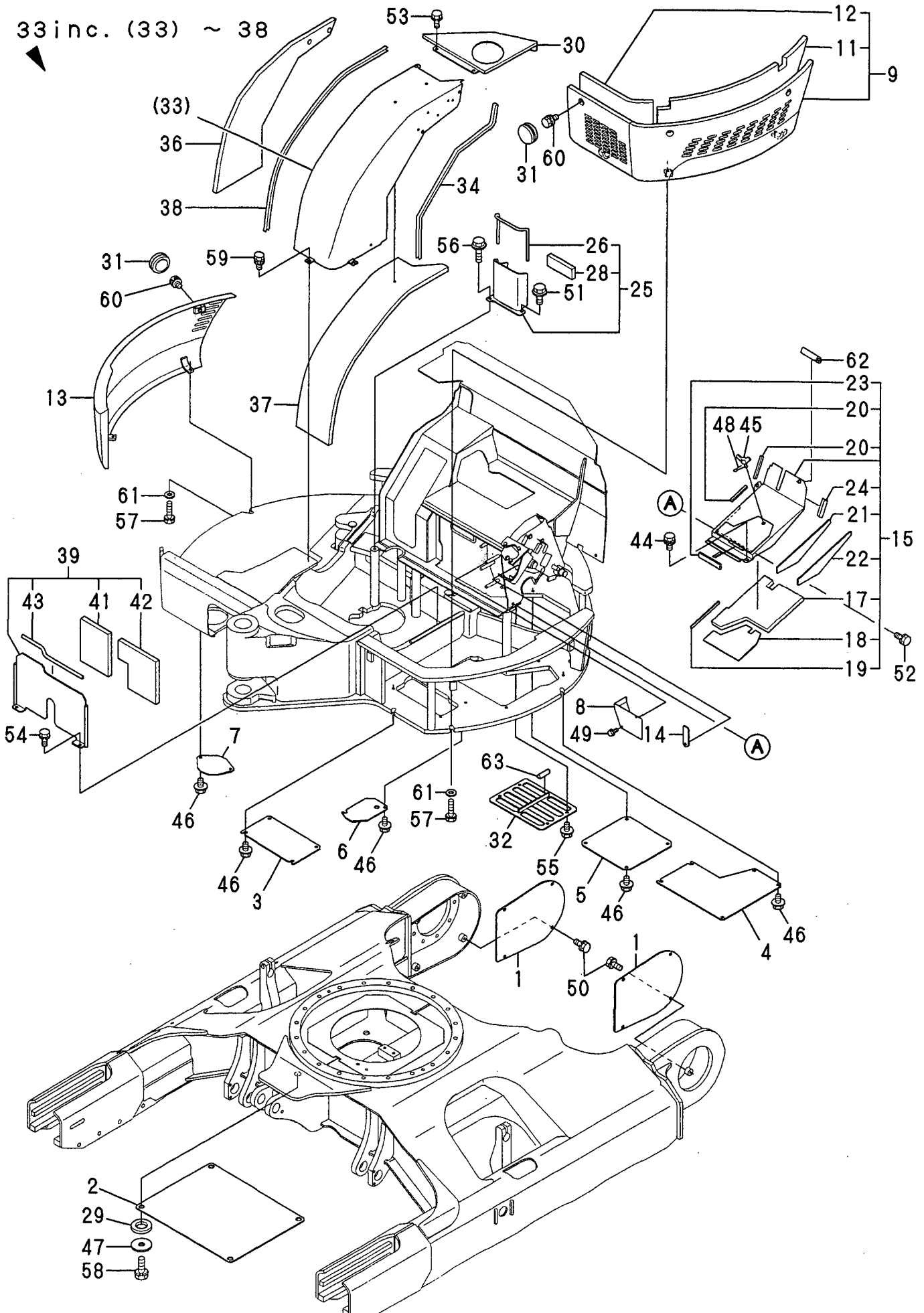
Fig. 22 COVER (FRAME)
