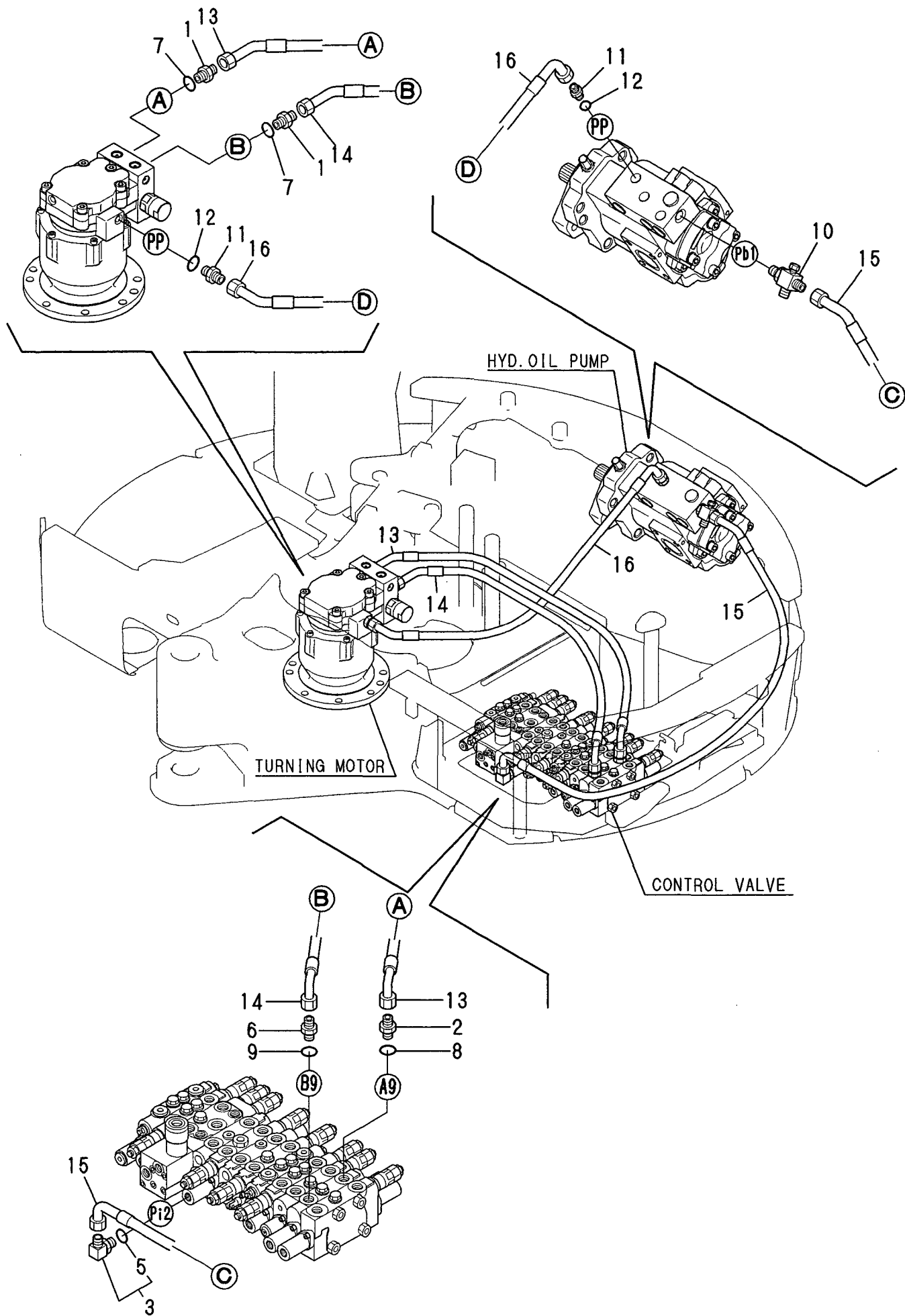
Fig. 45 HYD. OIL PIPING (PUMP~VALVE~MOTOR) https://truckmanualshub.com/
