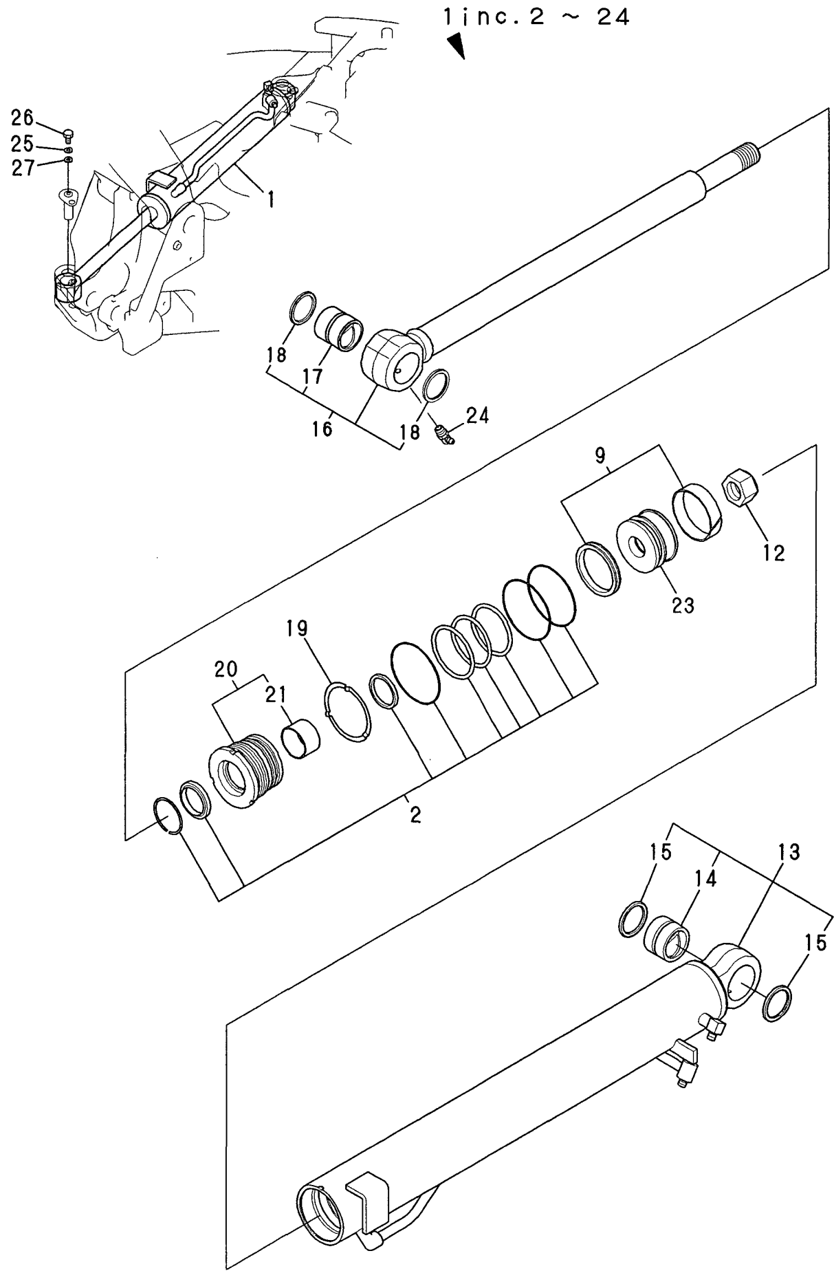
Fig. 32 SWING CYLINDER
