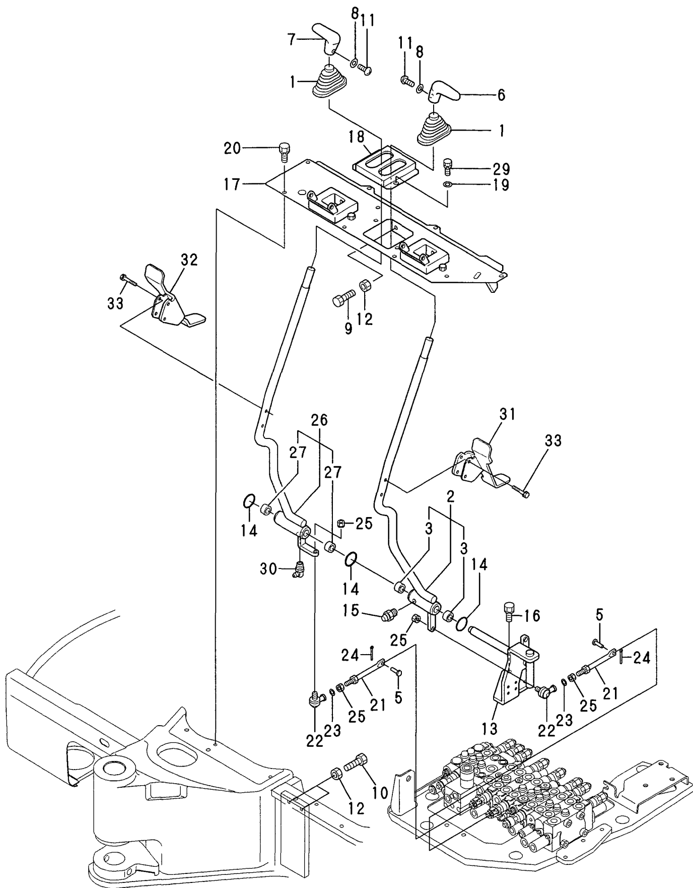
Fig. 16 https://truckmanualshub.com/ CONTROL EQUIPMENT (TRAVEL LEVER)
