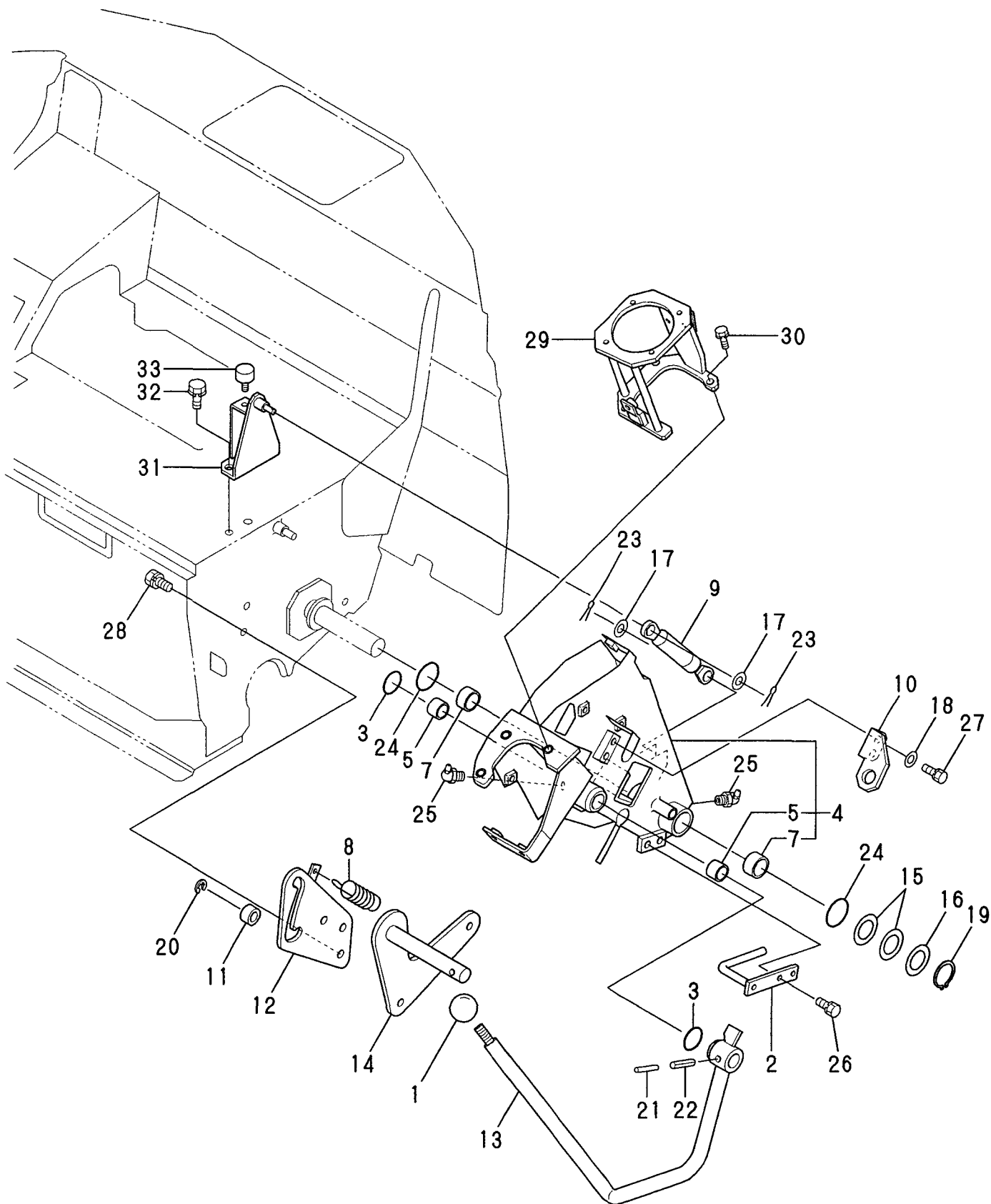
Fig. 15 https://truckmanualshub.com/ CONTROL EQUIPMENT (LOCK LEVER & STAND) LEFT
