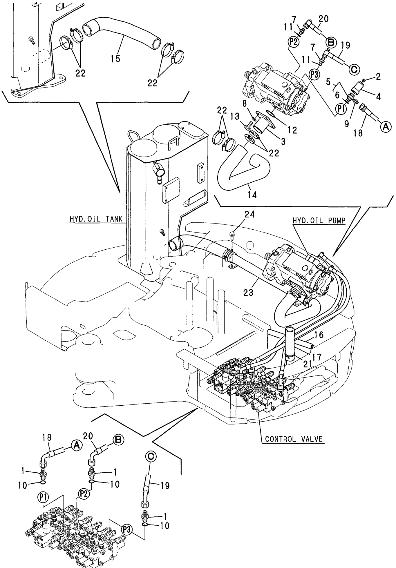
Fig. 44 HYD. OIL PIPING (TANK~PUMP~VALVE)
