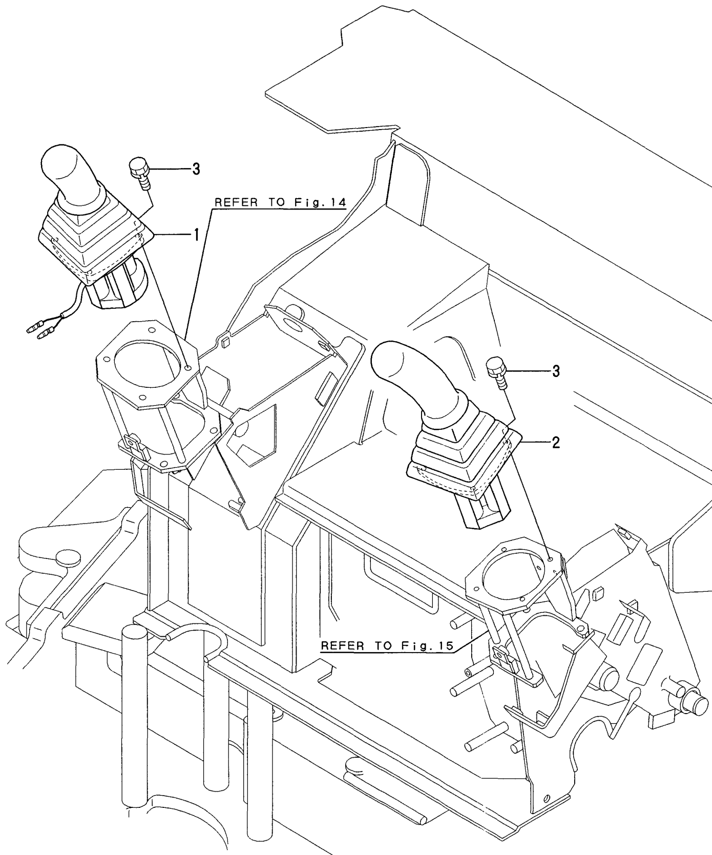
Fig. 42 REMOTE CONTROL VALVE
