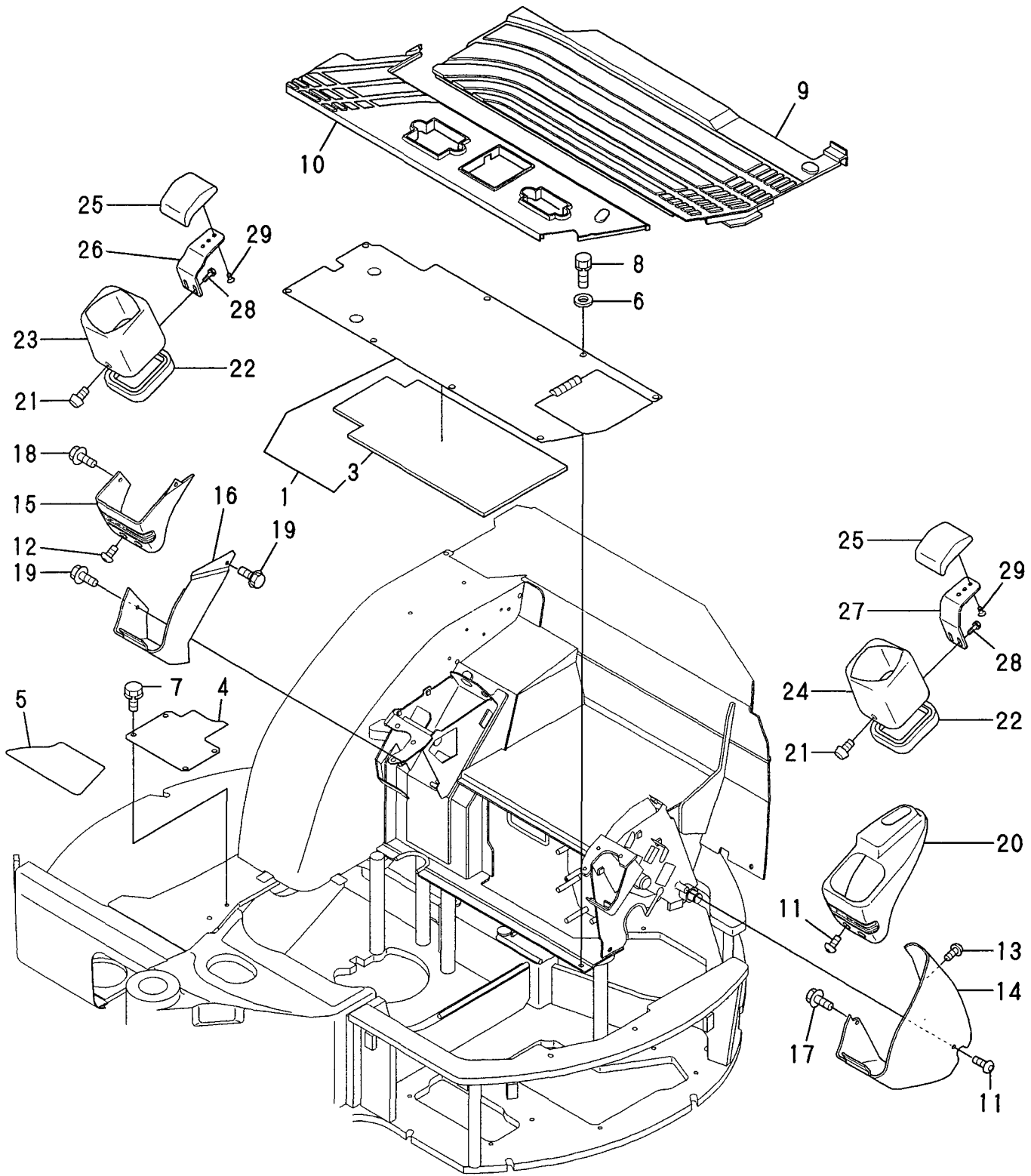
Fig. 24 STEP & INSTRUMENT PANEL
