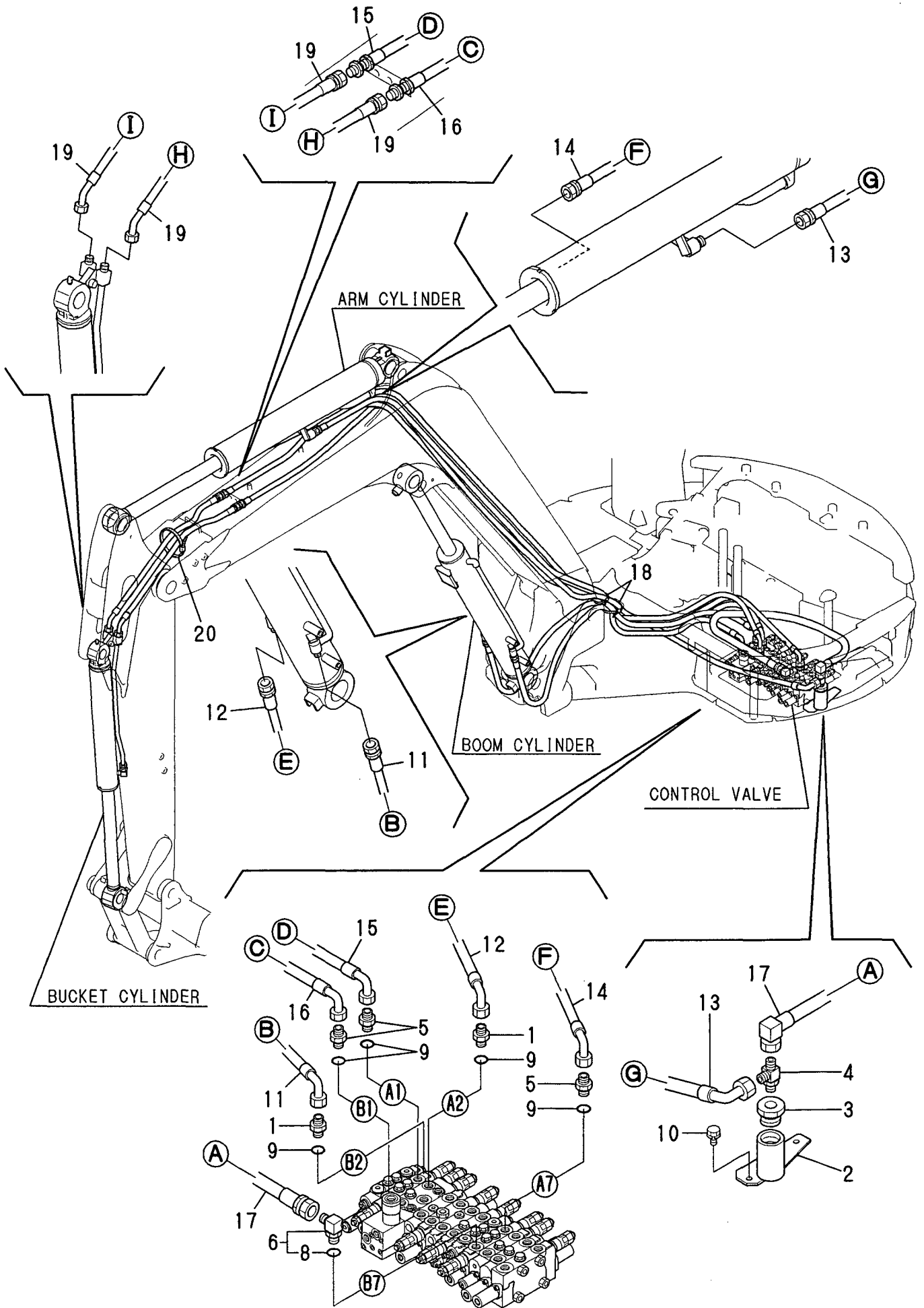
Fig. 49 HYD. OIL PIPING (BOOM)
