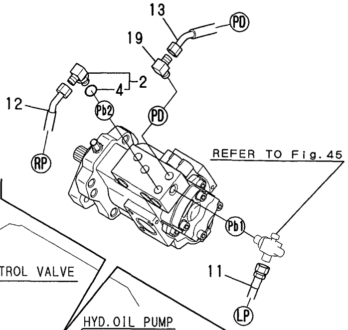
Fig. 51 CONTROL PIPING (PUMP~REMO.-CON. V. ~RETURN)
