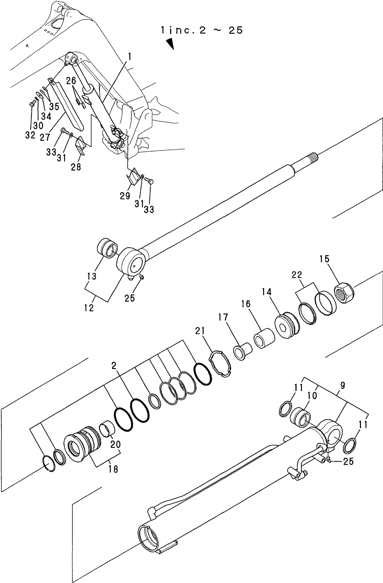
Fig. 29 BOOM CYLINDER
