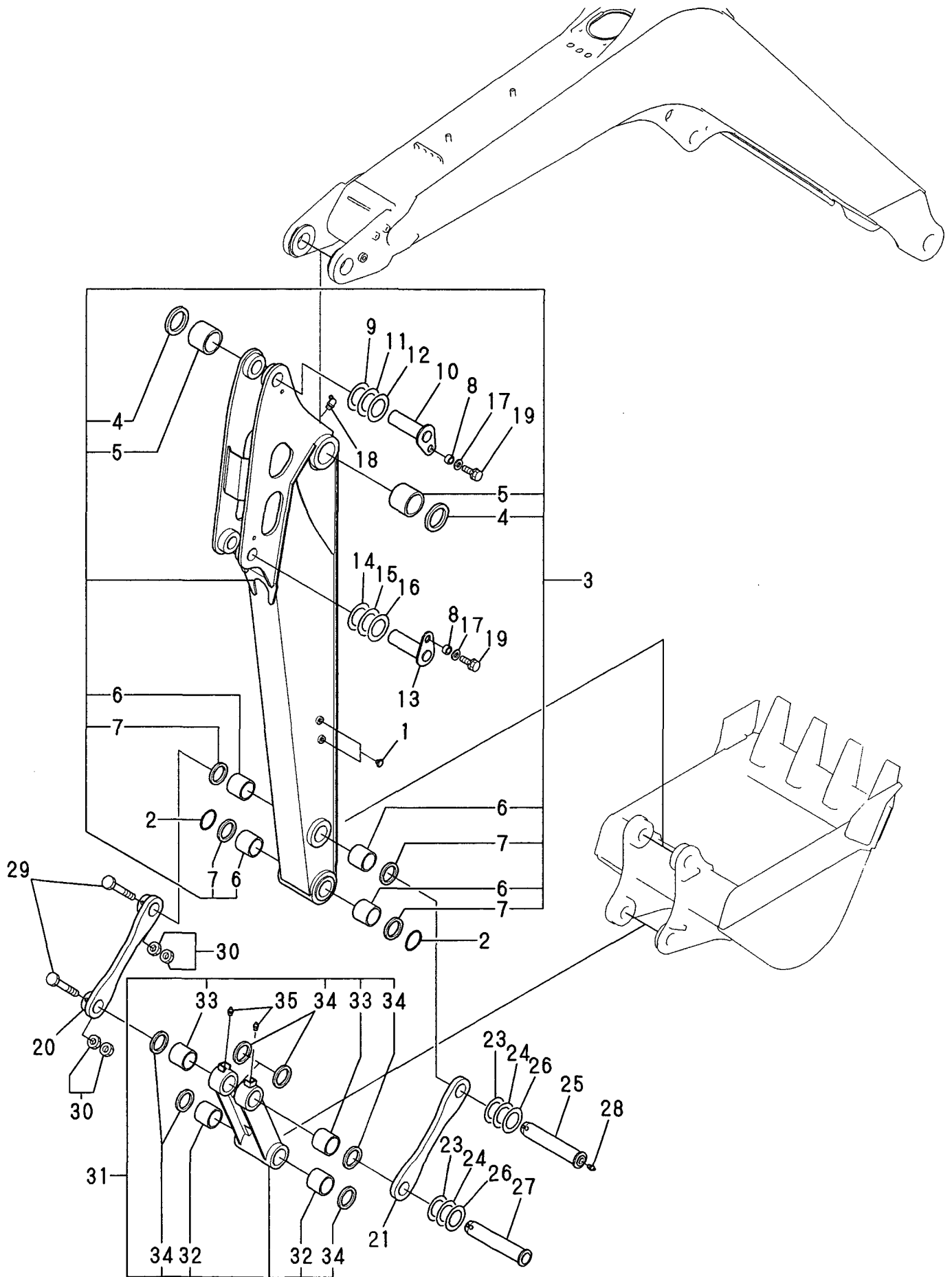
Fig. 55 ARM & BUCKET LINK
