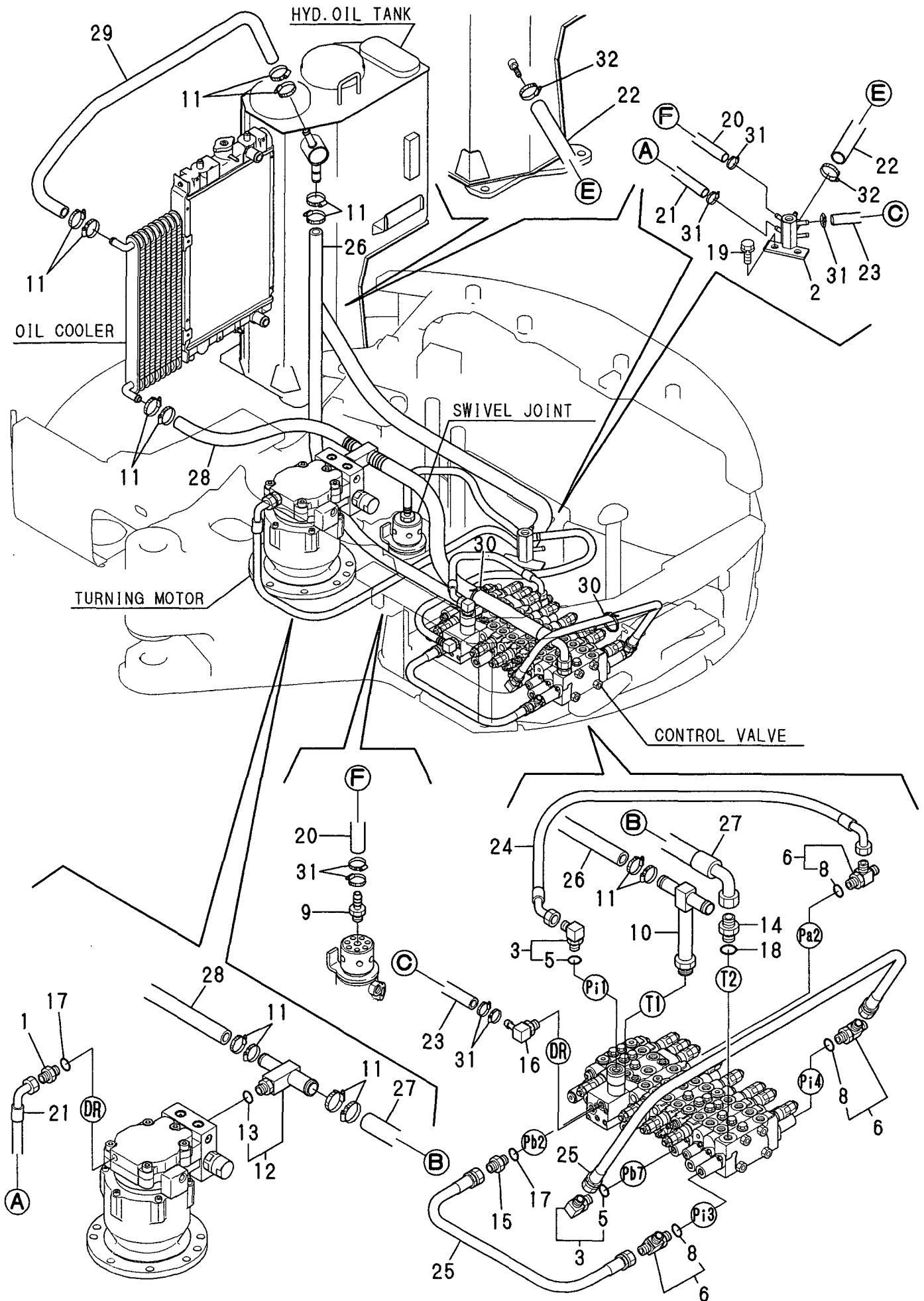
Fig. 47 HYD. OIL PIPING (RETURN)
