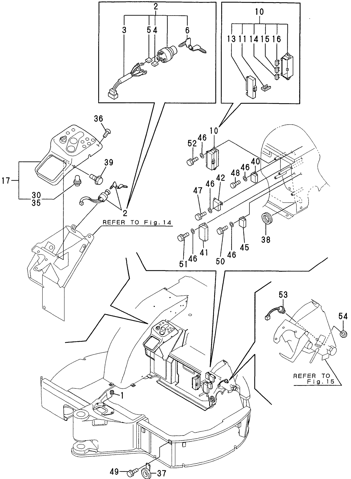
Fig. 10 ELECTRIC PART (EQUIPMENT)
