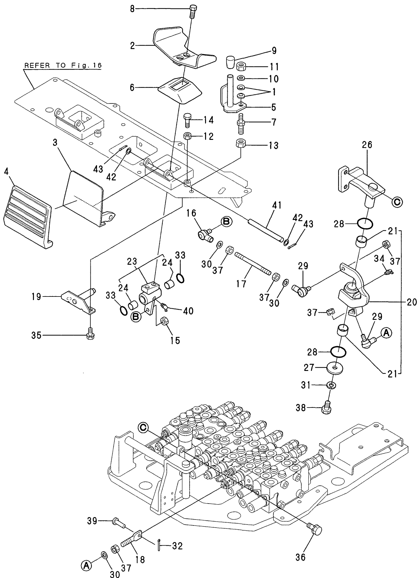
Fig. 20 CONTROL EQUIPMENT (P. T. O. PEDAL)
