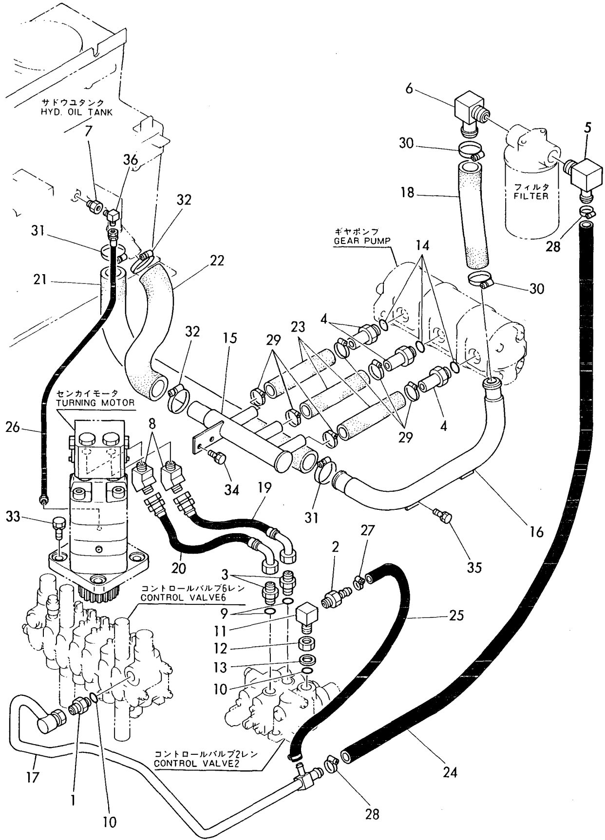
https://truckmanualshub.com Fig. 36 ユアツハイカン(タンク・バルブ・モータ)(キューガタ) HYD. OIL PIPING (TANK-VALVE-MOTOR) (PREVIOUS) (YB121U: M/ #00698マデ) (YB151U: M/ #00608マデ) (YB121U: TO M/ #00698) (YB151U: TO M/ #00608)
