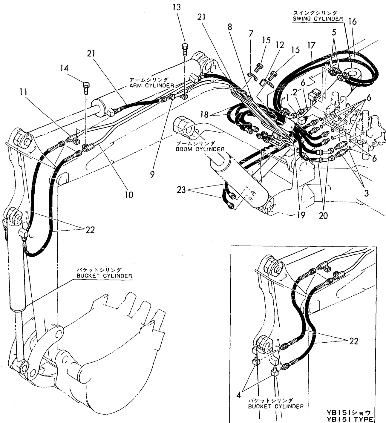
Fig. 39 ユアツハイカン(サギョウキブ)(キョウガタ) HYD. OIL PIPING (WORK EQUIPMNT) (PREVIOUS) (YB121U: M/ #00698マデ) (YB151U: M/ #00608マデ) (YB121U: TO M/ #00698) (YB151U: TO M/ #00608)
