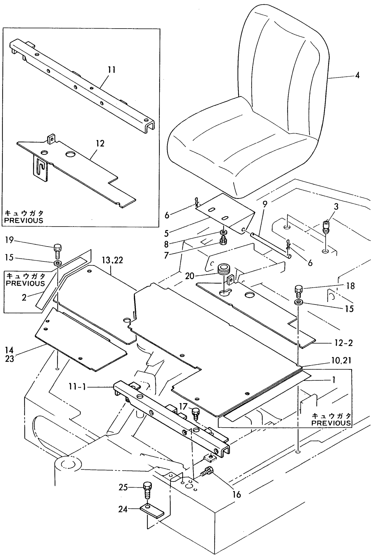
Fig. 28 シート&ステップ(シンガタ) SEAT & STEP (NEW TYPE) (YB121U,YB151U: M/ #10501カラ) (YB121U,YB151U: FROM M/ #10501)
