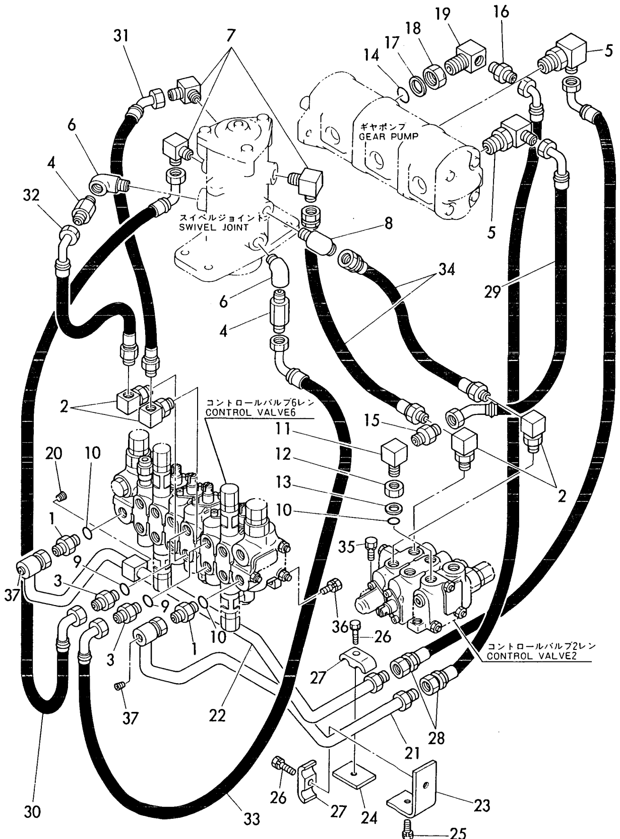
Fig. 34 ユアツハイカン(バルブスィベル)(キュウガタ) HYD. OIL PIPING (VALVE-SWIVEL) (PREVIOUS) (YB121U: M/ #00698マデ) (YB151U: M/ #00608マデ) (YB121U: TO M/ #00698) (YB151U: TO M/ #00608)
