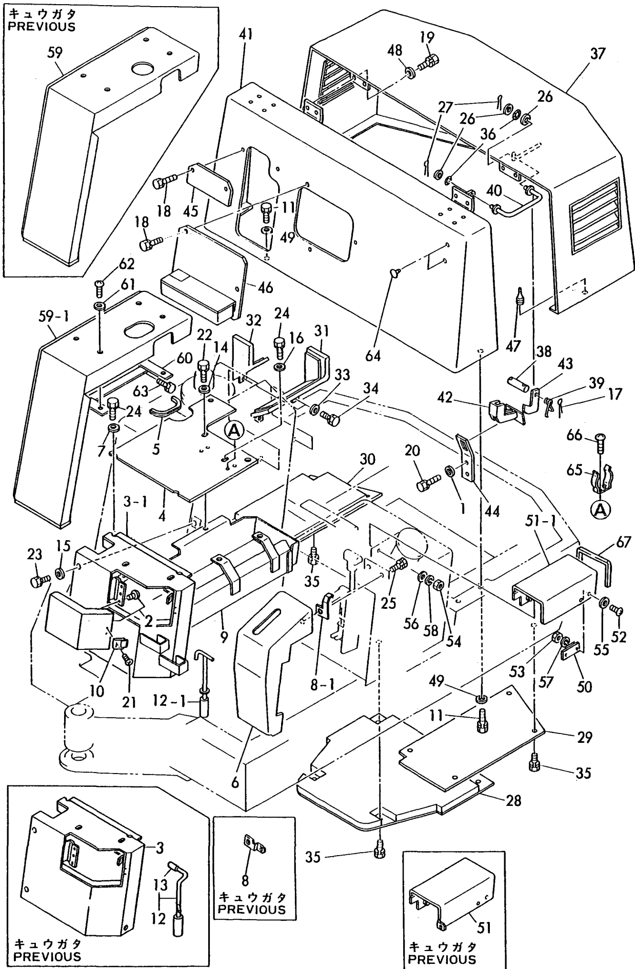
Fig. 26 ボンネット(シンガタ) BONNET (NEW TYPE) (YB121U, YB151U: M/ #10501カラ) (YB121U, YB151U: FROM M/ #10501)
