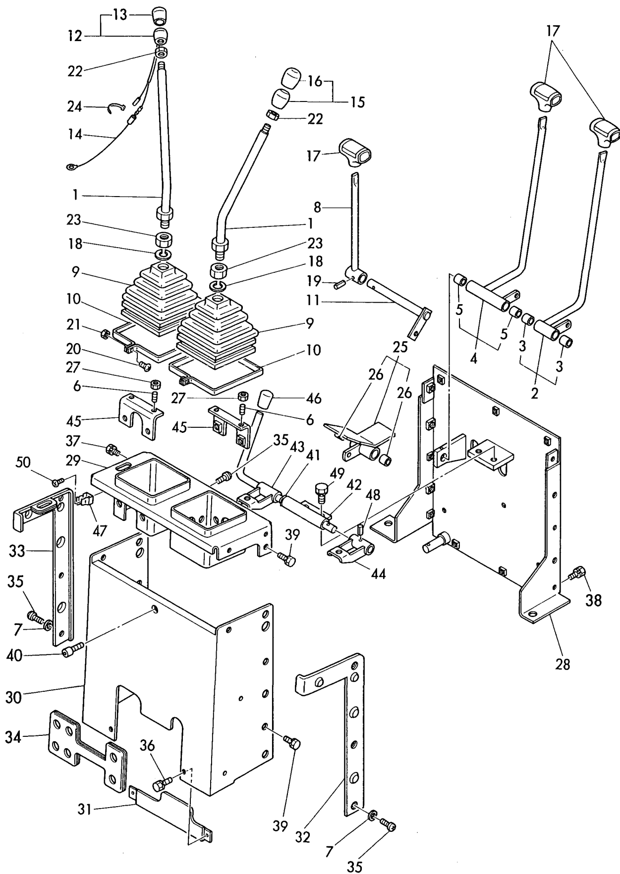
Fig. 18 ソウジュウソウチ(レバー)(キョウガタ) CONTROL EQUIPMENT (LEVER) (PREVIOUS) (YB121U: M/ #00698マデ) (YB151U: M/ #00608マデ) (YB121U: TO M/ #00698) (YB151U: TO M/ #00608)
