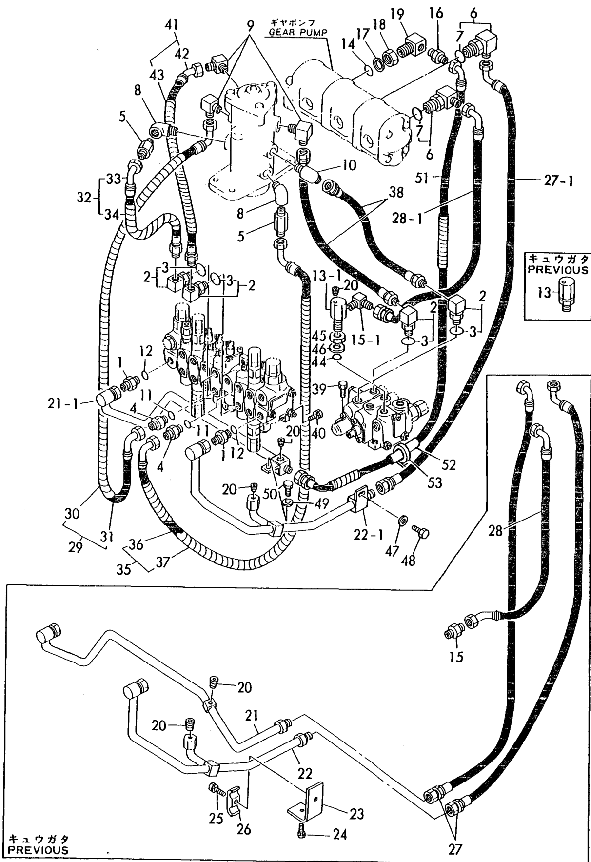
Fig. 35 ユアツハイカン(バルブースイベル)(シンガタ) HYD. OIL PIPING (VALVE-SWIVEL) (NEW TYPE) (YB121U, YB151U: M/ #10501カラ) (YB121U, YB151U: FROM M/ #10501)
