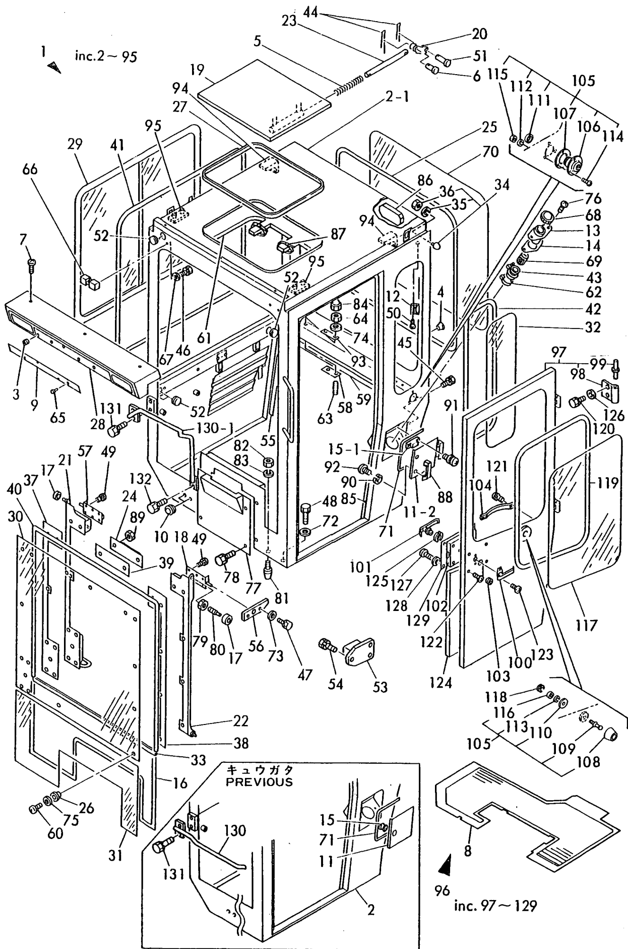
Fig. 31 キャビン(シンガタ) CABIN (NEW TYPE) (YB121U,YB151U: M/ # 10501カラ) (YB121U,YB151U: FROM M/ # 10501)
