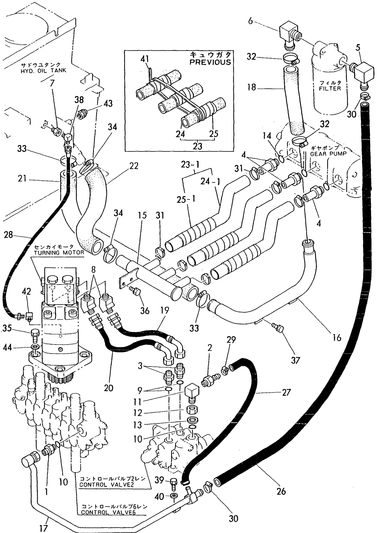
Fig. 37 ユアツハイカン(タンク-バルブ-モータ)(シンガタ) HYD. OIL PIPING (TANK-VALVE-MOTOR)(NEW TYPE) (YB121U, YB151U: M/ #10501カラ) (YB121U, YB151U: FROM M/ #10501)
