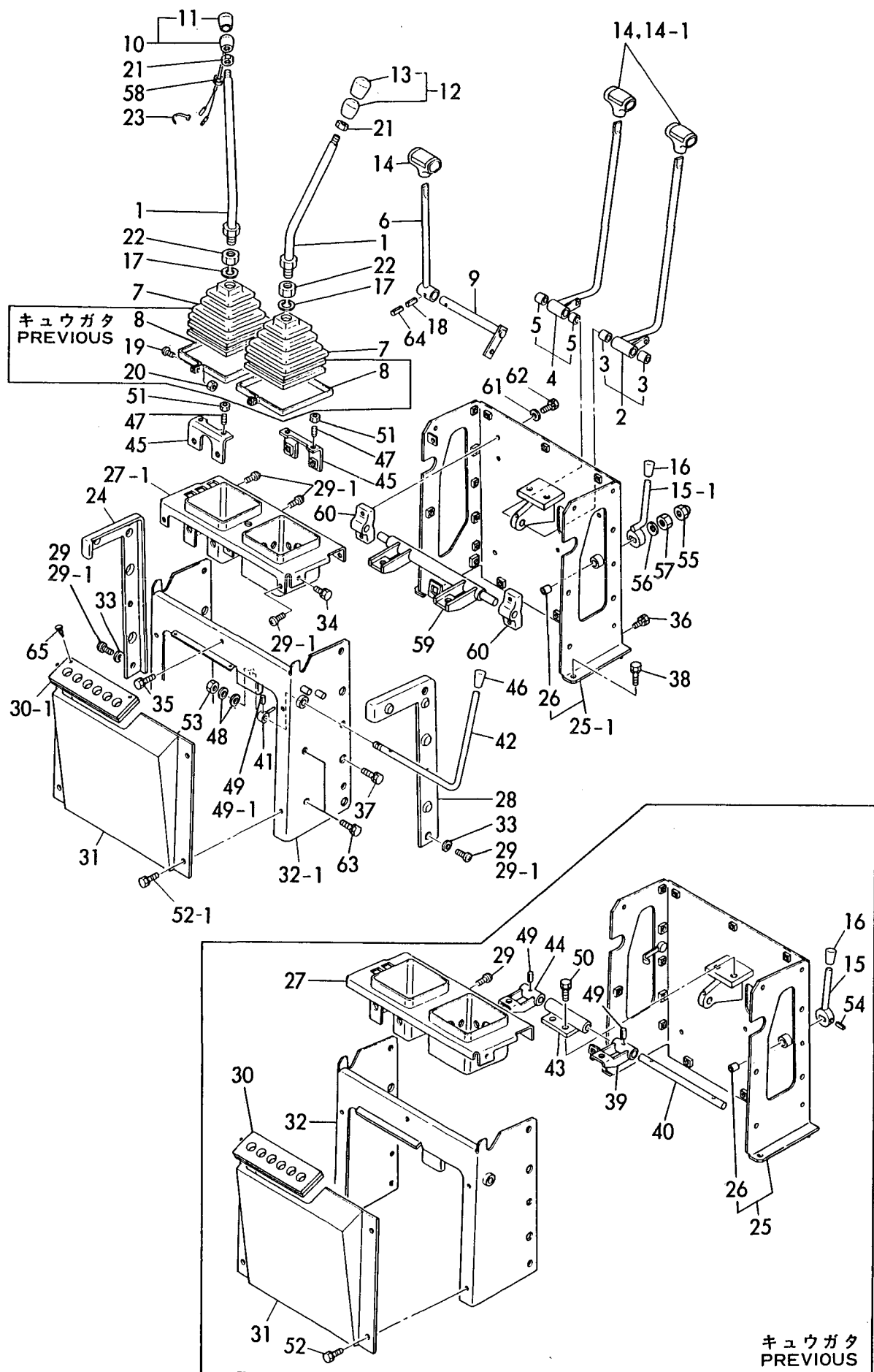
Fig. 19 ソウジュウソウチ(レバー)(シンガタ) CONTROL EQUIPMENT (LEVER) (NEW TYPE) (YB121U, YB151U: M/ #10501カラ) (YB121U, YB151U: FROM M/ #10501)
