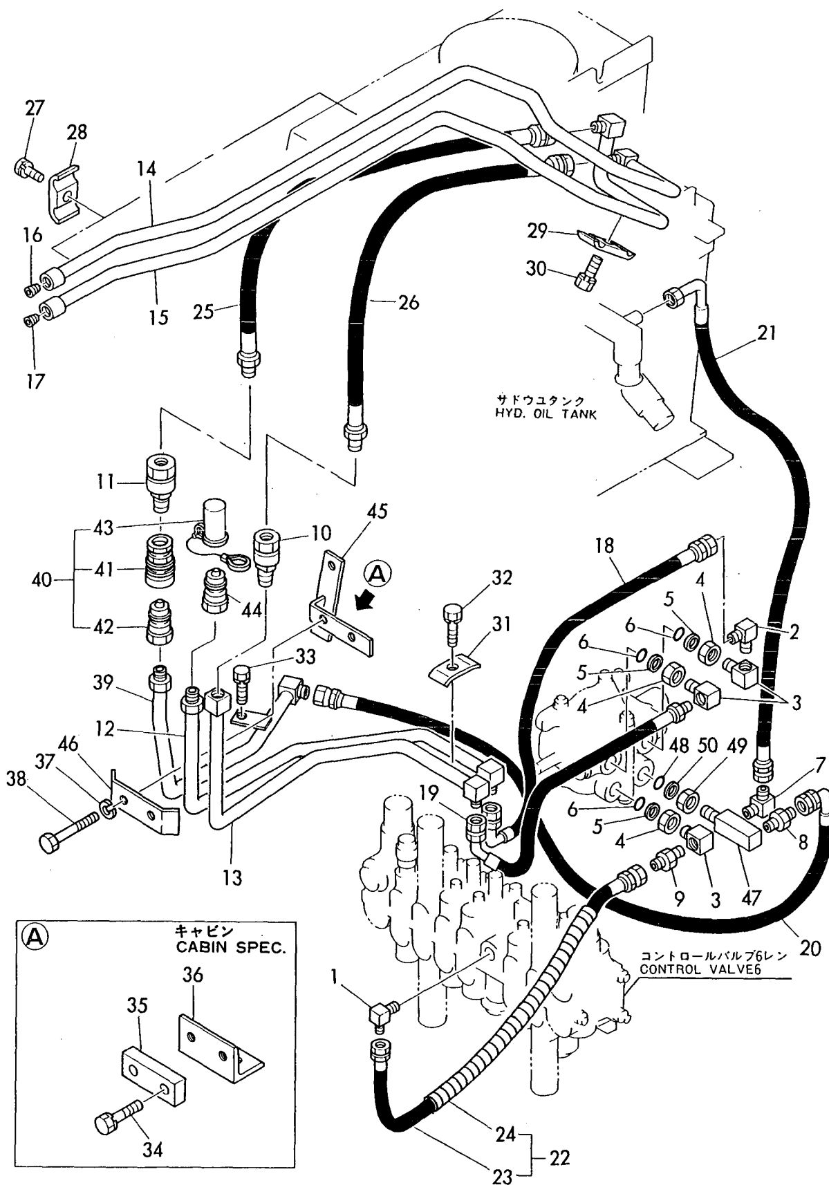
Fig. 75 サードバルブハイカン(オプション)(シンガタ) 3RD VALVE PIPING (OPTIONAL) (NEW TYPE) (YB121U, YB151U: M/ # 10501カラ) (YB121U, YB151U: FROM M/ # 10501)
