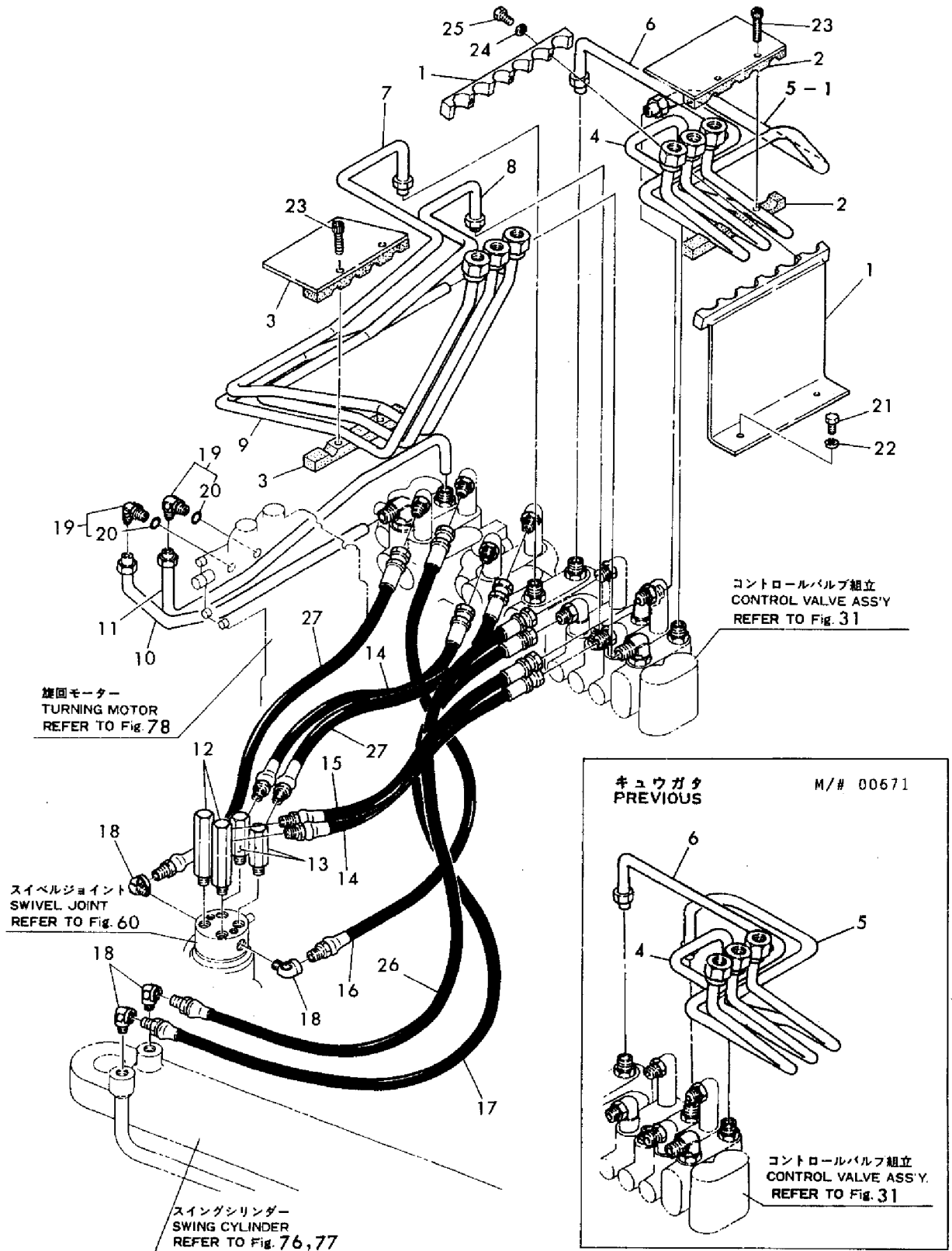
Fig. 35 上部油圧配管 (2), YB201U (Z) ヨウ UPPER HYDRAULIC OIL PIPING (2), FOR MODEL YB201U (Z)
