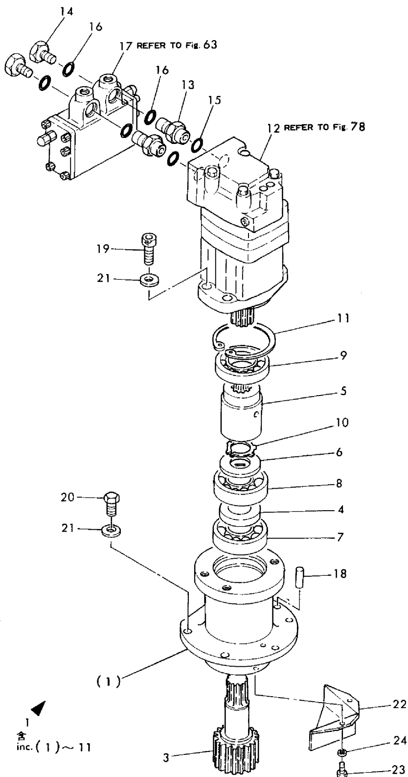
Fig. 8 旋回駆動装置 TURNING DRIVING GEAR
