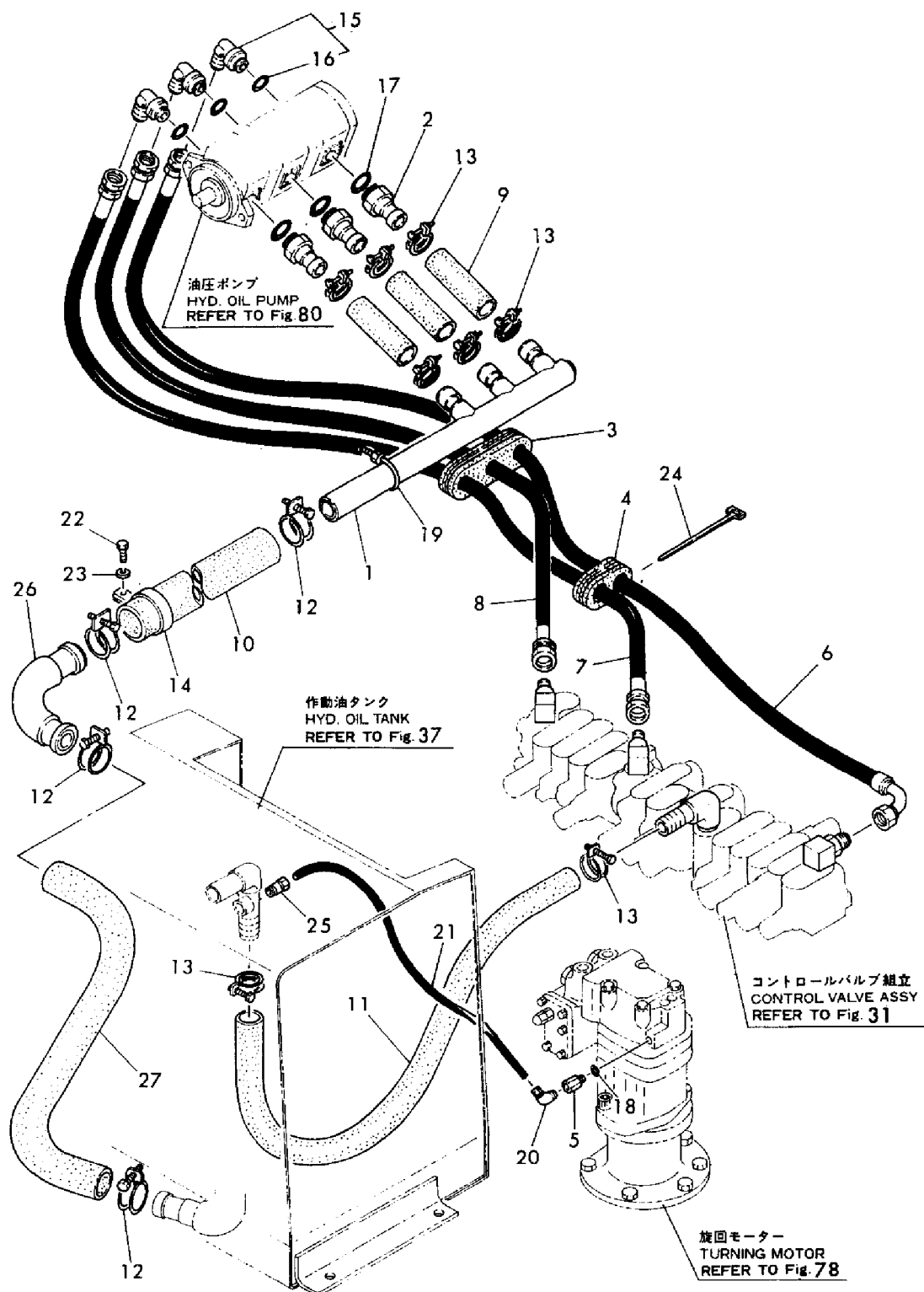
Fig. 33 上部油圧配管 (1), YB201U (Z) ヨウ UPPER HYDRAULIC OIL PIPING (1), FOR MODEL YB201U (Z)
