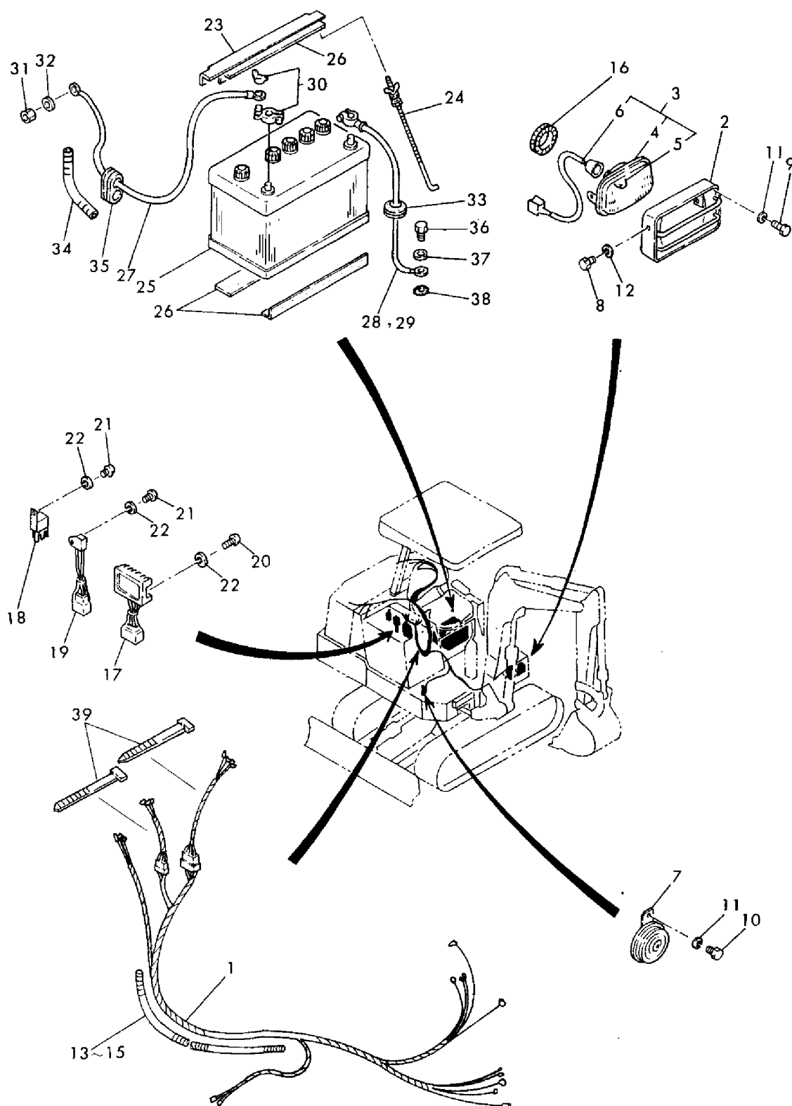
Fig. 26 電装品, YB201 (Z) ヨウ ELECTRIC EQUIPMENT RELATED, FOR MODEL YB201 (Z)
