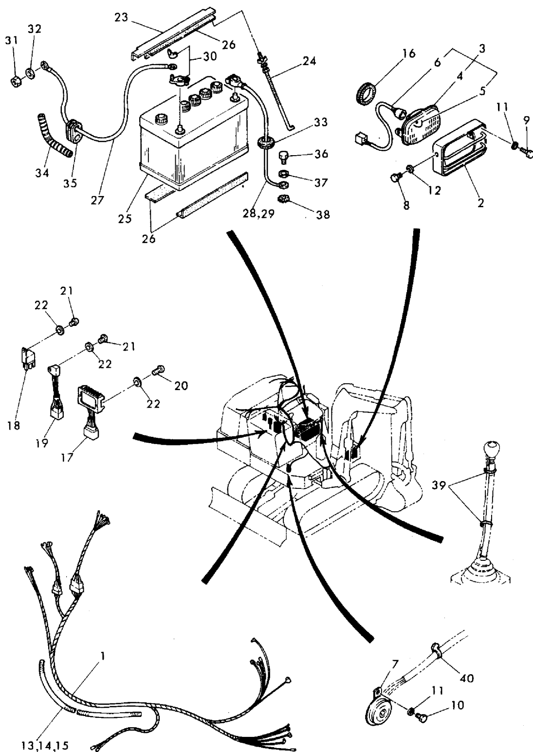
Fig. 27 電装品, YB201U (Z) ヨウ ELECTRIC EQUIPMENT RELATED, FOR MODEL YB201U (Z)
