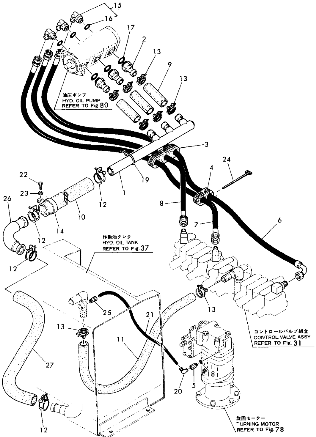
Fig. 33 上部油圧配管 (1), YB201U (Z) ヨウ UPPER HYDRAULIC OIL PIPING (1), FOR MODEL YB201U (Z)
