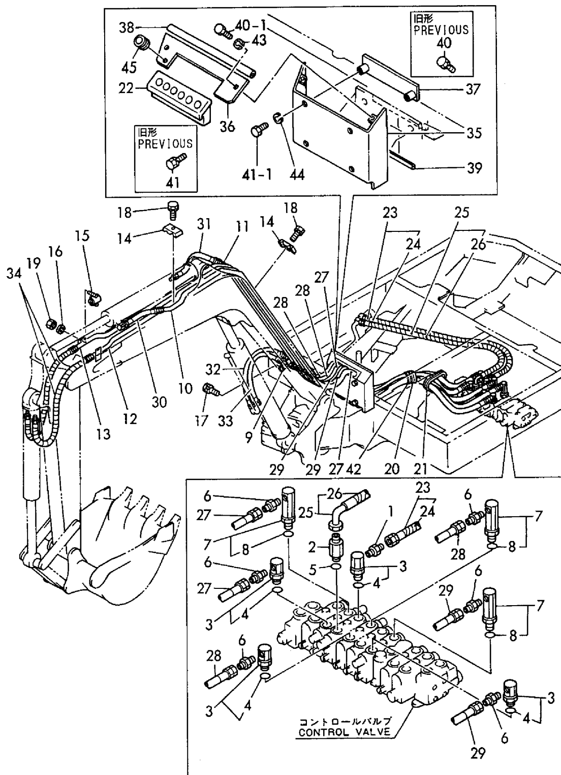
Fig. 52 油圧配管 (作業部) HYD. OIL PIPING (EQUIPMENT)
