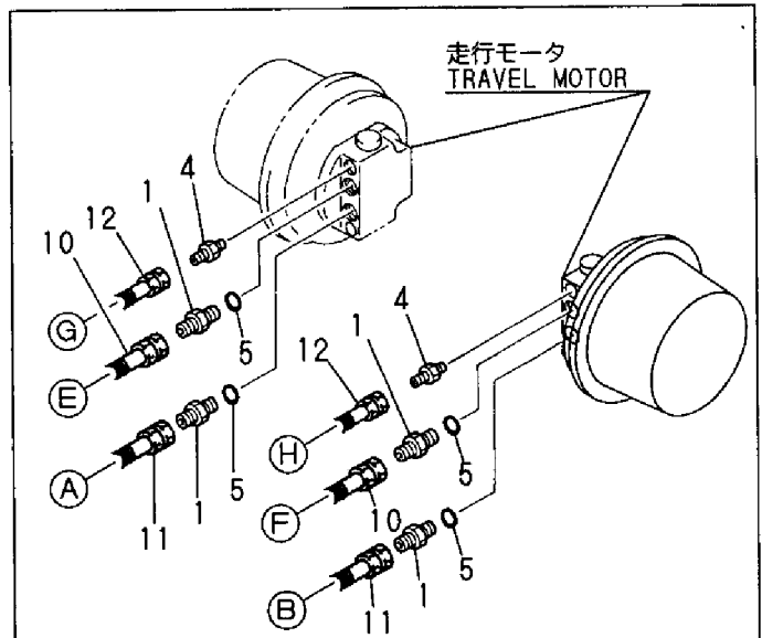
Fig. 51 油圧配管 (走行) HYD. OIL PIPING (TRAVEL)
