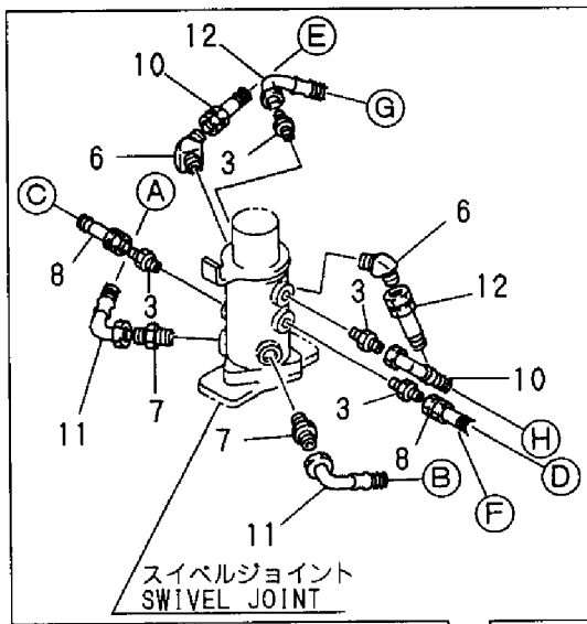
Fig. 51 油圧配管 (走行) HYD. OIL PIPING (TRAVEL)
