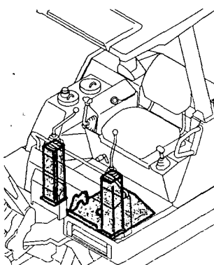
Fig.20 操縦装置 (レバー) CONTROL EQUIPMENT (LEVER)
