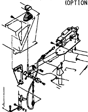
Fig.63 3RDバルブ配管 (オプション) 3RD VALVE PIPING (OPTIONAL)
