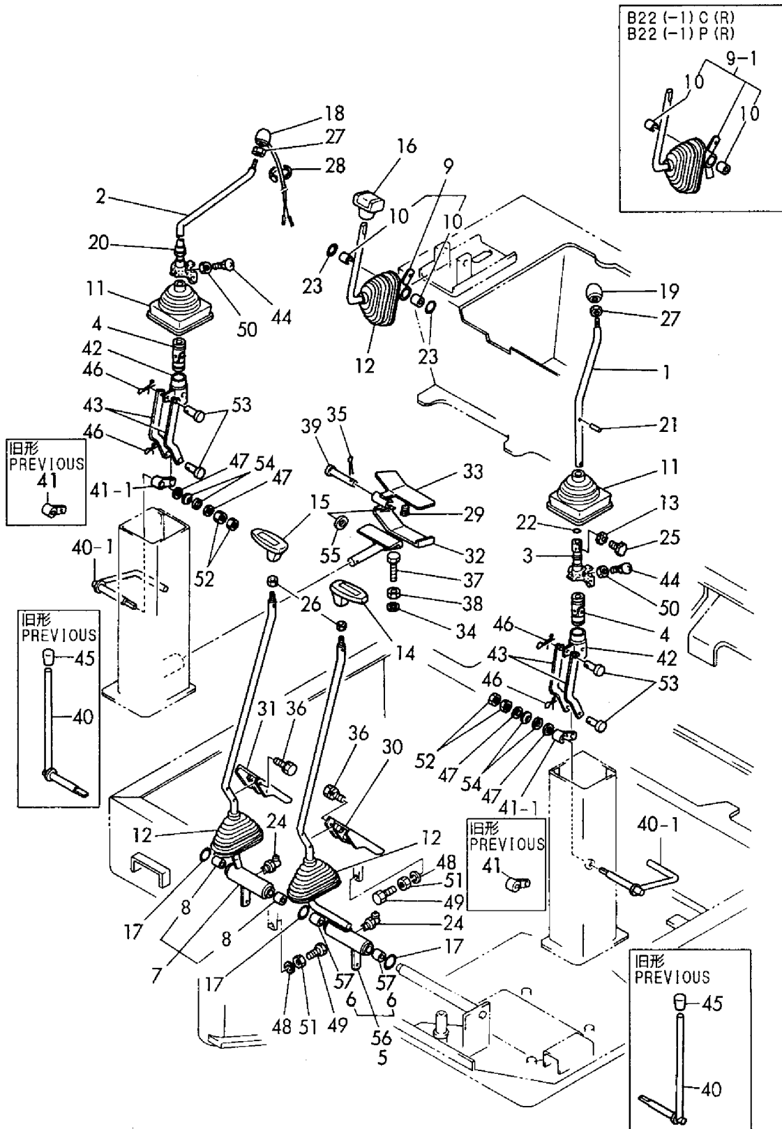
Fig. 20 操縦装置 (レバー) CONTROL EQUIPMENT (LEVER)
