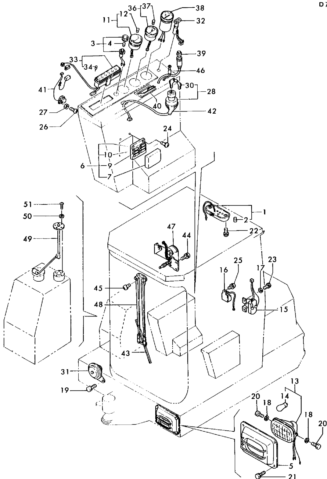
Fig. 15 デンキキキ (キャビン) (キュウガタ) ELECTRIC PARTS (CABIN) (PREVIO TYPE)
